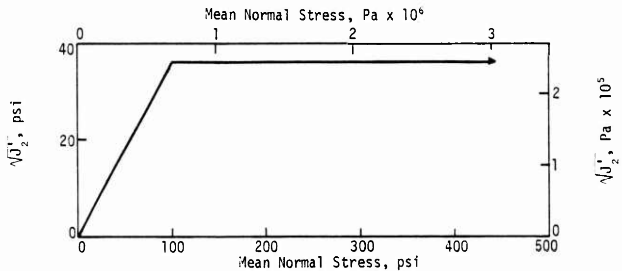
Figure 10. Material Properties of Dry Clay
