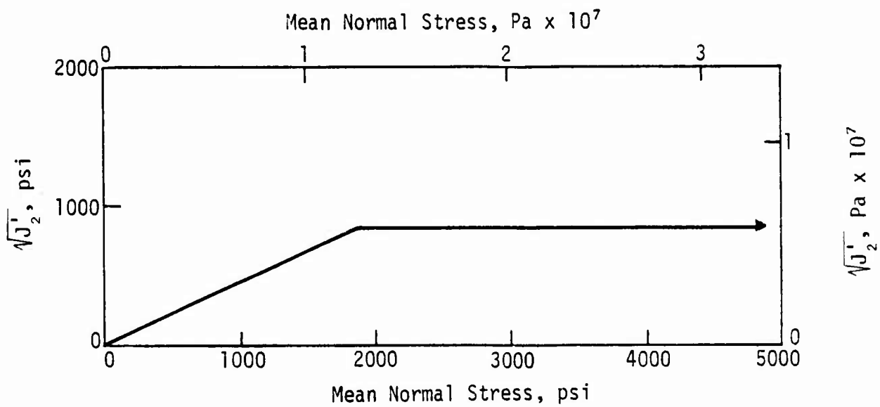
Figure 13. Material Properties of Limestone/Shale Composite
