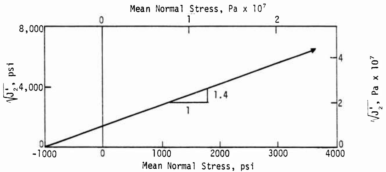
Figure 17. Material Properties of Deep Limestone
