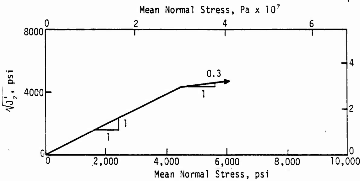
Figure 15. Material Properties of Coal
