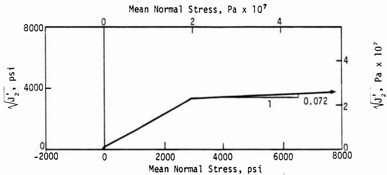
Figure 14. Material Properties of Shale
