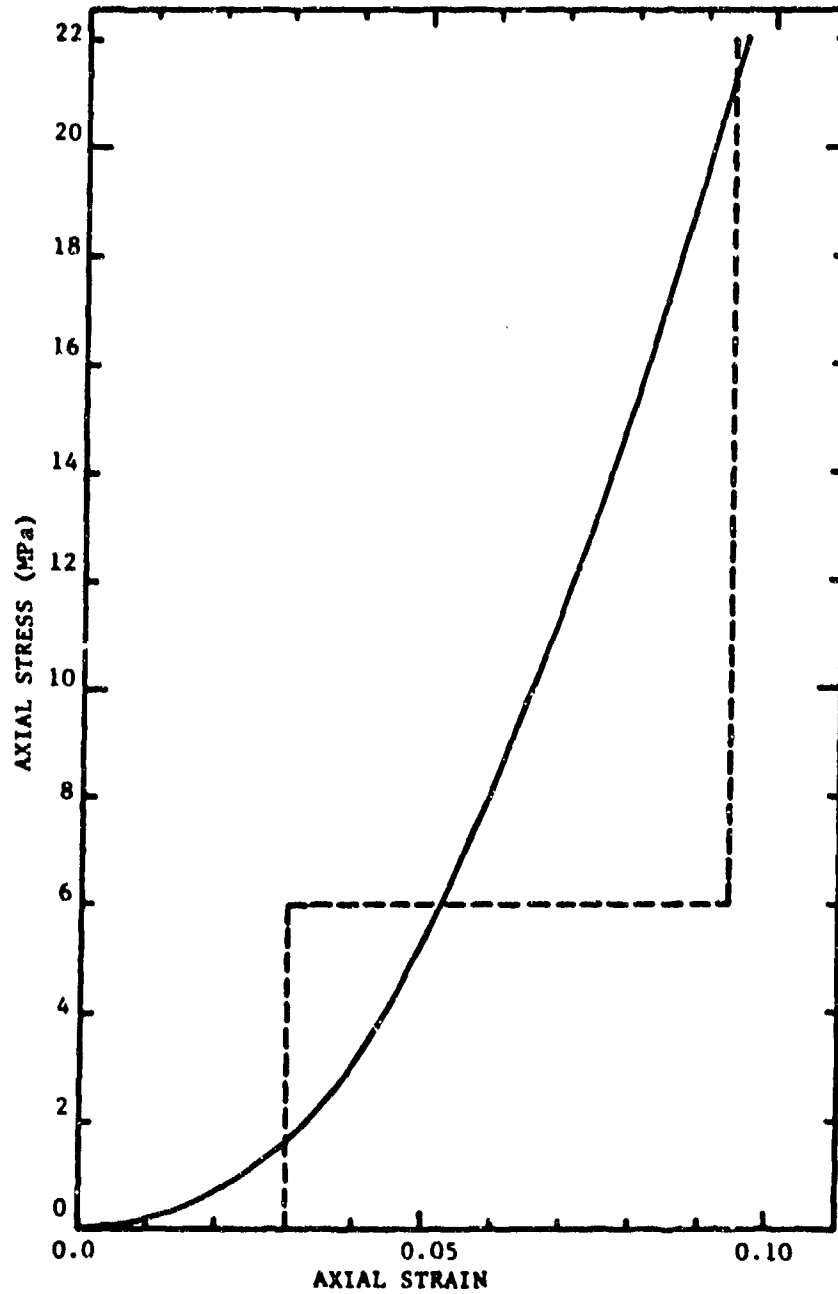
Figure 56. Ideal Locking Approximation to Uniaxial Strain Curve for Loose Egin Sand (Initial Density 1540 \text{ kg/m}^3 )
