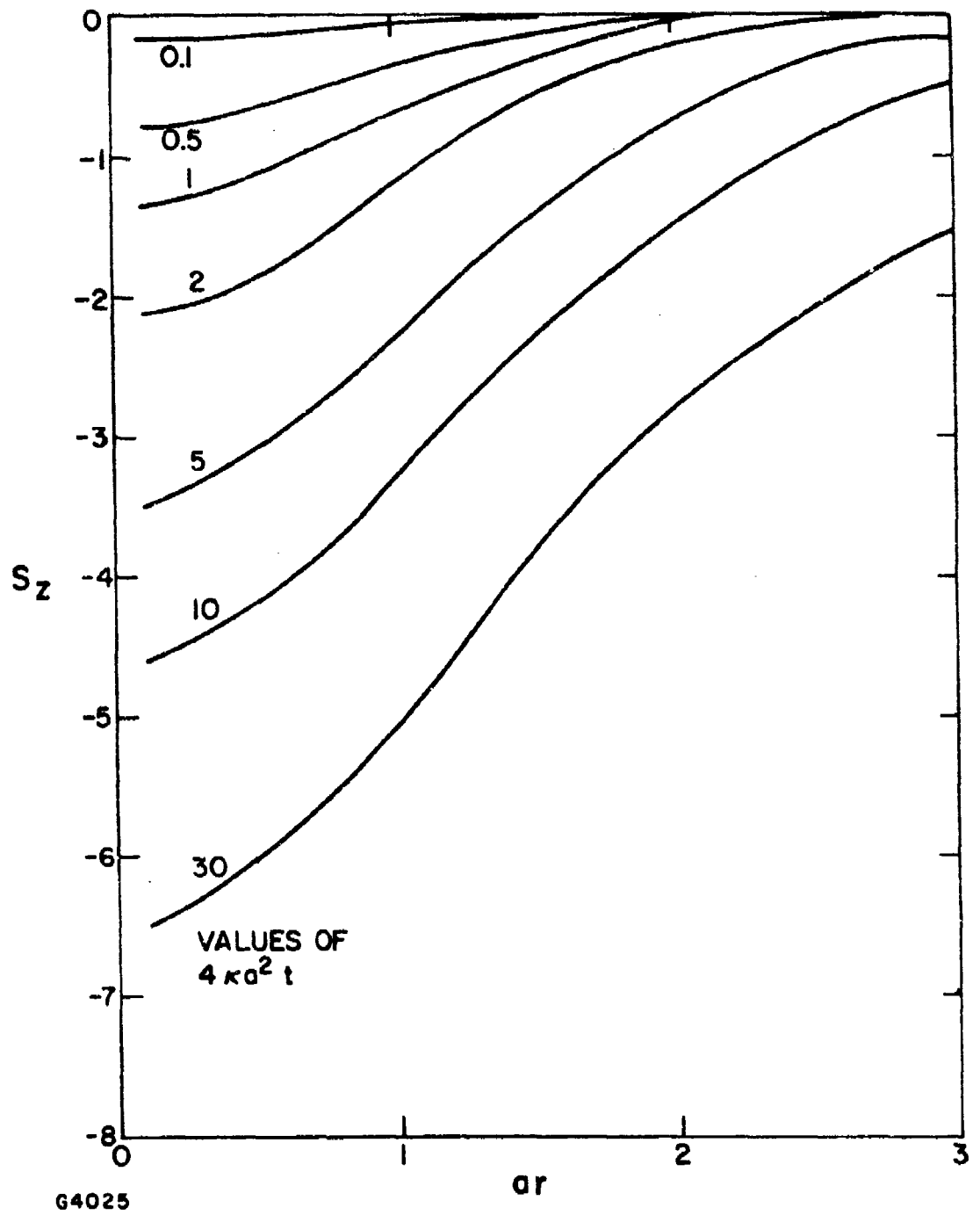
Figure 4 Non-Dimensional Axial Stress
