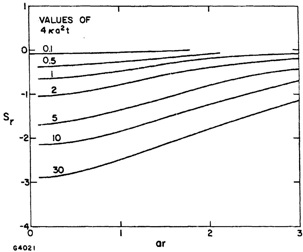
Figure 2 Non-Dimensional Radial Stress
