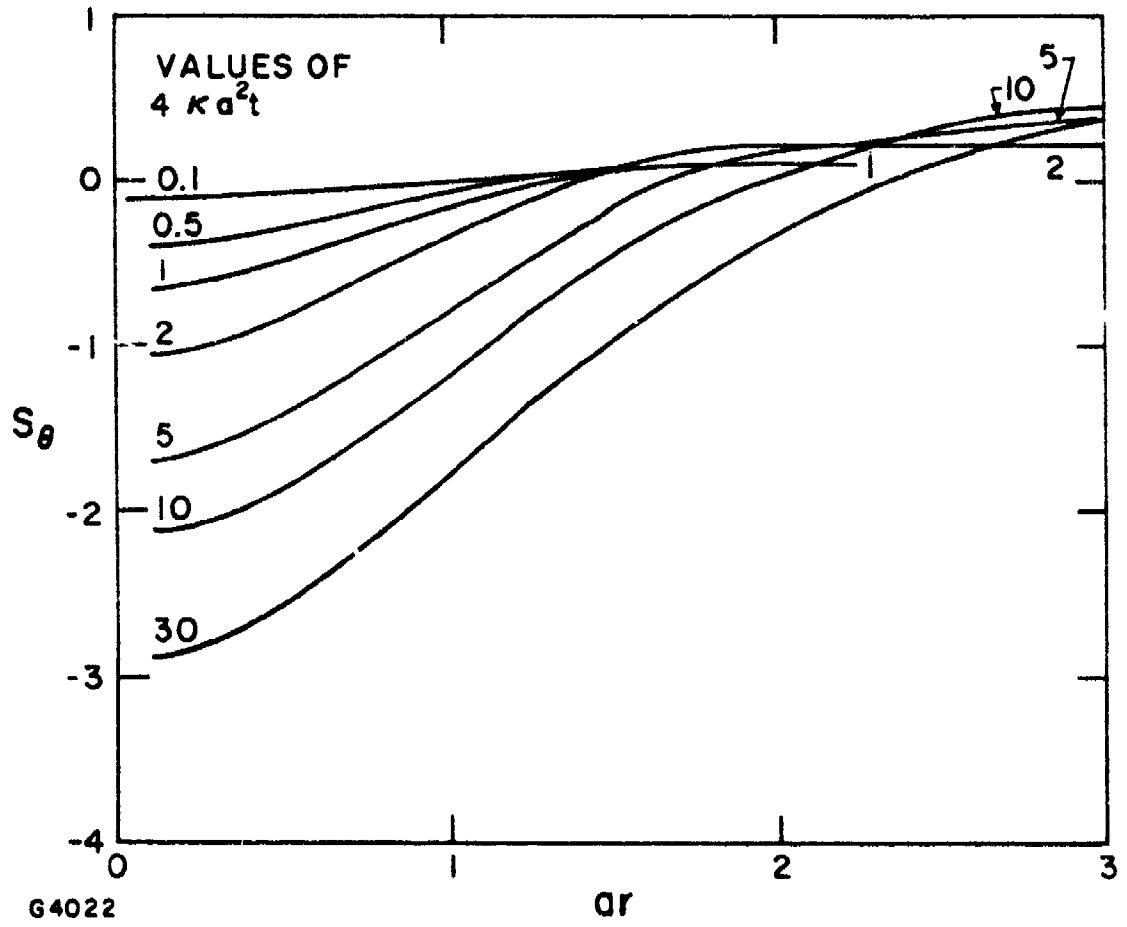
Figure 3 Non-Dimensional Tangential Stress
