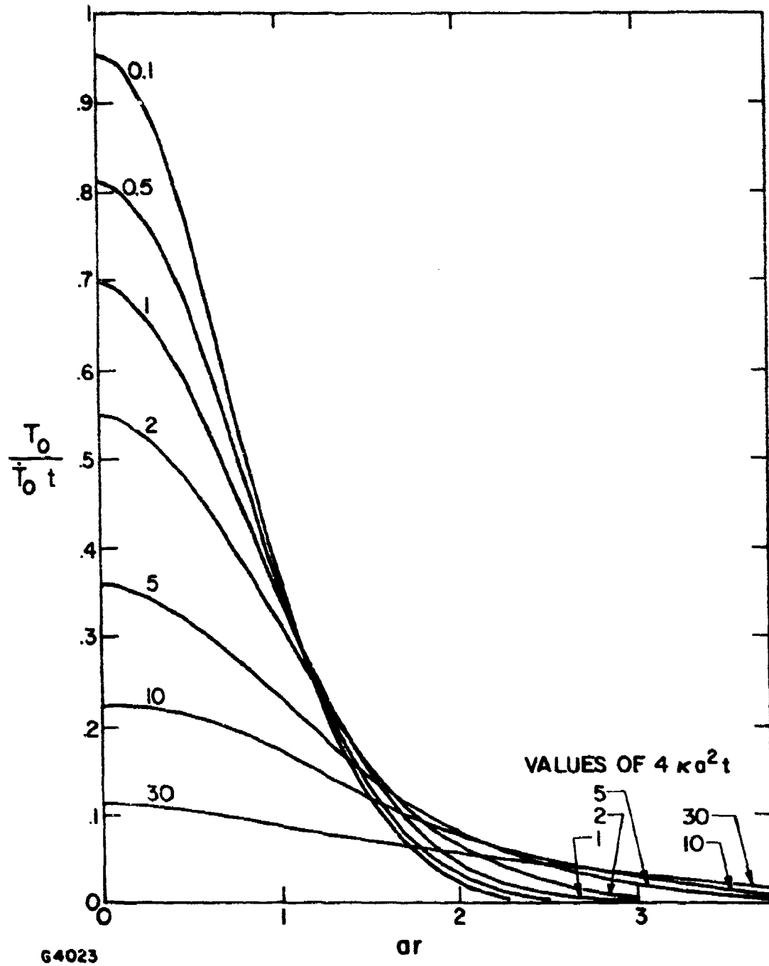
Figure 1 Temperature Profiles
