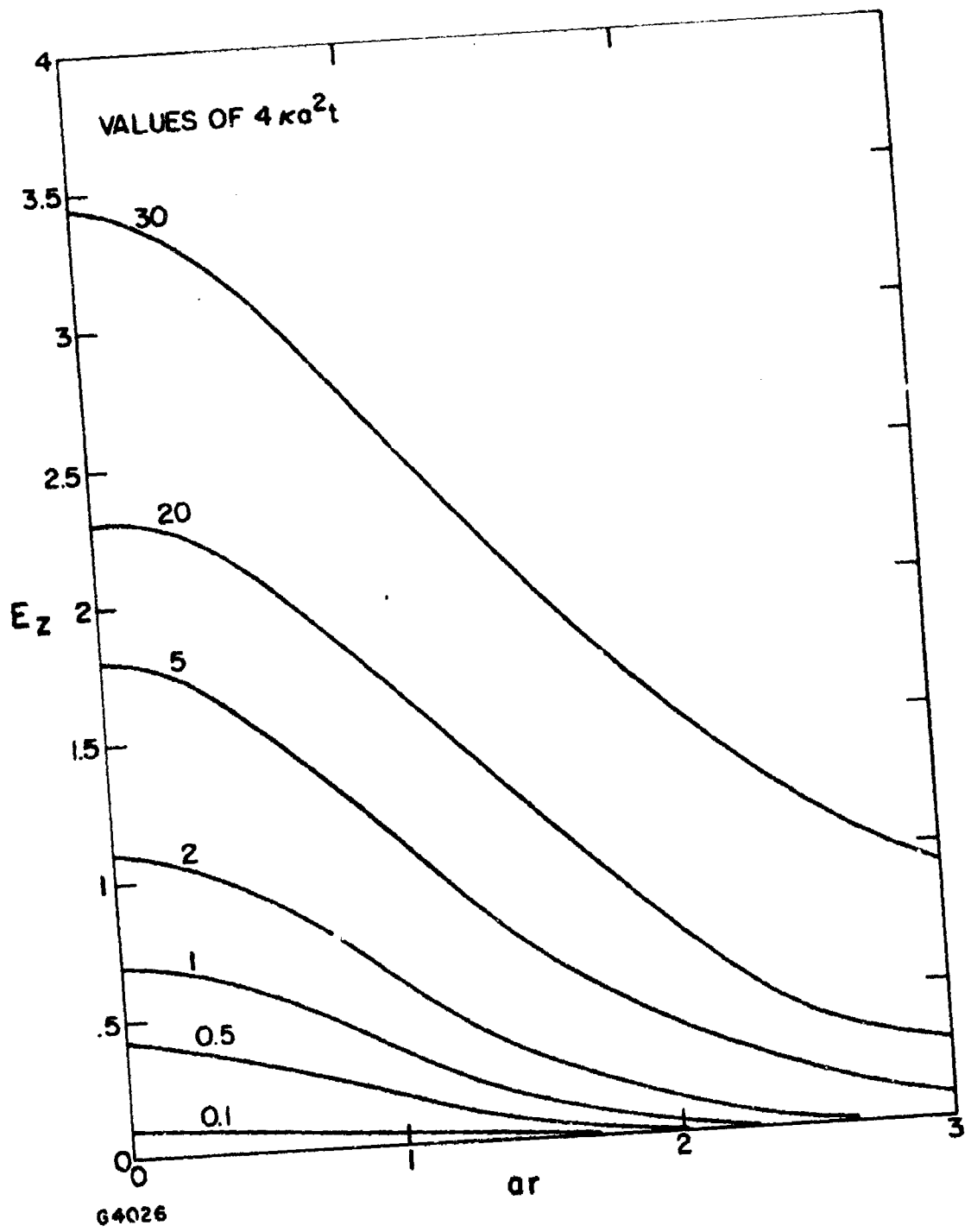
Figure 5 Non-Dimensional Strain
