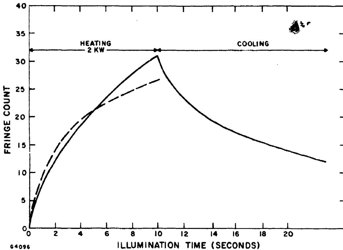
64096 Figure 7 Comparison of Experimental and Calculated Optical Path Difference
