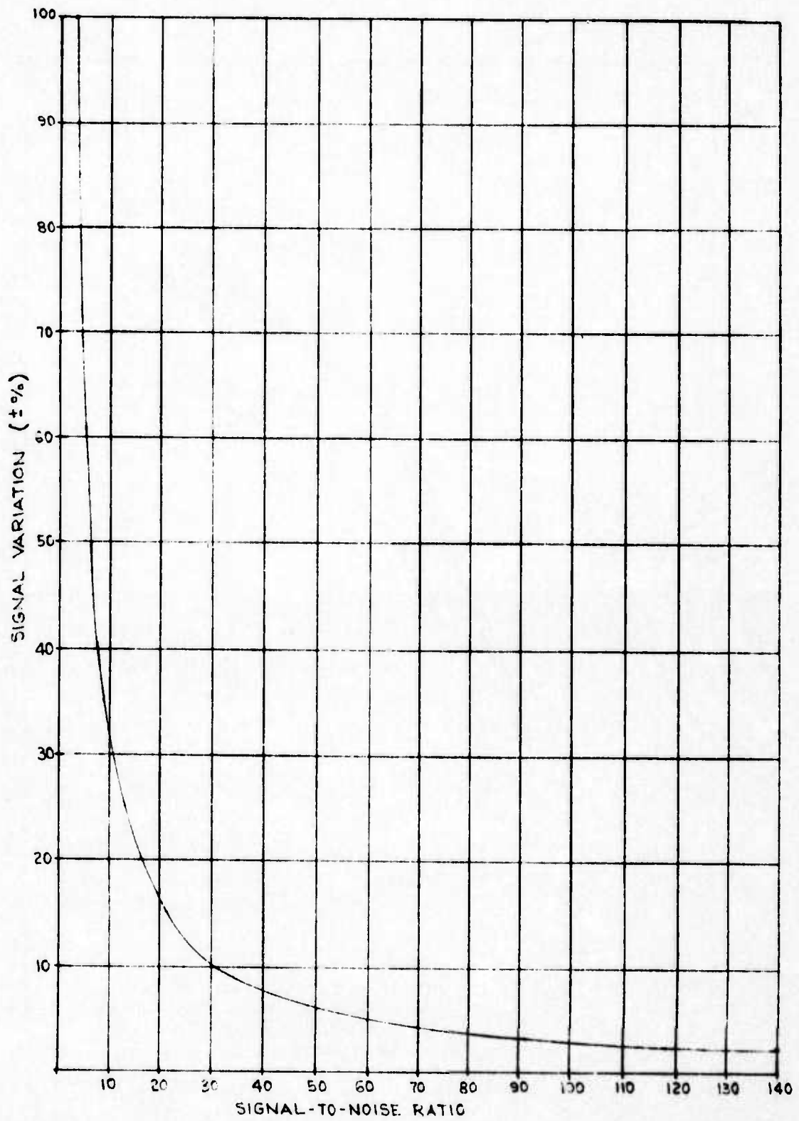
Figure 17 Percent Signal Variation Versus Signal-to-Noise Ratio
