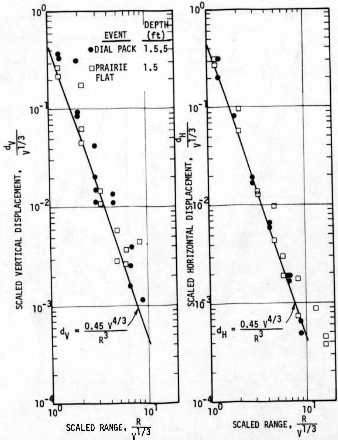
Figure 41. Crater Volume Scaled Peak Displacement Correlation for Top 0.1 v^{1/3} for SES Events (Reference 67)
