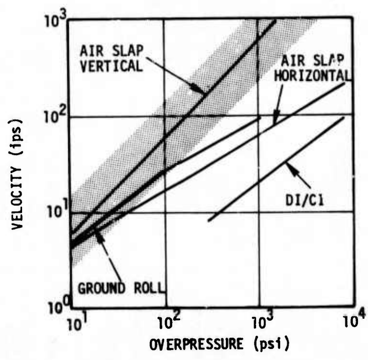
Figure 55. Dry Soil 1-MT Surface Burst Near-Surface Motion Peak Values
