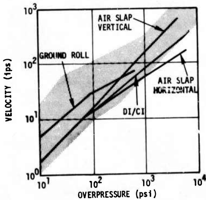
Figure 56. Wet Soil 1-MT Surface Burst Near-Surface Motion Peak Values
