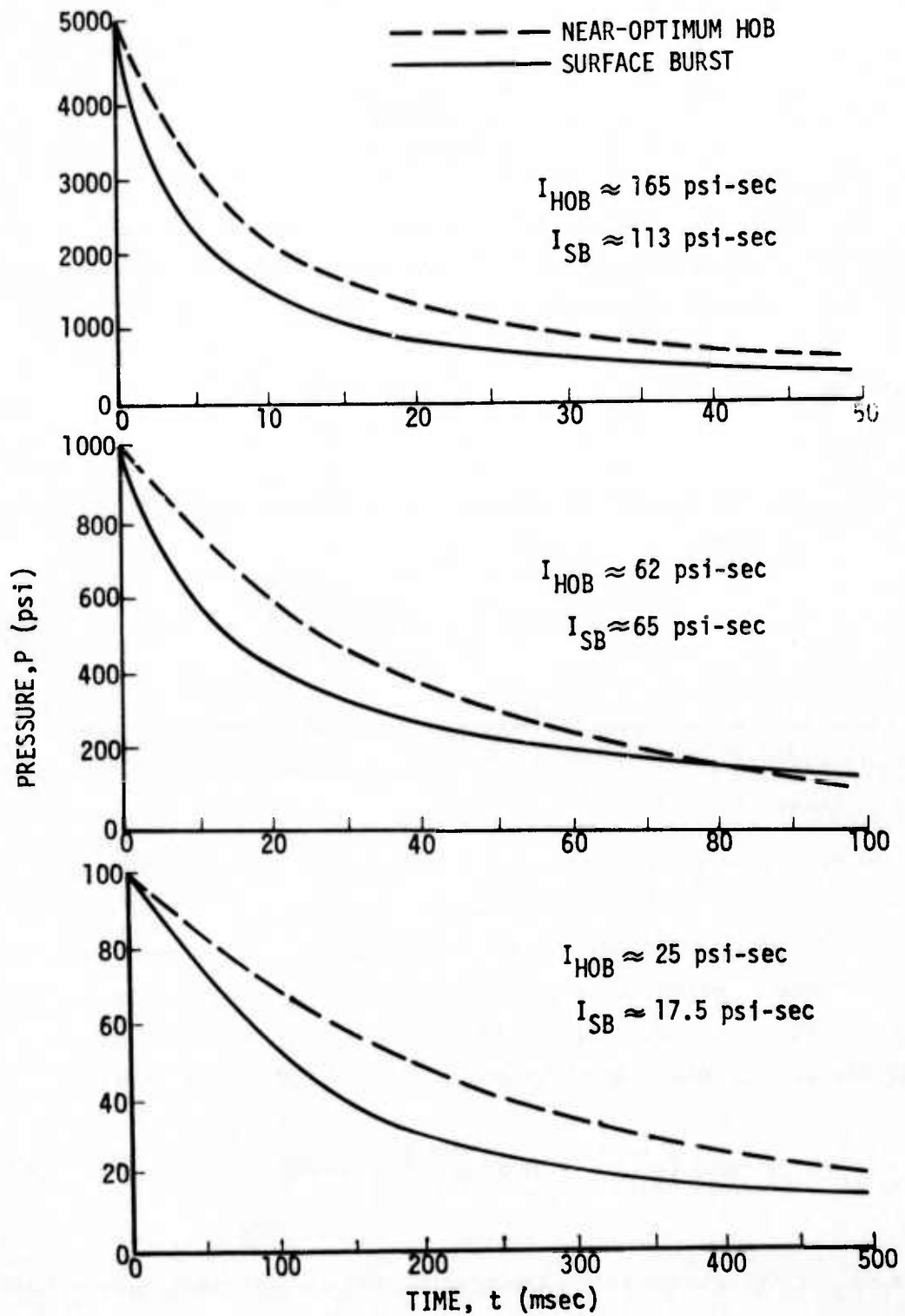
Figure 76. Comparison of Surface Burst and HOB Overpressure Waveforms
