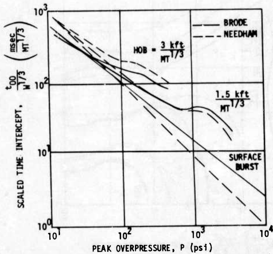
Figure 3. Overpressure Initial Decay Time Intercept
