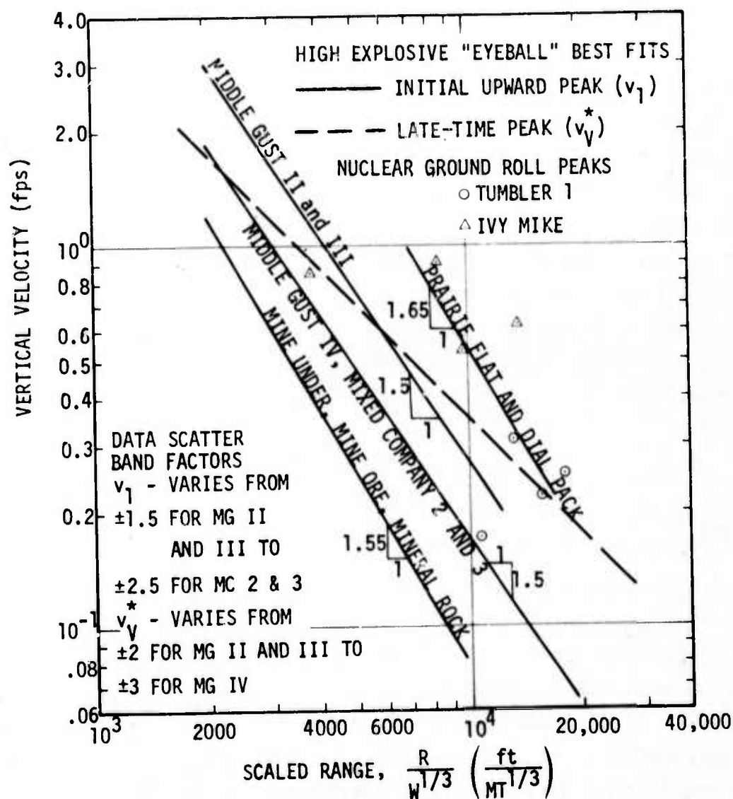
Figure 52. High Explosive Outrunning Vertical Velocity Peak Attenuation and Nuclear Data Comparison (Reference 71)
