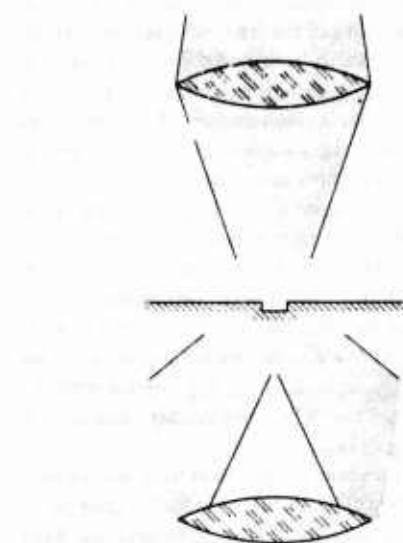
Fig. 1. Modulation of the light by a pit in the surface of a 'VLP' record. For clarity the system is drawn as if the record were transparent, with the beam incident from above and a second lens placed underneath the record to receive the light. The pit is also shown many times enlarged with respect to the rest of the figure. If the record surface is flat, all of the incident light is received by the lower lens. If there is a pit in the surface there will be diffraction, and some of the light will be deflected; when the pit is correctly dimensioned much of the incident light will be deflected away from the aperture of the lower lens. In practice the record surface is reflecting, and only one lens is required for concentrating the light on to the record and receiving the reflected light.
