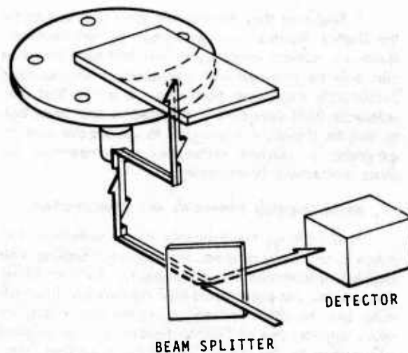
FIGURE 7. Read Back Light Path
