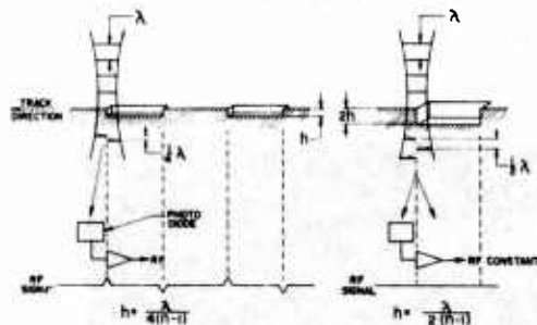
Fig. 4. RF signal derived from pitted tracks.
