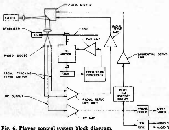
Fig. 6. Player control system block diagram.
