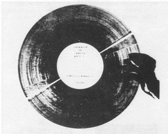
Figure 3. Appearance of the video film disc. This particular disc has a playing time in excess of 20 minutes at the full NTSC video framing rate.
