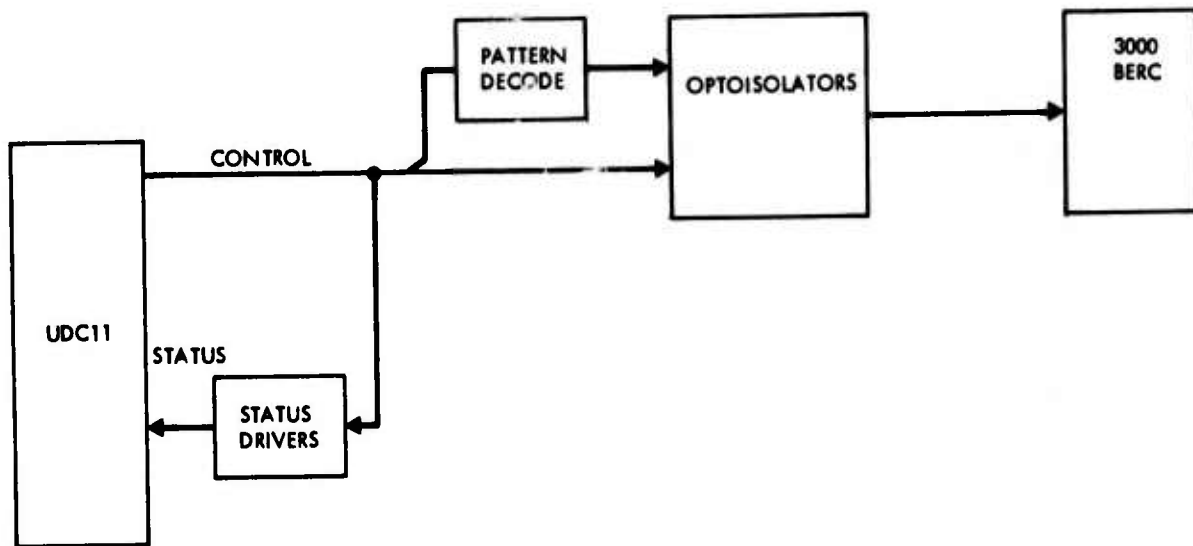
Figure 10. 3000 Data Generator Control, Block Diagram
