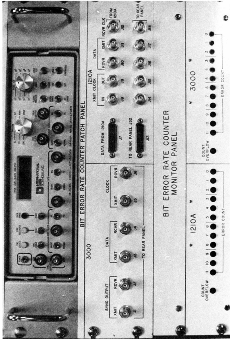
Figure 2. Patch Panel
