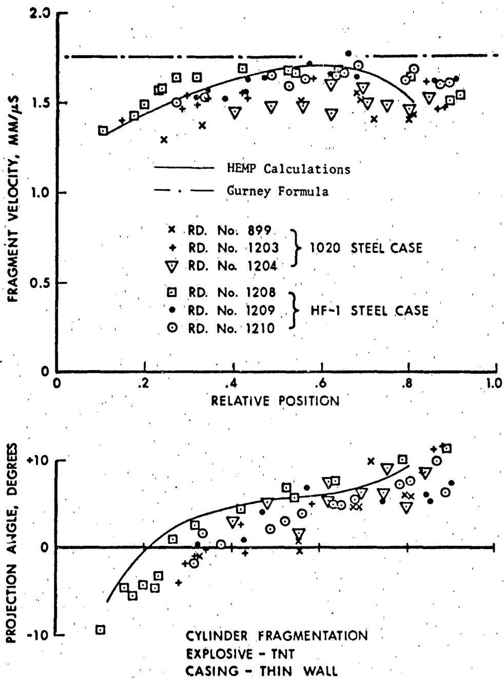
Figure 15. Comparison Between HEMP Calculations and Experimental Data of Fragment Speed and Projection Angle for Cylinders of L/D = 2 , TNT, C/M = .8
