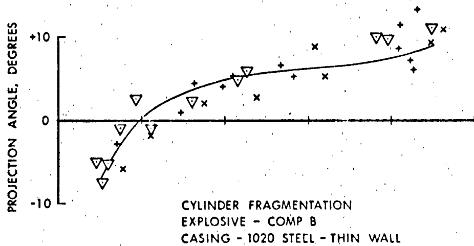
Figure 14. Comparison Between HEMP Calculations and Experimental Data of Fragment Speed and Projection Angle for Cylinders of L/D = 2 , Composition B, C/M = .8
