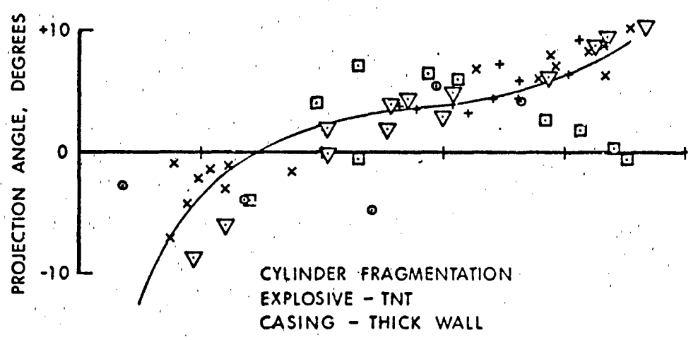
Figure 18. Comparison Between HEMP Calculations and Experimental Data of Fragment Speed and Projection Angle for Cylinders of L/D = 2 , TNT, C/M = .4
