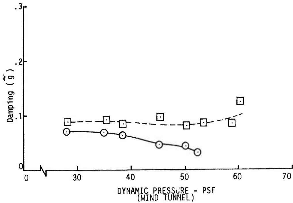
Figure 38. Flutter Mode Damping and Frequency Obtained From Co-Quad Plots of Inboard Wing Vertical Acceleration Due to Outboard Aileron
