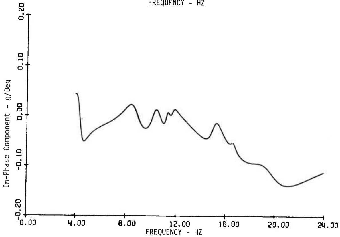
Figure 29. Analytical Outboard Wing Vertical Acceleration Due to Aileron Command Co-Quad Plot - FMCS On
