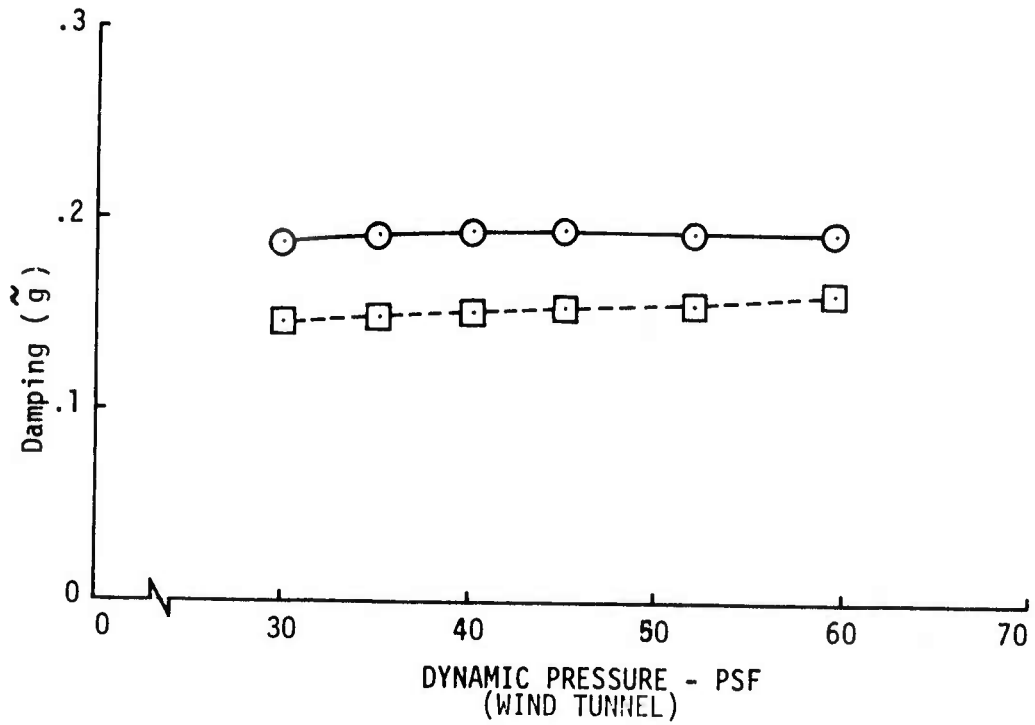
Figure 35. First Elastic Mode Damping and Frequency - Theoretical Characteristic Equation Roots
