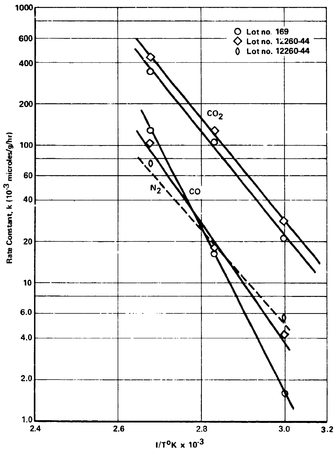
Figure 3-9 Arrhenius Plots of \text{CO}_2 , \text{CO} and \text{N}_2 Gassing Rates
