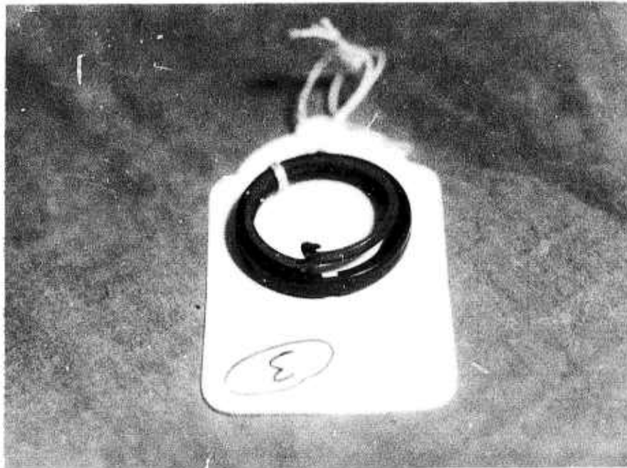
V720-75 T-Seal with Standard Revonoc 18158 Back-ups
