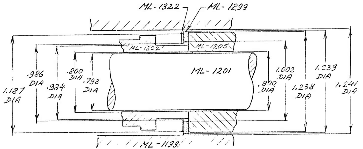
CYLINDER NO. 1.
