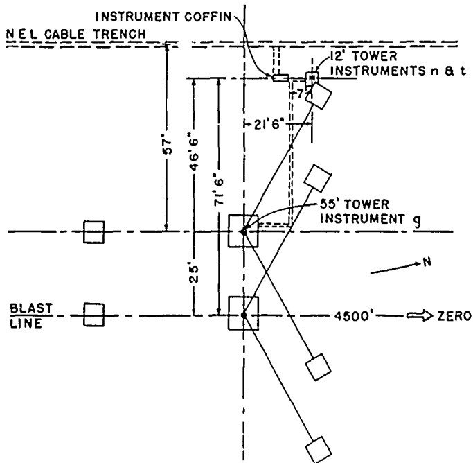
Fig. 2.9 7-206 Layout
