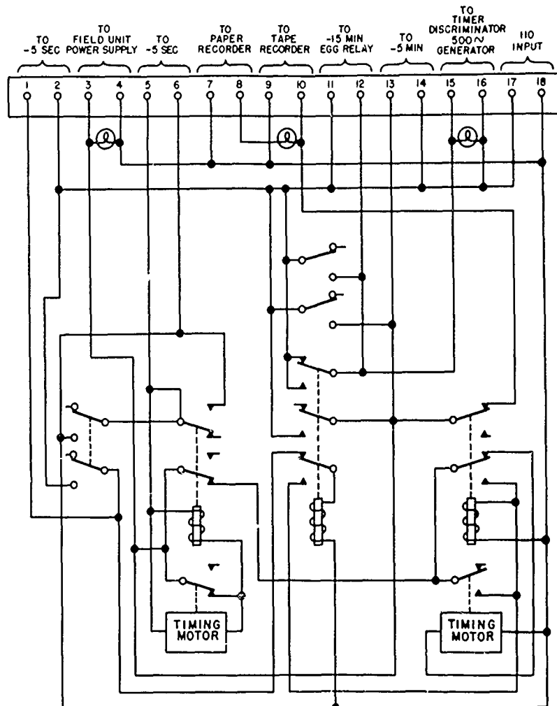
Fig. A.9 Relay Control Diagram Schematic
