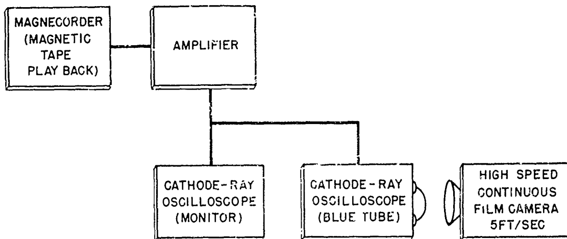
Fig. 2.16 Magnetic Tape to Film Record System
