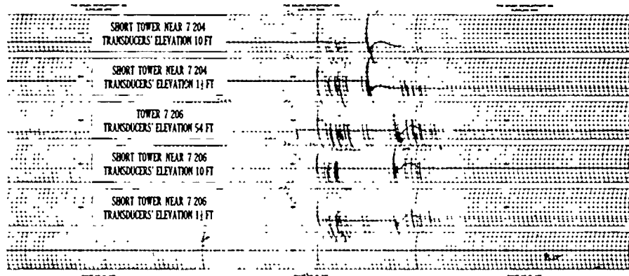
Fig. 2.13 Velocity Vs Time Field Records Tumbler 2. Increasing velocity downward. Increasing time to the right.
