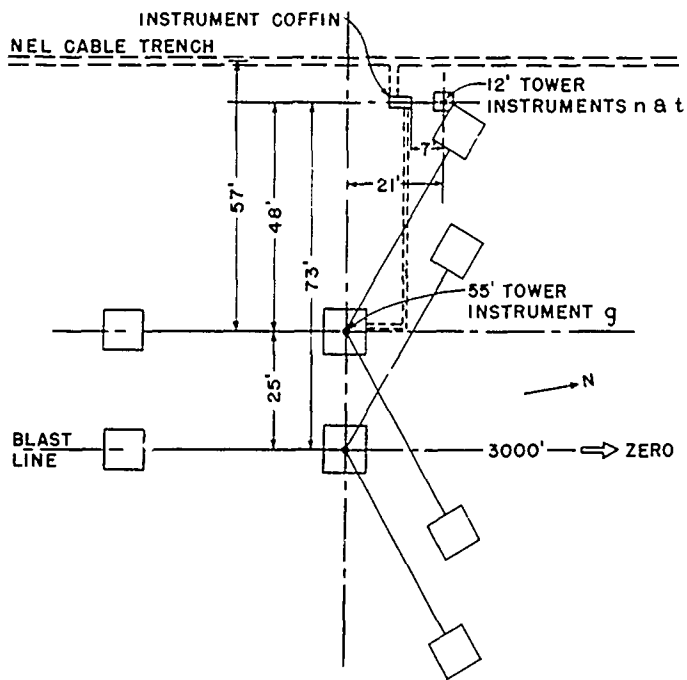
Fig. 2.8 7-204 Layout
