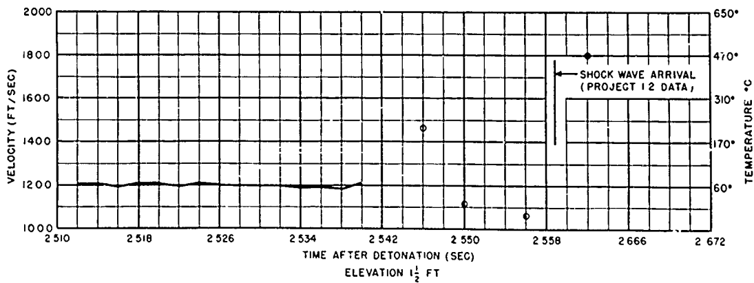
Fig. 3.12 Acoustic Velocity Vs Time Curves Tumbler 3, Tower 204
