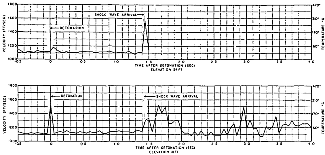
Fig. 3.7 Acoustic Velocity Vs Time Curves Tumbler 4, Tower 204
