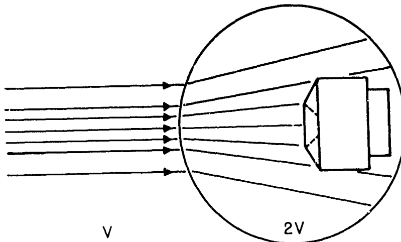
Fig. 4.1 Refraction Due to Hot Air Surrounding Receiver
