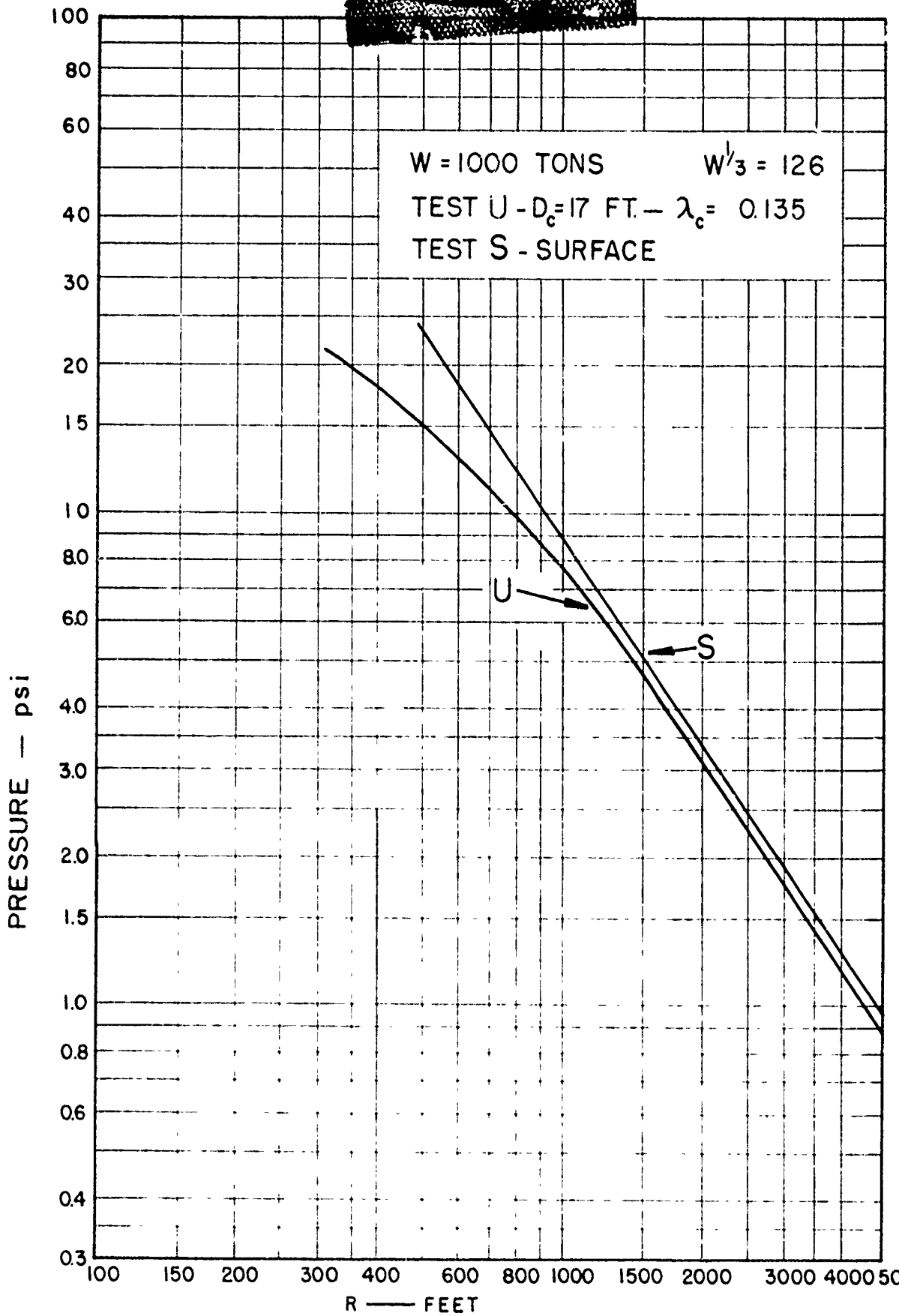
FIGURE 6 PEAK AIR - BLAST PRESSURE TEST U AND TEST S
