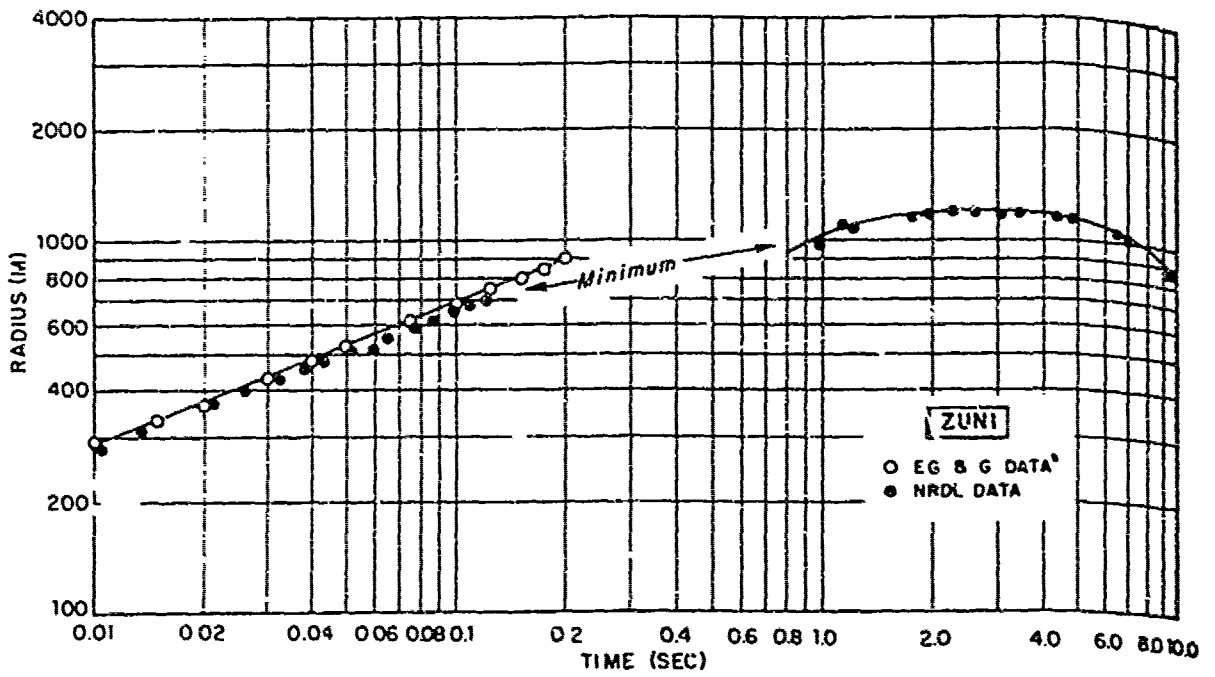
Figure 8.11 Shot Zuni fireball radius versus time.
