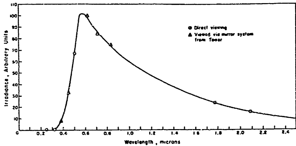
Figure 8.17 Relative spectral distribution of irradiance at t_{max_3} , Shot Zuni, Site Nan, composite, Project 8.1.
