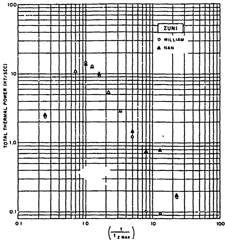
Figure 8.3 Total thermal power versus time, Shot Zuni.
