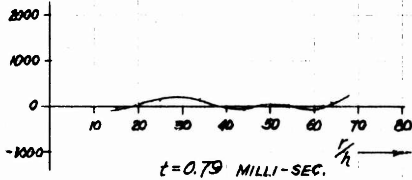
STRAIN VS. DISTANCE FROM POINT OF IMPACT RESULTING FROM ELASTIC IMPACT. TIME MEASURED FROM START OF OSCILLOGRAPH SWEEP.
