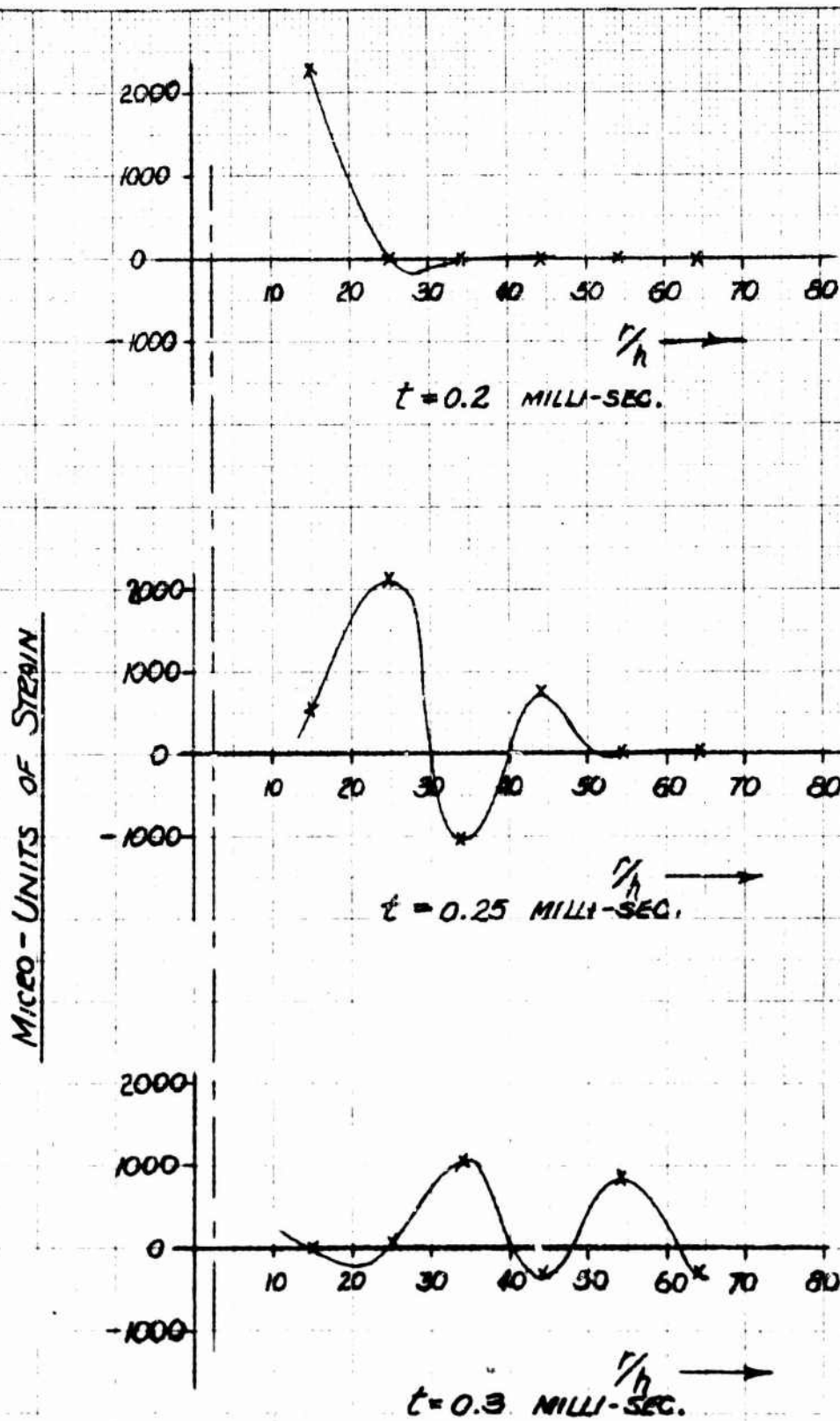
STRAIN VS. DISTANCE FROM POINT OF IMPACT FIG. 19A RESULTING FROM COMPLETE PENETRATION. TIME MEASURED FROM START OF OSCILLOGRAPH SWEEP.
