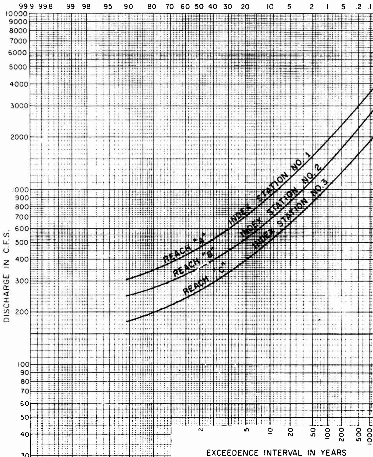
TURKEY CREEK SUMTER, S. C. DISCHARGE—FREQUENCY CURVES
