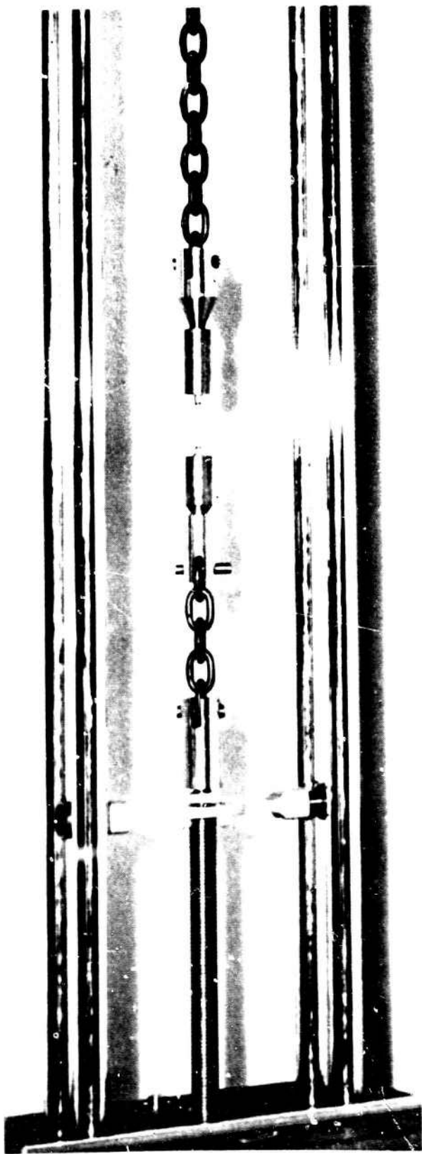
Fig. 5 Round Specimen Mounted in Tensile Machine Prior to Critical Straining
