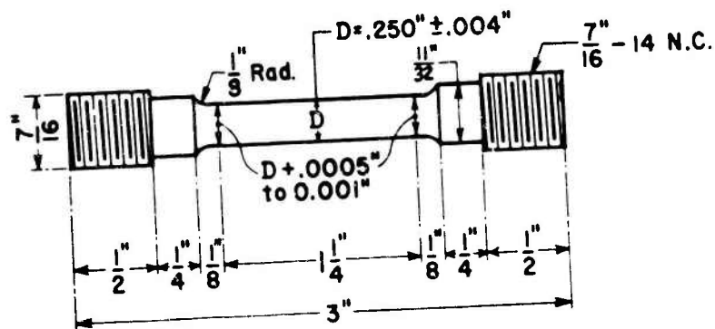
ROUND TENSILE SPECIMEN
