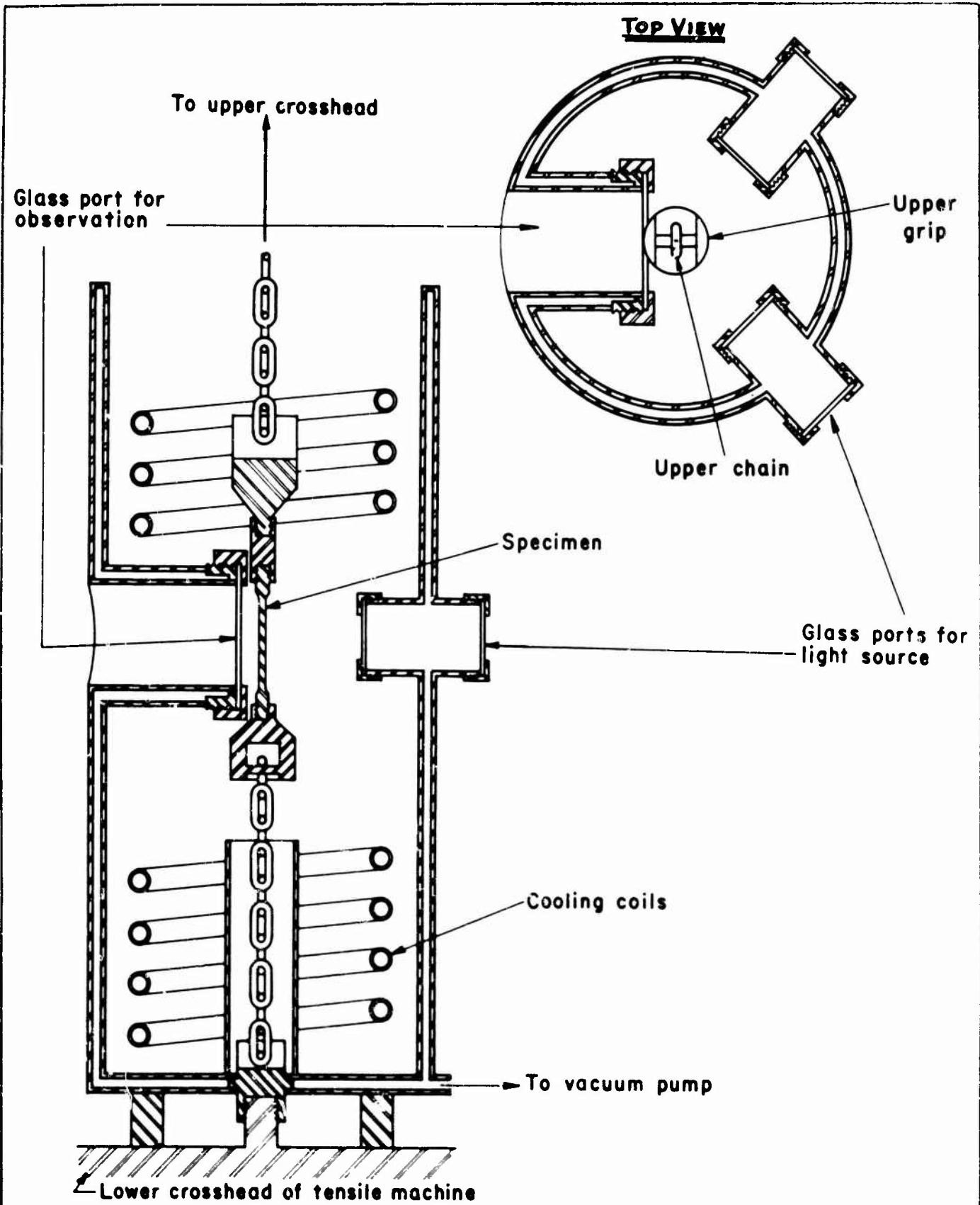
Fig. 7 Schematic Diagram of Low-Temperature Tensile Test Apparatus
