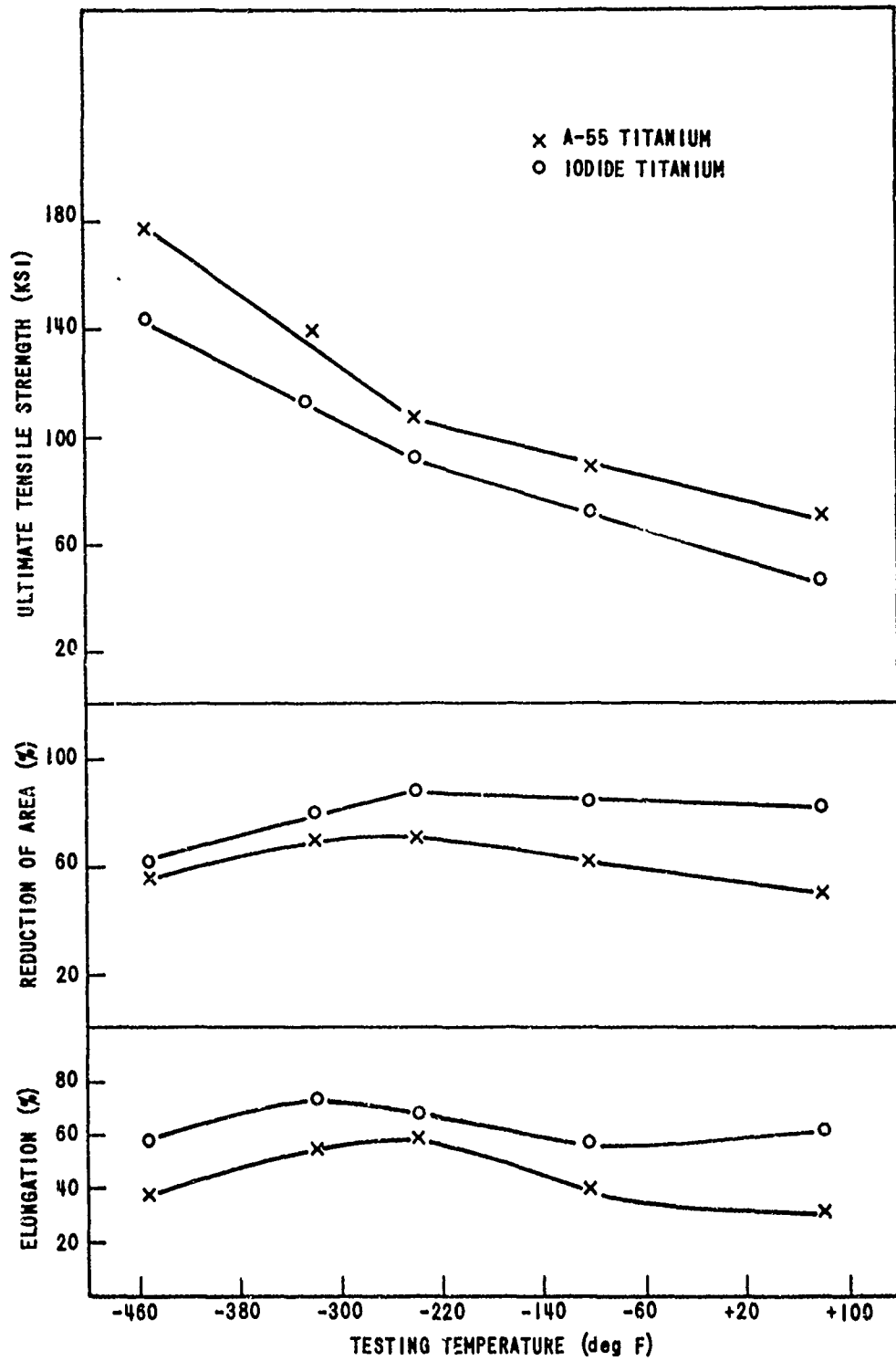
ENGINEERING TENSILE PROPERTIES OF COMMERCIALY PURE AND IODIDE TITANIUM AT VARIOUS TEMPERATURES
