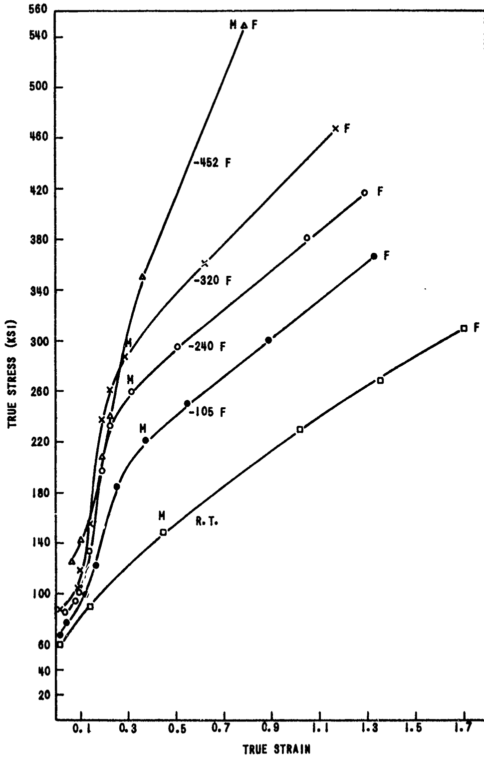
TRUE STRESS-STRAIN CURVES OF AISI 302 STAINLESS STEEL AT VARIOUS TEMPERATURES
