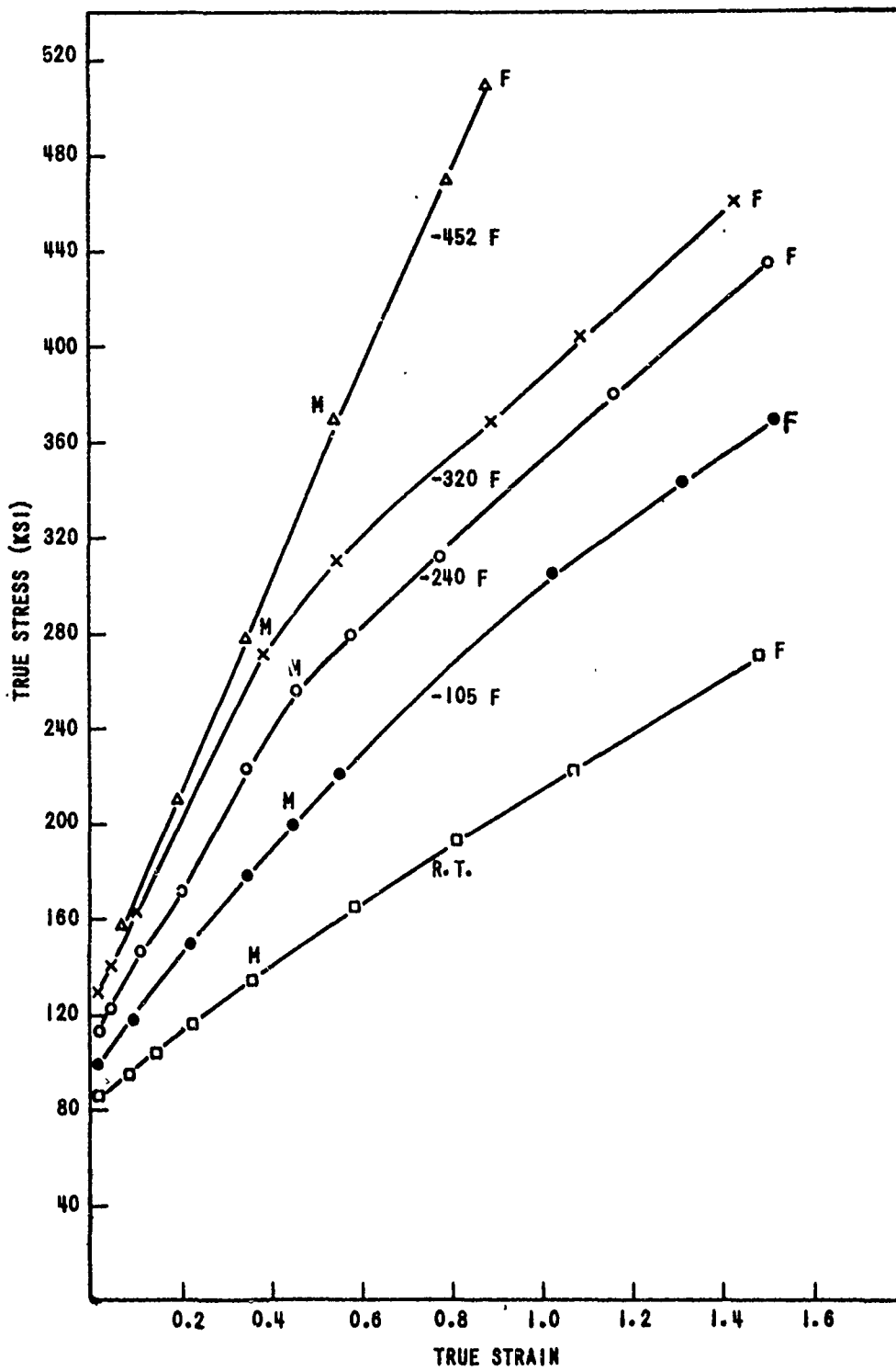
TRUE STRESS-STRAIN CURVES OF AISI 316 STAINLESS STEEL AT VARIOUS TEMPERATURES
