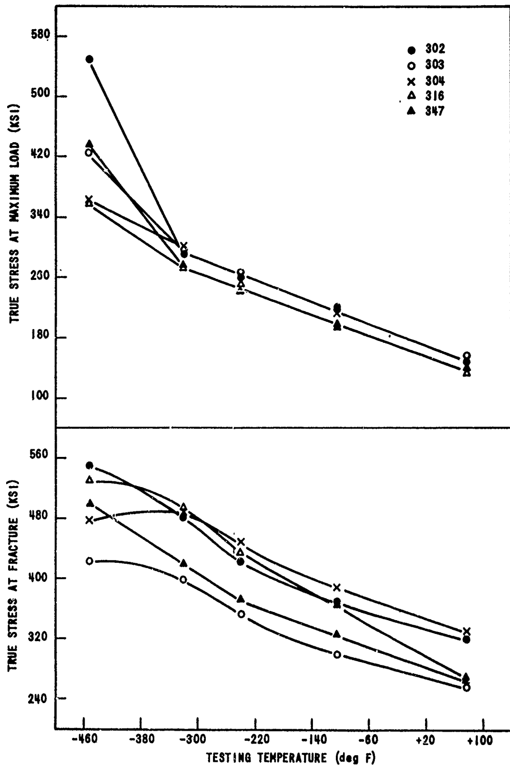
EFFECT OF TEMPERATURE ON TRUE STRESS AT FRACTURE AND MAXIMUM LOAD
