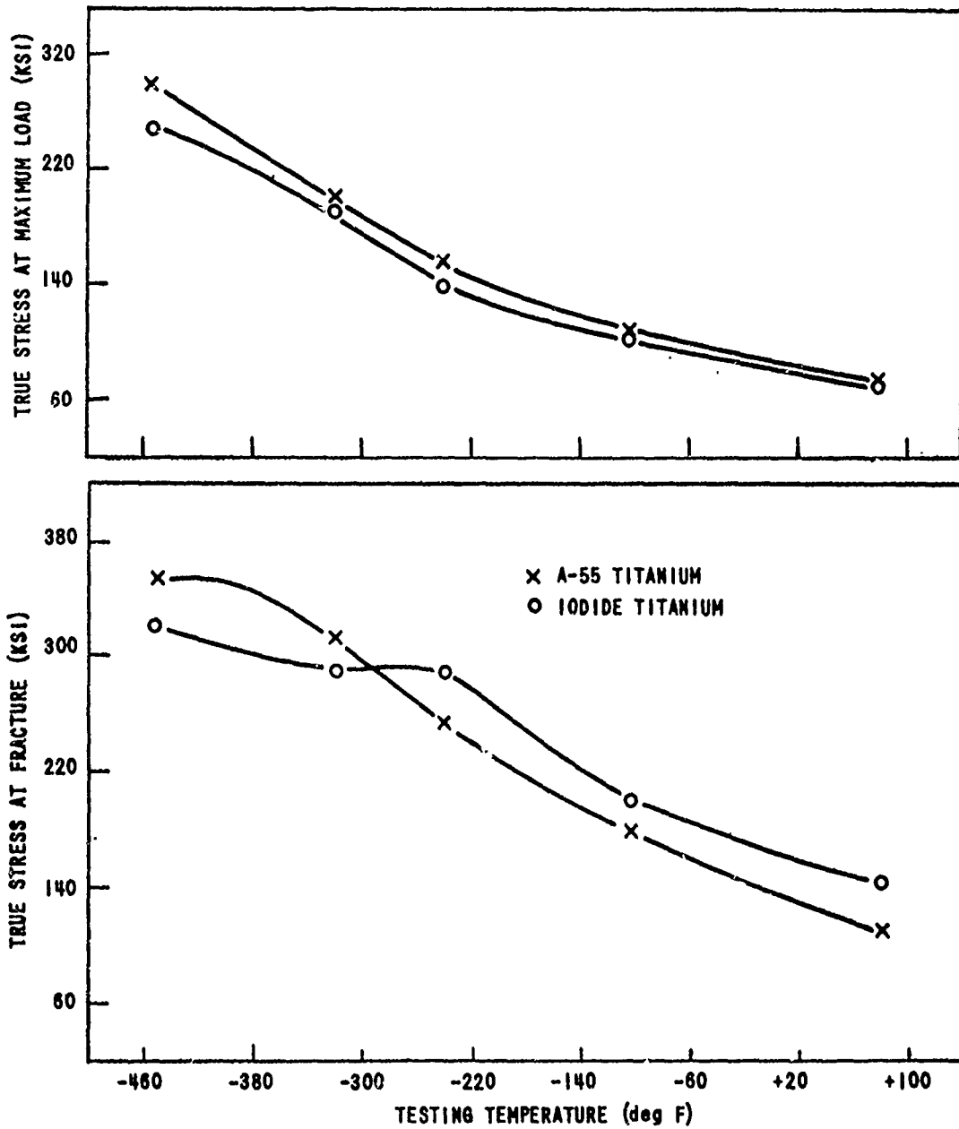
EFFECT OF TEMPERATURE ON TRUE STRESS AT FRACTURE AND MAXIMUM LOAD
