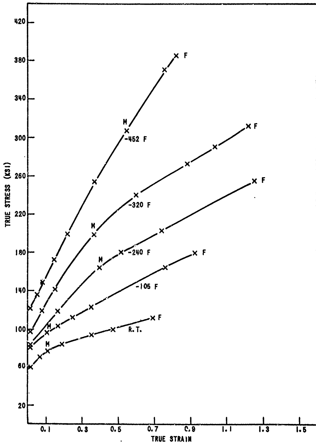
TRUE STRESS-STRAIN CURVES OF A-55 TITANIUM AT VARIOUS TEMPERATURES
