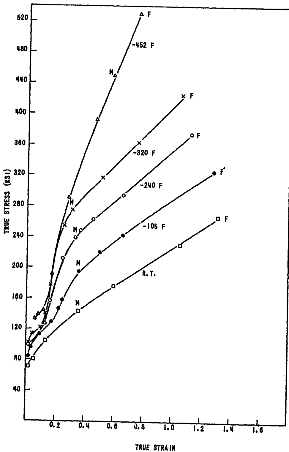
TRUE STRESS-STRAIN CURVES OF AISI 347 STAINLESS STEEL AT VARIOUS TEMPERATURES
