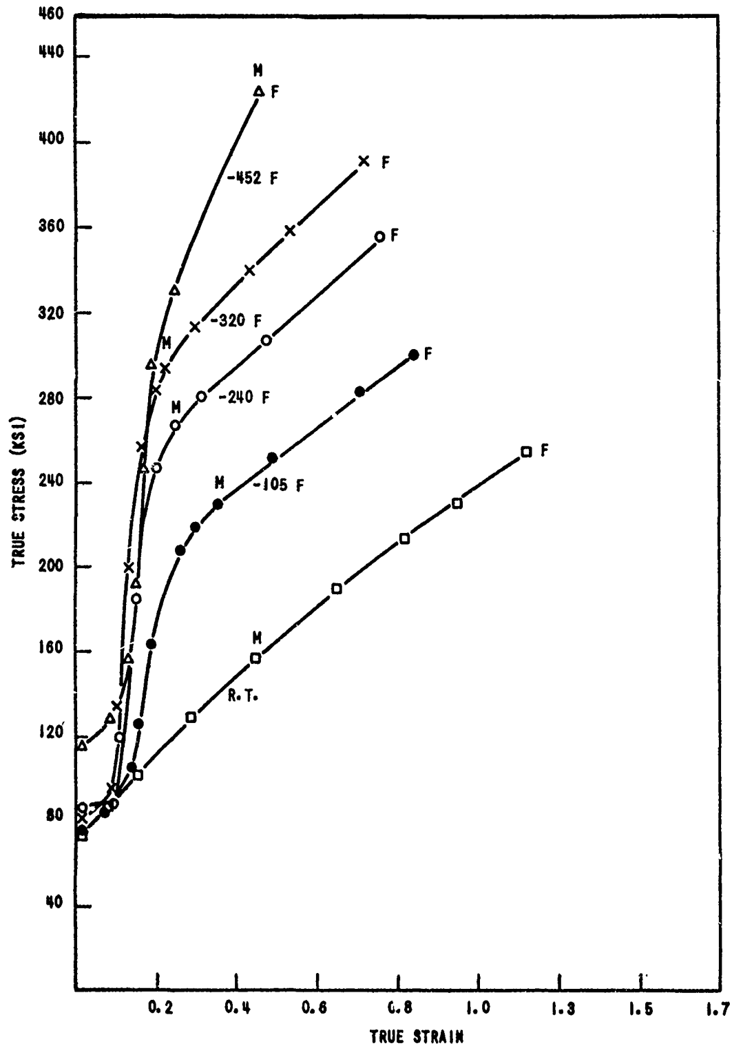
TRUE STRESS-STRAIN CURVES OF AISI 303 STAINLESS STEEL AT VARIOUS TEMPERATURES
