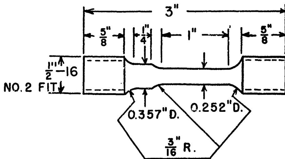
LOW-TEMPERATURE TENSILE SPECIMEN
