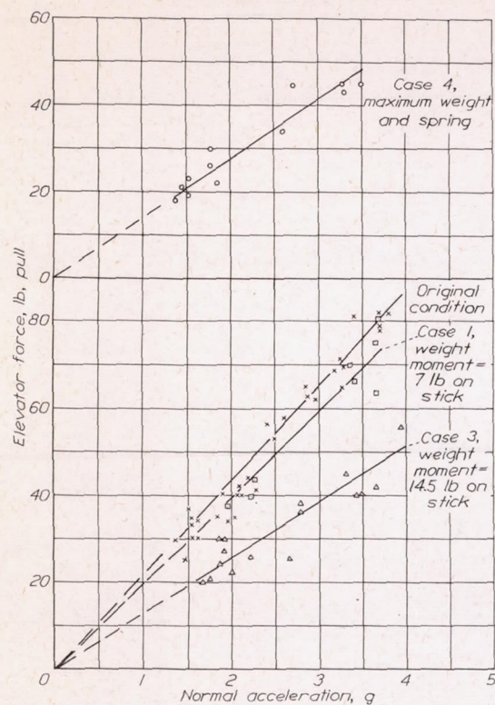
Figure 20.- Variation of elevator force with normal acceleration in 180^\circ turns made at various speeds; Brewster XSBA-1 airplane in original condition and with three arrangements of weights and springs.
