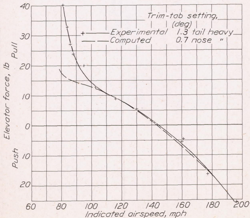
Figure 18.- Variation of stick force with indicated airspeed in the climbing condition for case 4, maximum weight moment offset by spring. Brewster XSBA-1 airplane.
