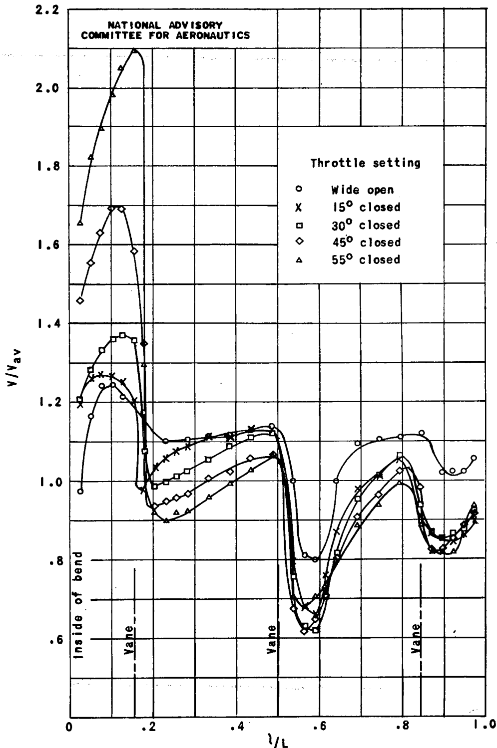
Figure 4. - Effect of throttle angle on velocity profile at vaned-elbow outlet, station 3.
