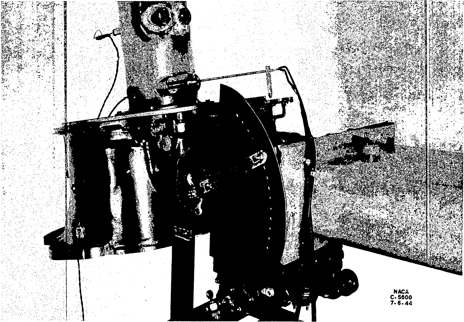
Figure 2. - Installation of carburetor-elbow assembly in duct-component test rig.
