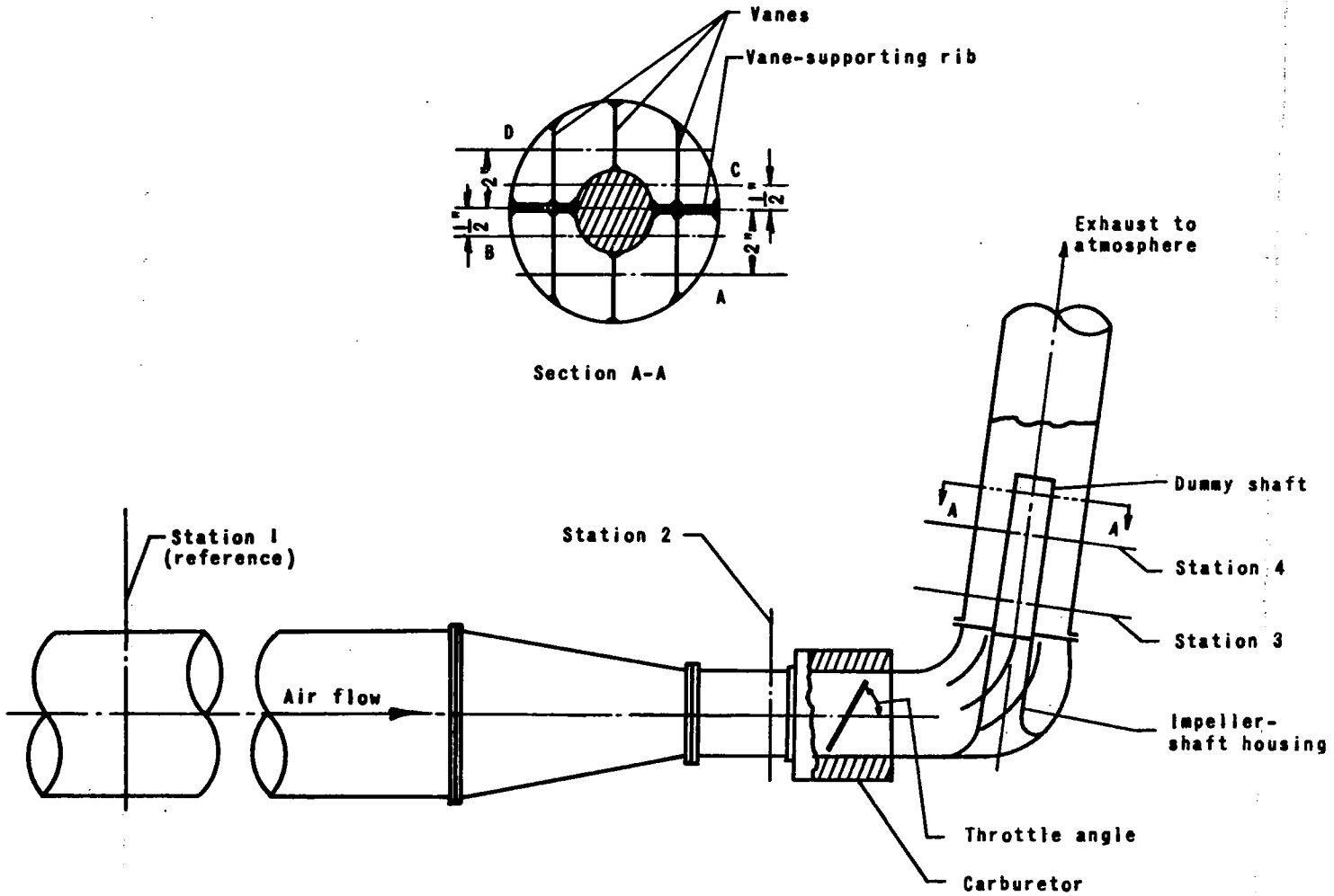
Figure 1. - Schematic diagram of carburetor and inlet elbow.
