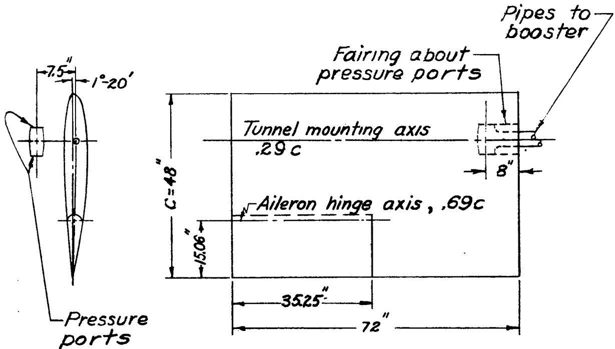
Figure 2. - Wing model details.
