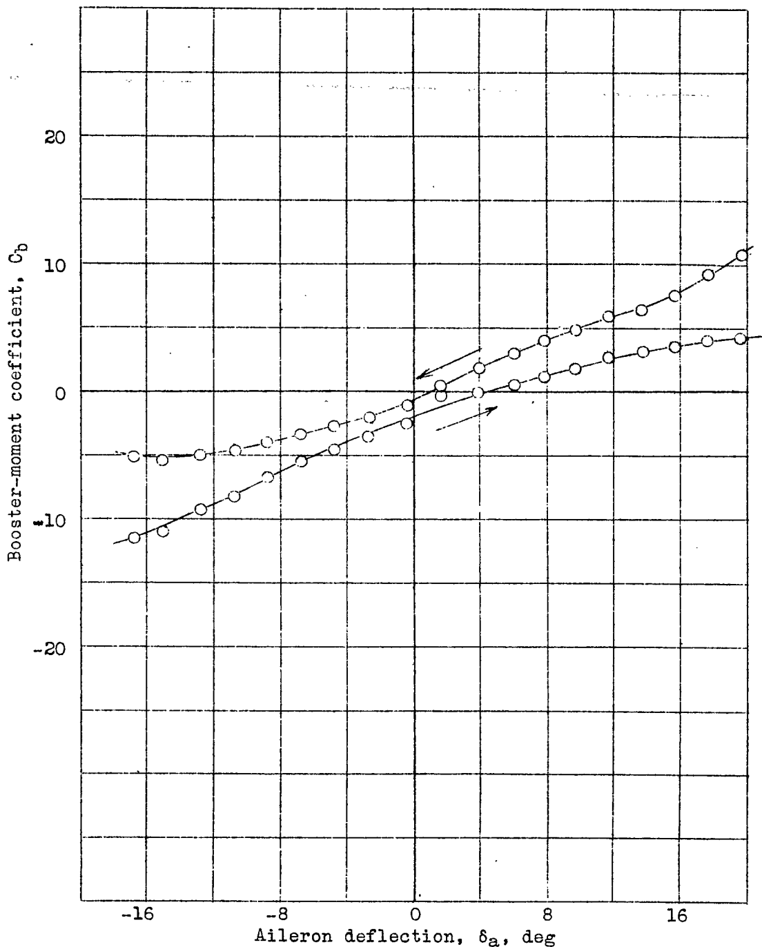
Figure 5.- Effect of friction on the booster-moment coefficient. Moments were recorded while rotating the booster mechanism in the direction indicated by the arrows. \alpha = 0^\circ ; q = 25 pounds per square foot.
