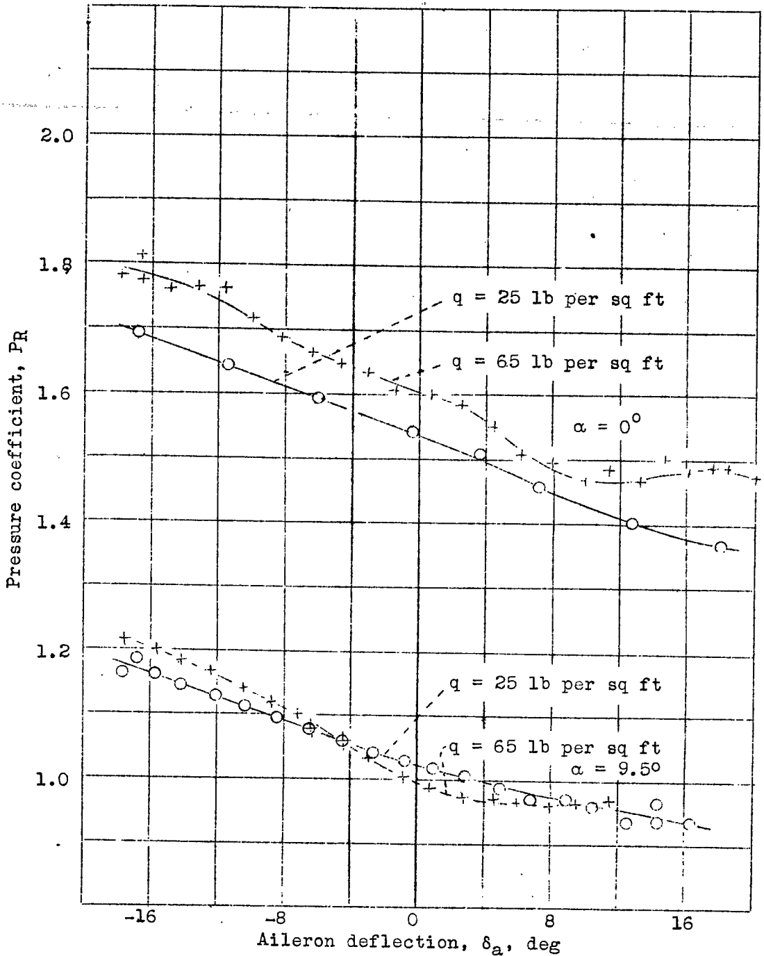
Figure 8.- Pressure coefficients at various aileron angles for the piston-type control booster.
