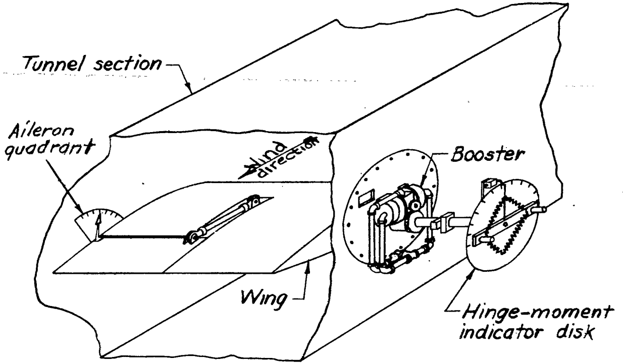
Figure 1. - Schematic diagram of test installation.
