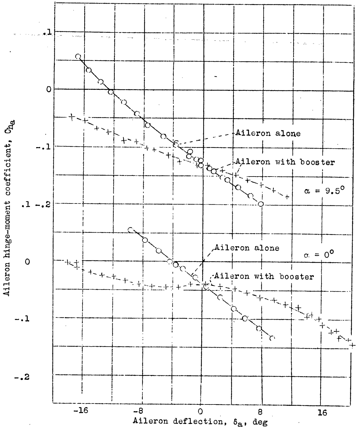
Figure 7.- Effect of the piston-type control booster on aileron hinge-moment coefficients. q = 65 pounds per square foot.
