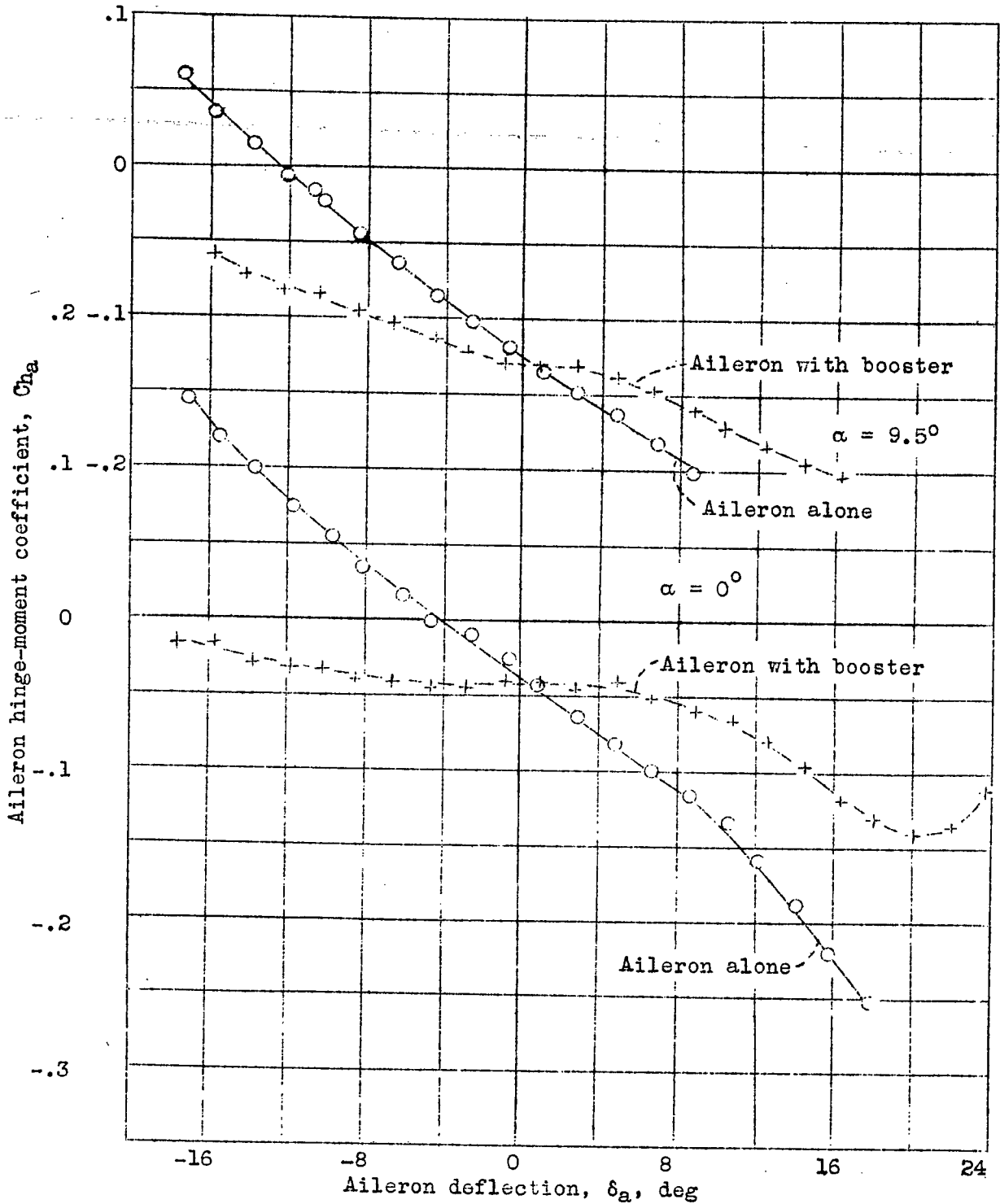
Figure 6.- Effect of the piston-type control booster on aileron hinge-moment coefficients. q = 25 pounds per square foot.
