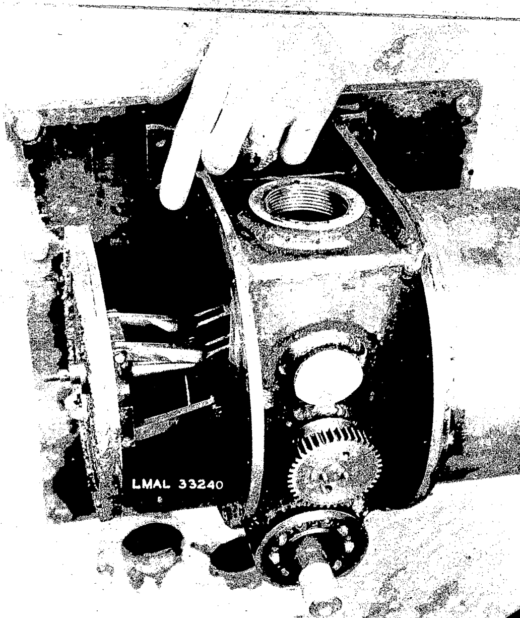
Figure 4.- Photograph of booster mechanism.
