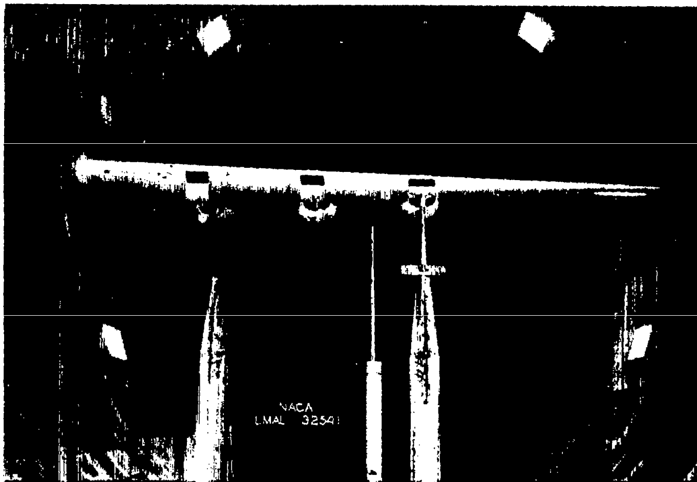
Figure 24.- Partial-span tapered wing model with end plate mounted in Langley 19-foot pressure tunnel.
