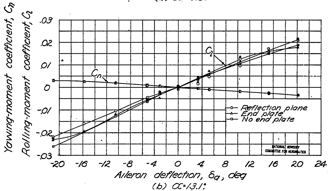
Figure 31.—The corrected aileron characteristics of the tapered-wing model for three end conditions. Flaps neutral; R \approx 8.9 \times 10^6 ; M \approx 0.17 .
