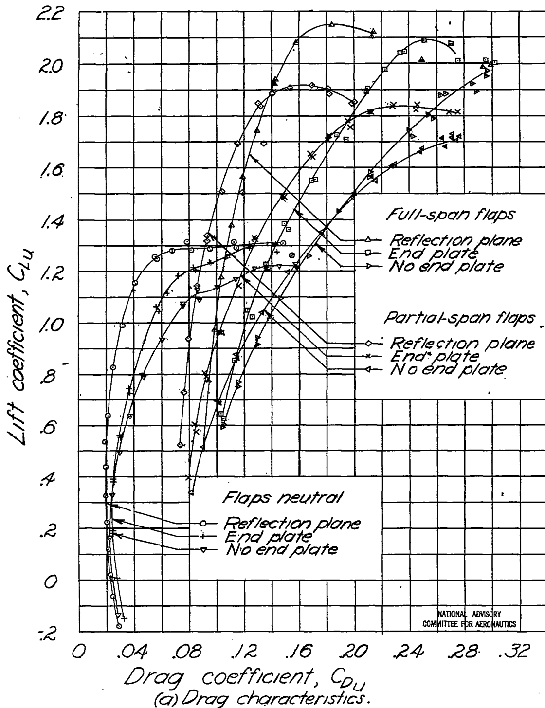
Figure 26.-The uncorrected aerodynamic characteristics of the tapered-wing model for three flap arrangements and three end conditions. R \approx 8.9 \times 10^6 ; M \approx 0.17 .
