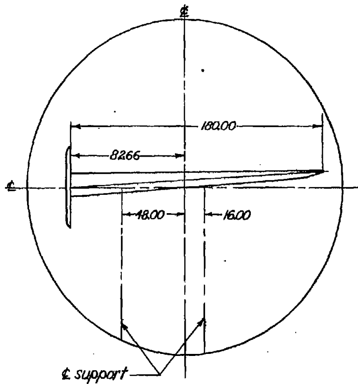
Figure 13.- General arrangement of tapered-wing model and the end plate in the Langley 19-foot pressure tunnel. (All dimensions in inches.)
