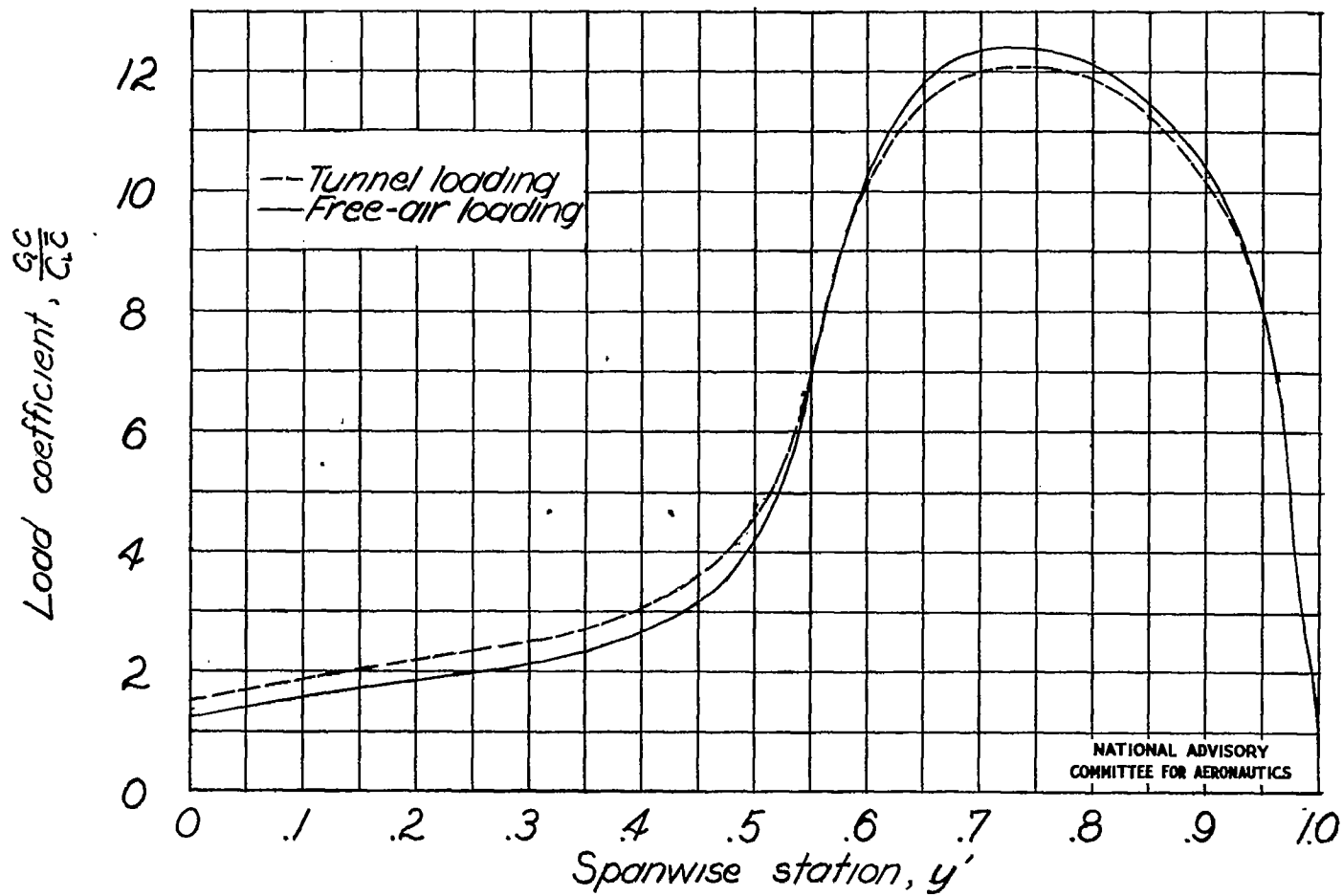
Figure 16.- Comparison of the free-air and tunnel span load distribution due to the aileron deflection. End-plate condition.
