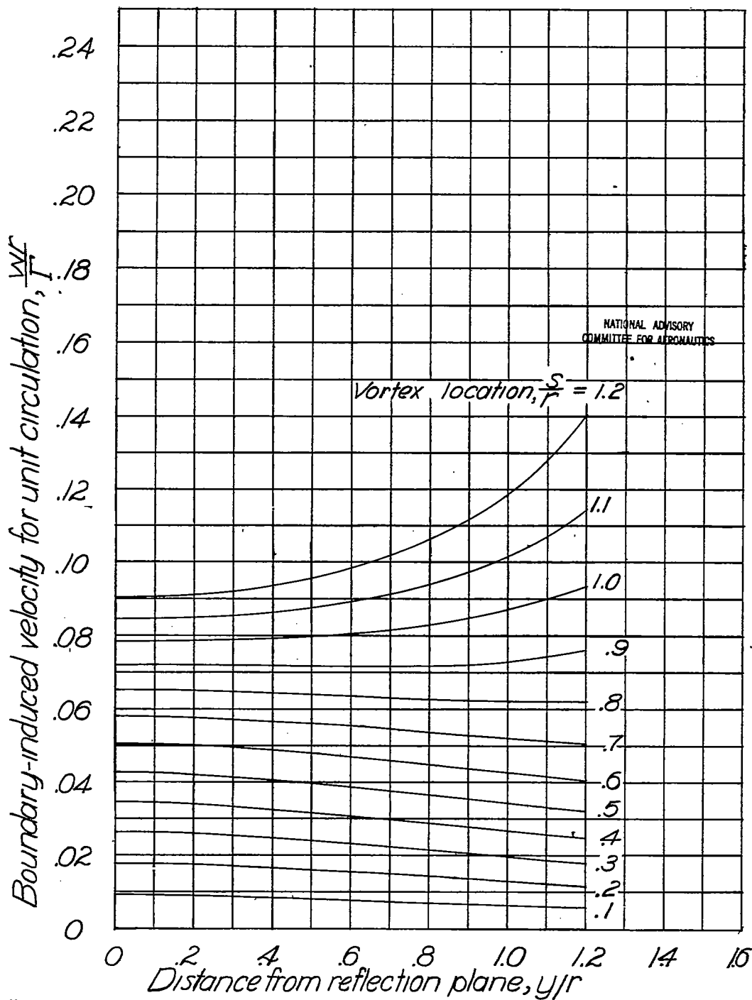
Figure 3. - Boundary-induced velocity along the horizontal center line due to a unit counterclockwise vortex at various distances \frac{s}{r} from the reflection plane. \frac{\rho}{r} = 0.49781 .
