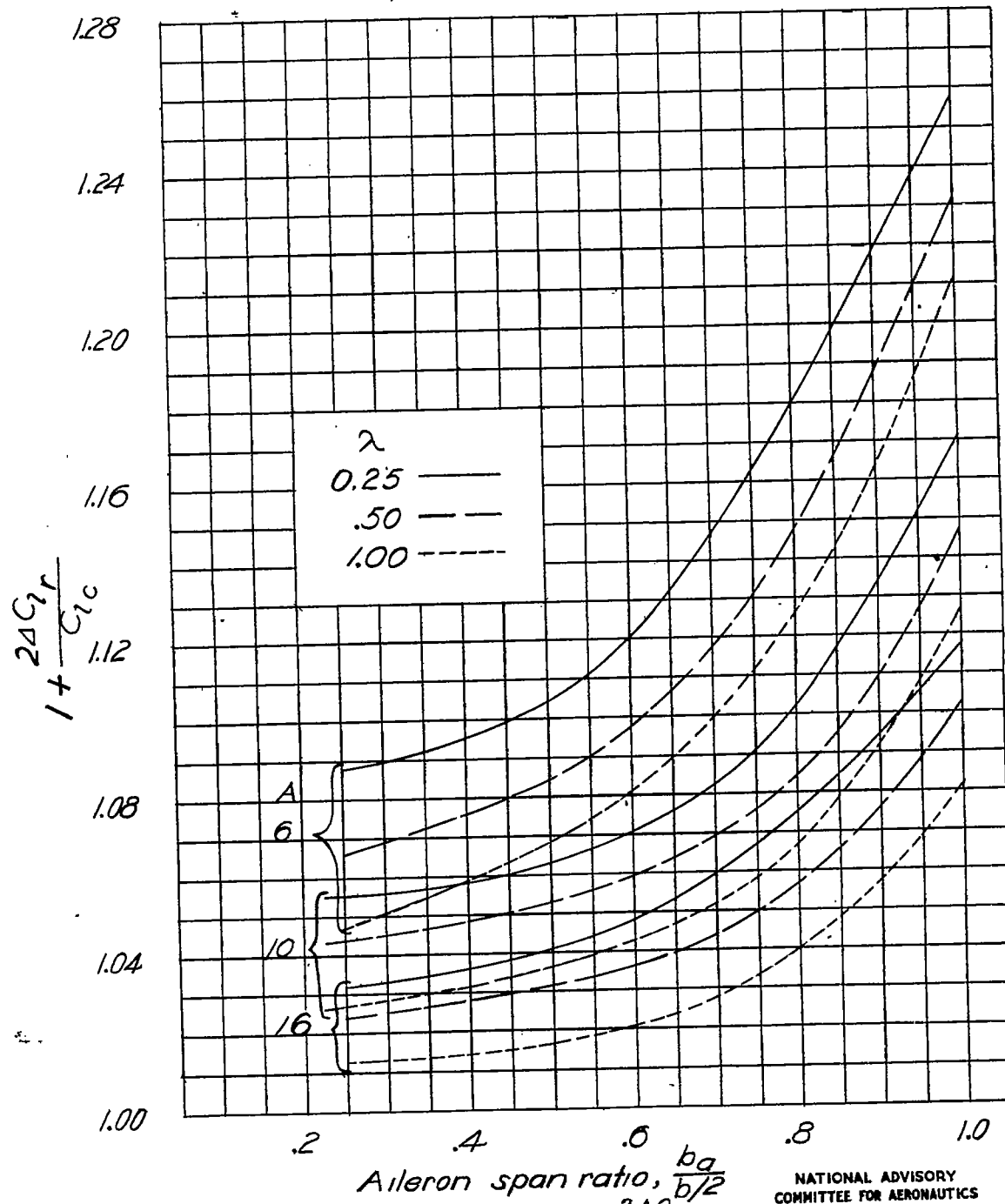
Figure 10.-Values of the factor 1 + \frac{2\Delta C_r}{C_{lc}} used to account for the effect of the reflection plane on the rolling-moment coefficient for ailerons extending inboard from the tips of the wings of reference 8. (From reference 3.)
