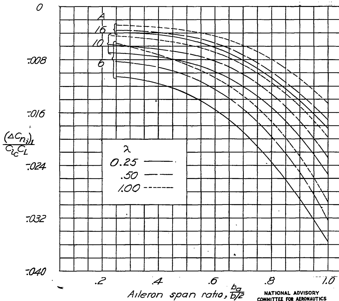
Figure 11 - Increment of yawing-moment-coefficient correction due to the reflection plane for ailerons extending in-board from the tips of the wings of reference 8. (From reference 3.)
