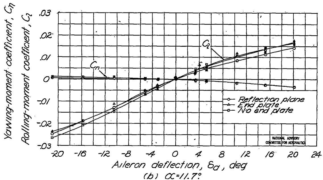
Figure 32.-The corrected aileron characteristics of the tapered-wing model for three end conditions. Partial-span flaps; R \approx 8.9 \times 10^6 ; M \approx 0.17 .
