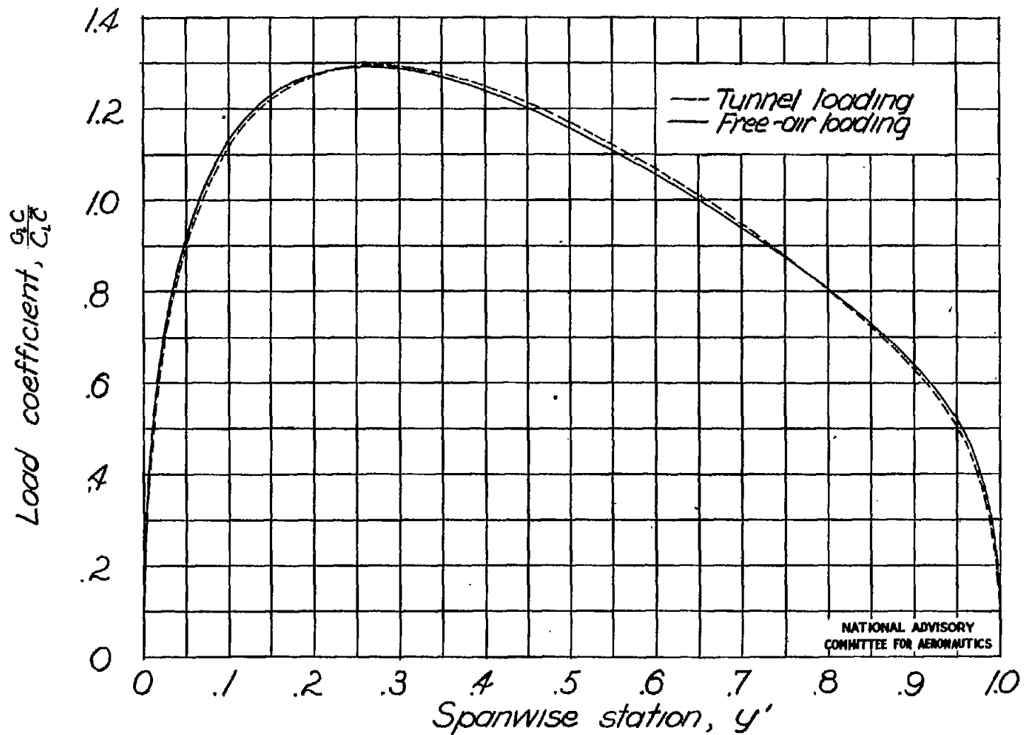
Figure 19.- Comparison of the free-air and tunnel span load distributions. No end plate.
