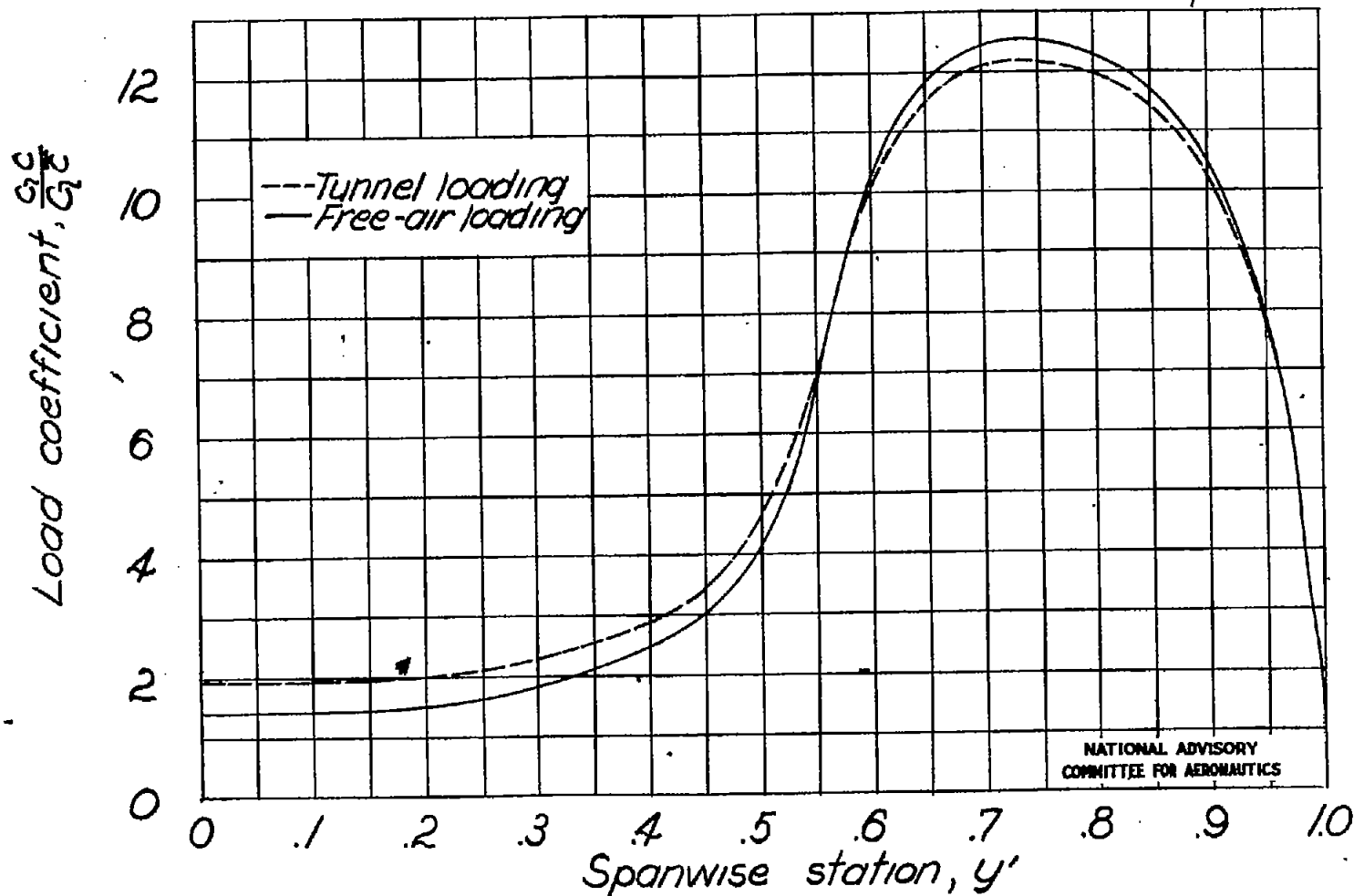
Figure 8. - Comparison of the free-air and tunnel span load distribution due to the aileron deflection. Reflection-plane condition.
