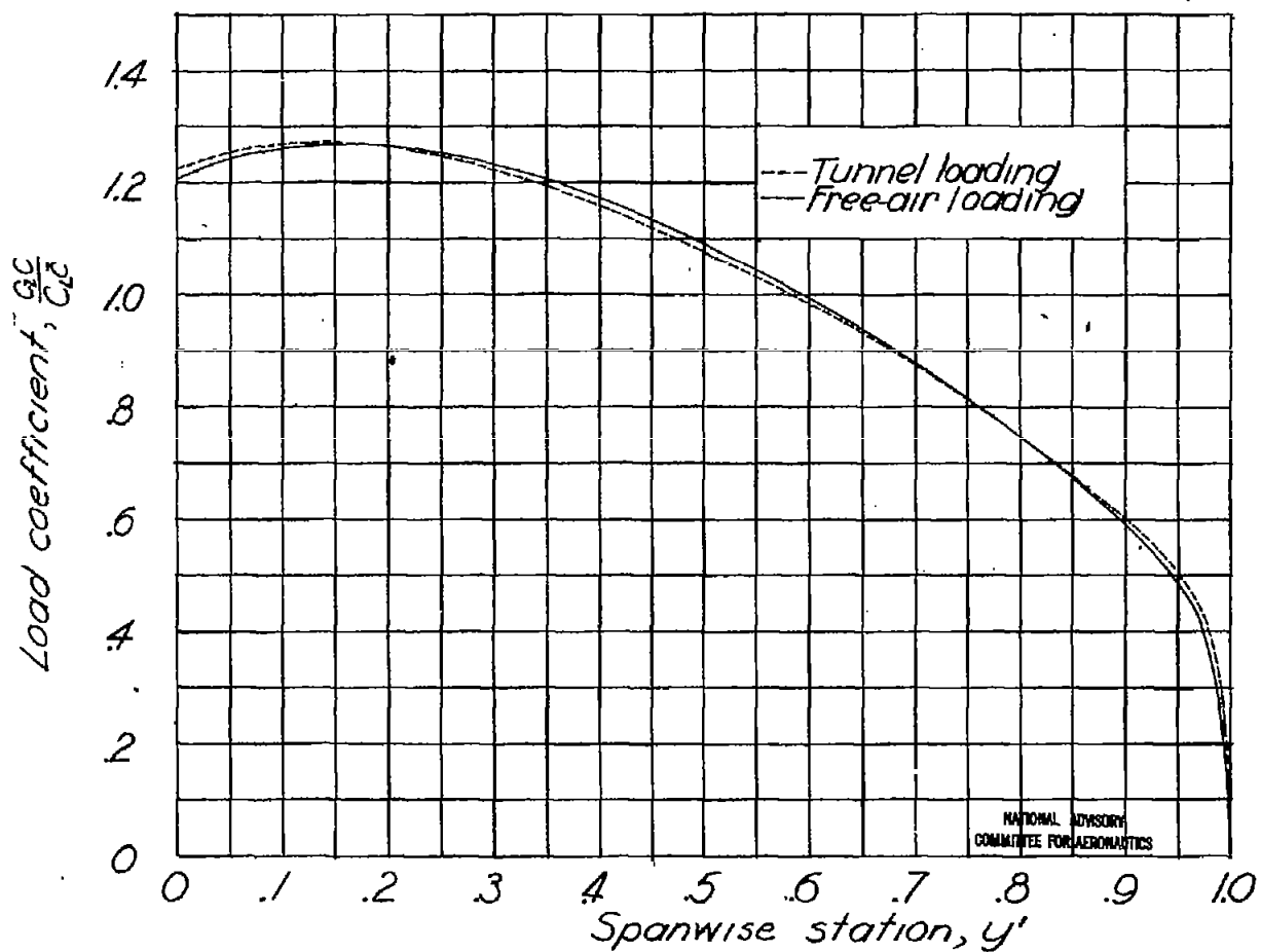
Figure 14. - Comparison of the free-air and tunnel span load distribution. End-plate condition.
