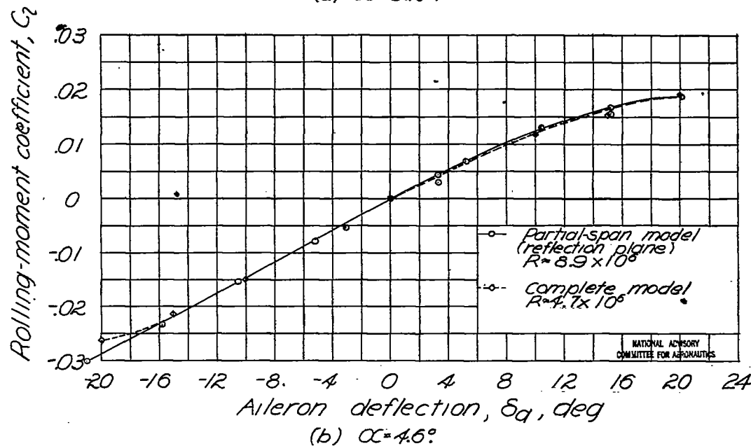
Figure 34.-Comparison of the aileron effectiveness of the partial-span tapered-wing model and the complete-span model. Flaps neutral, M \approx 0.17 .
