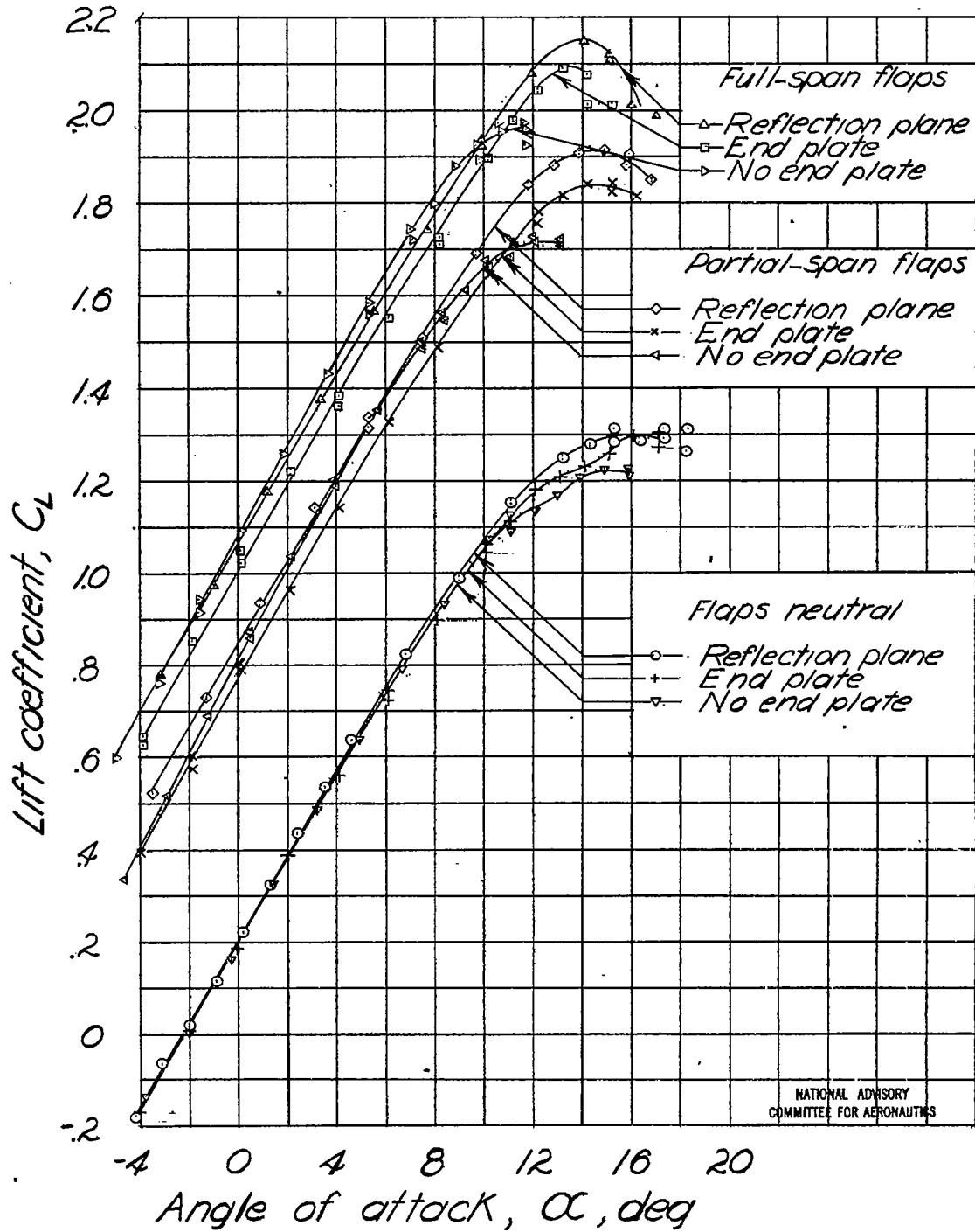
(b) Lift characteristics. Figure 30.-Continued.
