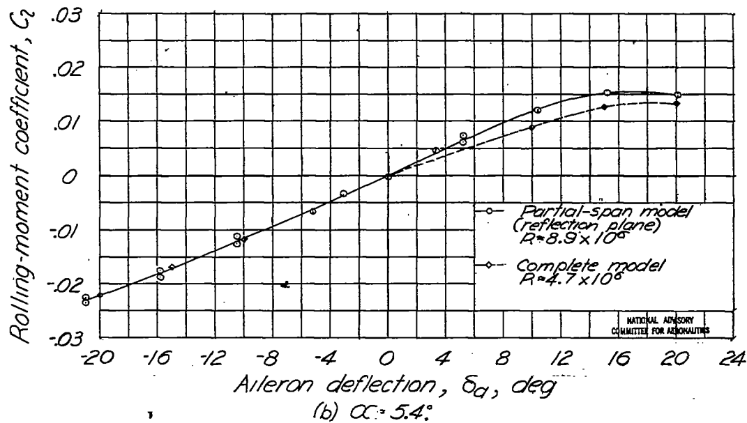
Figure 35.—Comparison of the aileron effectiveness of the partial-span tapered-wing model and the complete-span model. Full-span flaps deflected, M \approx 0.17 .
