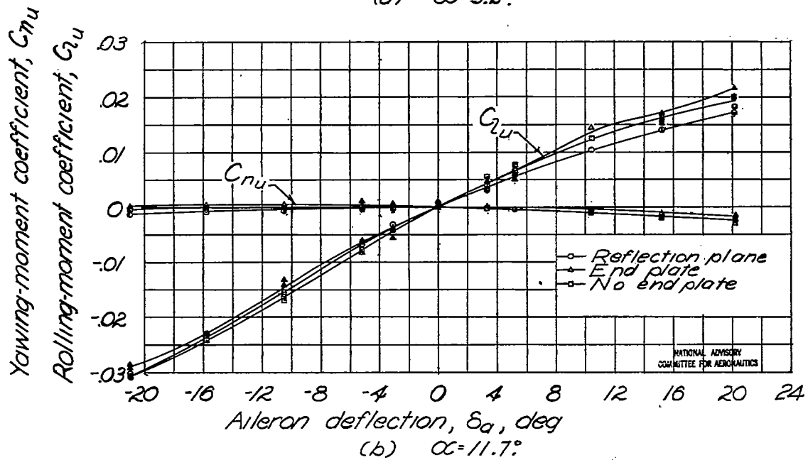
Figure 28 --The uncorrected aileron characteristics of the tapered-wing model for three end conditions. Partial-span flaps, R \approx 8.9 \times 10^6 ; M \approx 0.17 .
