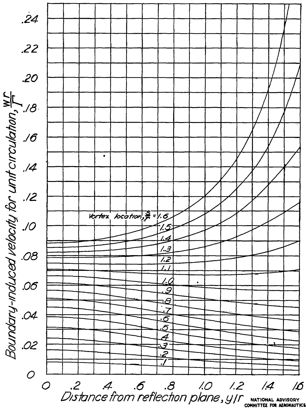
Figure 2.-Boundary-induced velocity along the horizontal center line due to a unit counterclockwise vortex at various distances \frac{s}{r} from the reflection plane. \frac{c}{r} = 0.73026 .
