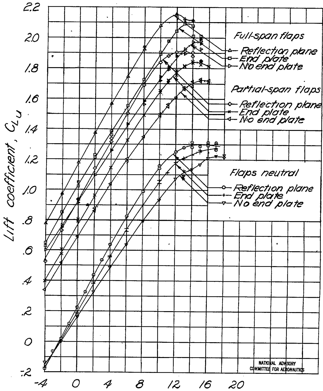
(b) Lift characteristics.
