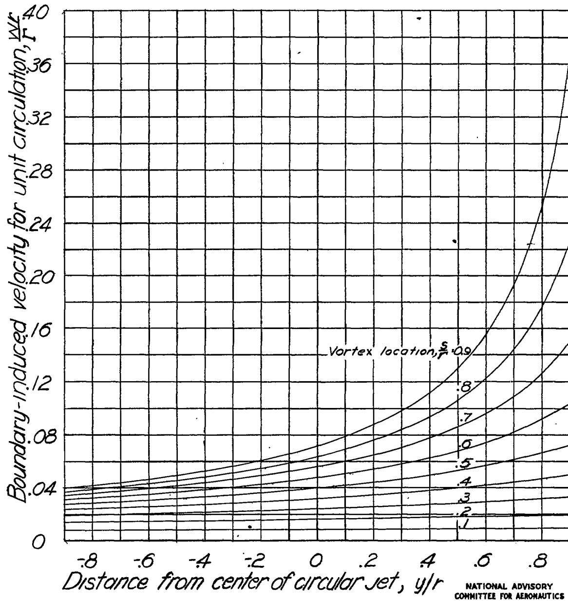
Figure 18.-Boundary-induced velocity along the horizontal center line due to a unit counterclockwise vortex at various distances \frac{z}{r} from the center of a circular jet.
