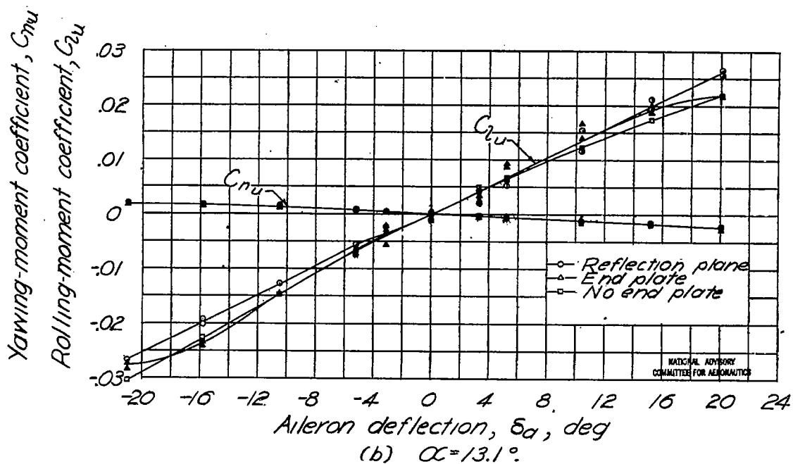
Figure 27-The uncorrected aileron characteristics of the tapered-wing model for three end conditions. Flaps neutral, R \approx 8.9 \times 10^6 , M \approx 0.17 .
