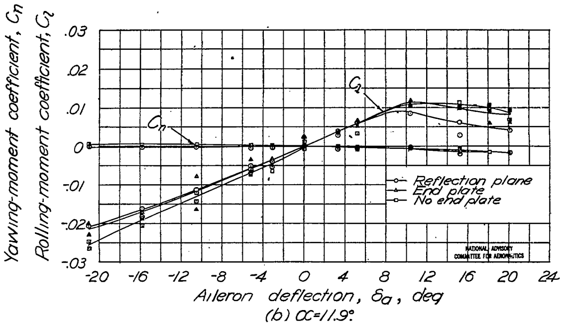
Figure 33.- The corrected aileron characteristics of the tapered-wing model for three end conditions. Full-span flaps; R \approx 8.9 \times 10^6 ; M \approx 0.17 .
