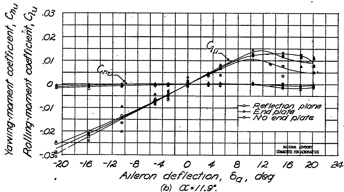
Figure 29.—The uncorrected aileron characteristics of the tapered-wing model for three end conditions. Full-span flaps; R \approx 8.9 \times 10^6 ; M \approx 0.17 .
