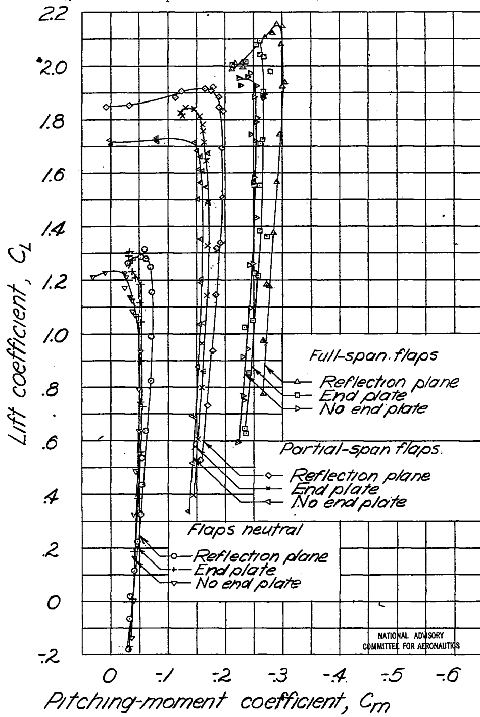
(c) Pitching-moment characteristics.
