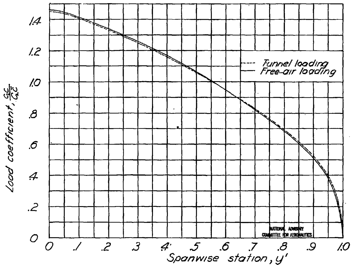
Figure 6 - Comparison of the free-air and tunnel span load distribution. Reflection-plane condition.
