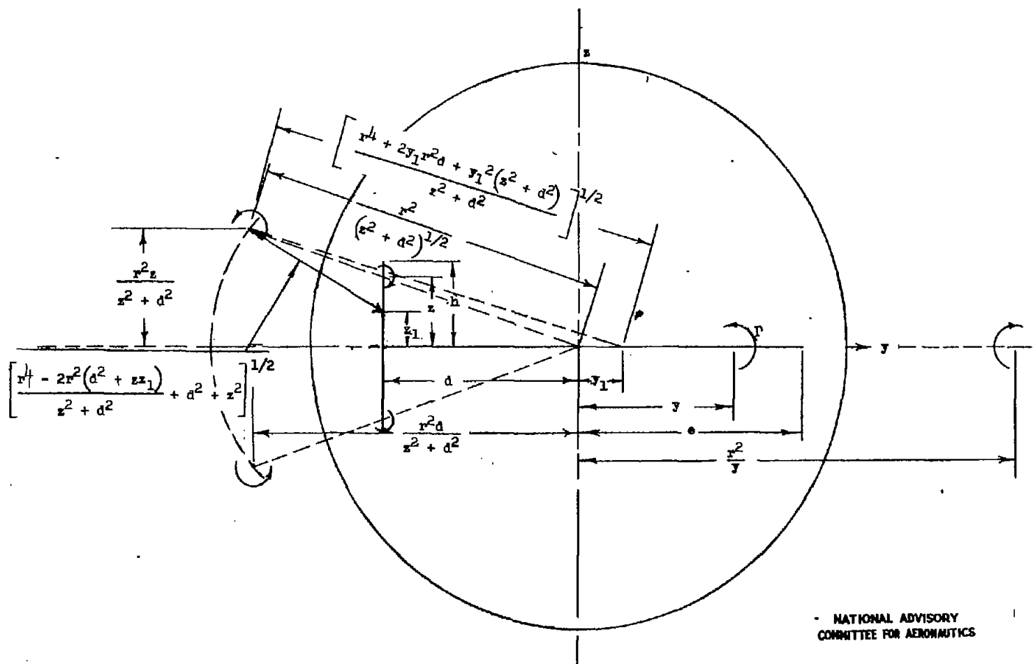
Figure 12.- Diagram of the model and end-plate trailing-vortex system and the corresponding reflected images.
