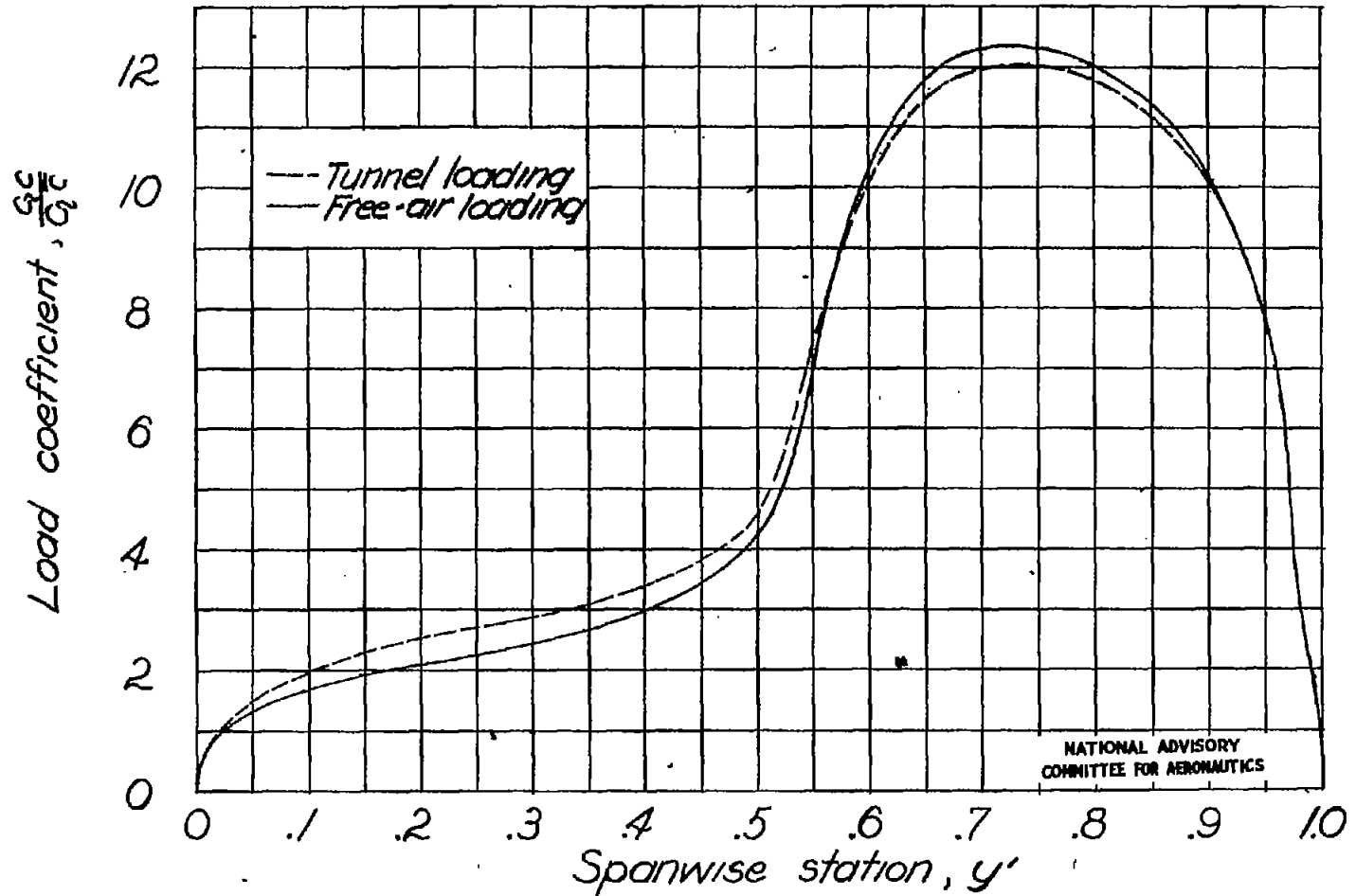
Figure 21.- Comparison of the free-air and tunnel span load distribution due to the aileron deflection. No end plate.
