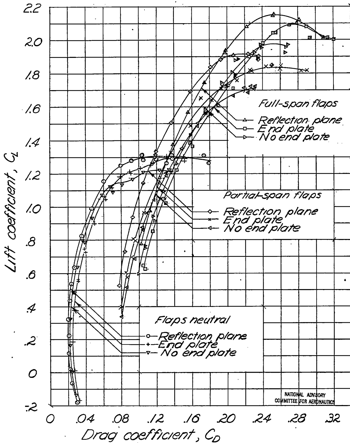
(a) Drag characteristics. Figure 30.-The corrected aerodynamic characteristics of the tapered-wing model for three flap arrangements and three end conditions. R \approx 8.9 \times 10^6 ; M \approx 0.17 .
