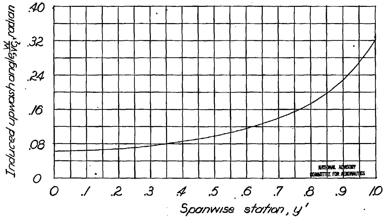
Figure 9.- Spanwise distribution of the boundary-induced upwash angle due to the aileron deflection. Reflection-plane condition.
