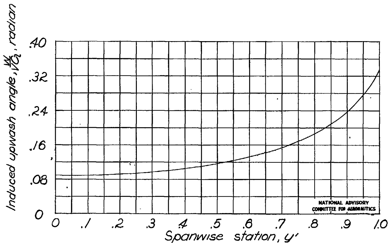
Figure 22.- Spanwise distribution of the boundary-induced upwash angle due to the aileron deflection. No end plate.
