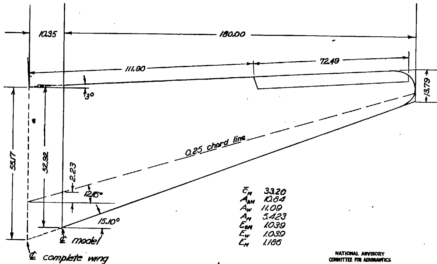
Figure 5.-Plan view and general dimensions of the tapered-wing model. (All dimensions in inches.)
