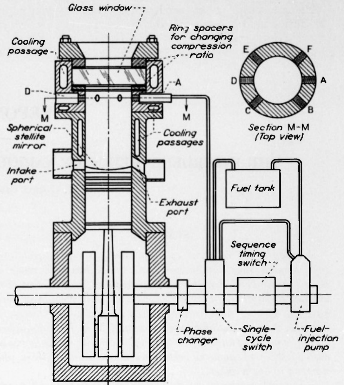
FIGURE 1.—Schematic diagram of full-view combustion apparatus.
