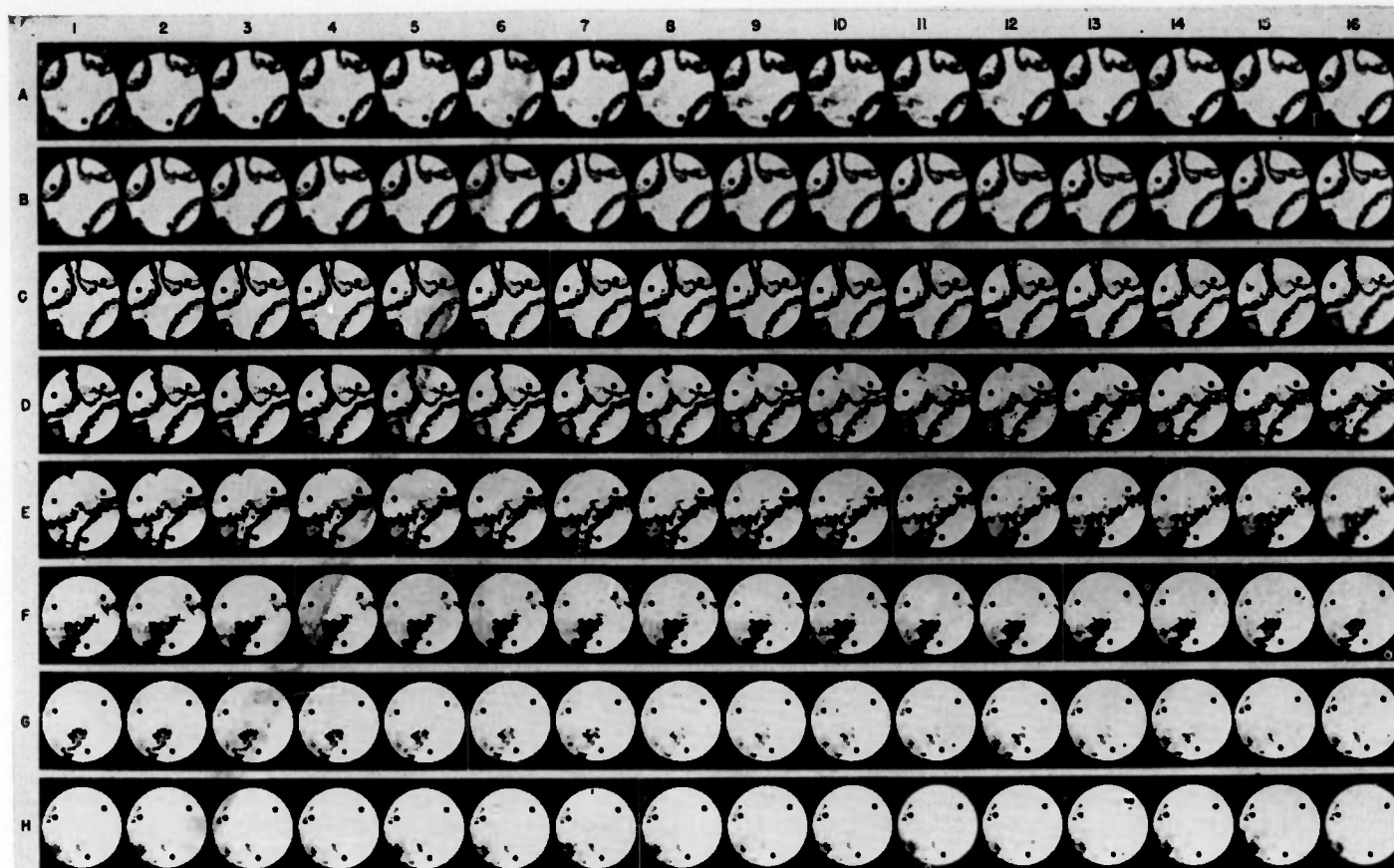
FIGURE 2.—High-speed motion picture of combustion of benzene showing occurrence of pin-point autoignition not followed by knock.
