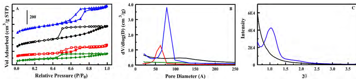
Fig. 8 — Alkyammonium-functionalized sorbents. (A) Nitrogen sorption isotherms for the base HX sorbent (blue, 566 m 2 /g, 77 Å); HX2M2B (red, 169 m 2 /g, 63 Å); the base CF sorbent (black, 523 m 2 /g, 111 Å); and CF2M2B (green, 143 m 2 /g, 93 Å). (B) Pore size distributions for materials (colored as in A). (C) The XRD spectrum for the base HX and CF sorbents. Functionalization of the HX and CF sorbents resulted in significant loss in surface area. Pore diameters for the functionalized materials were broadened and lacked a well-defined peak.
