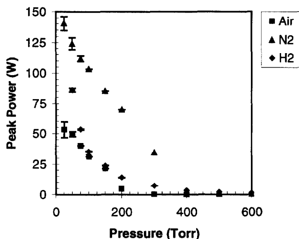
Figure 10. Peak photoemission power generated by corona in various gases and pressures at 500 Hz.
