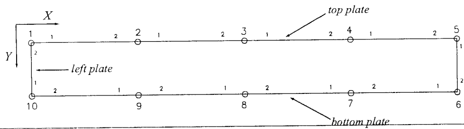
Figure 5. Cross-section of 2-D capsule with corner and branch numbers
