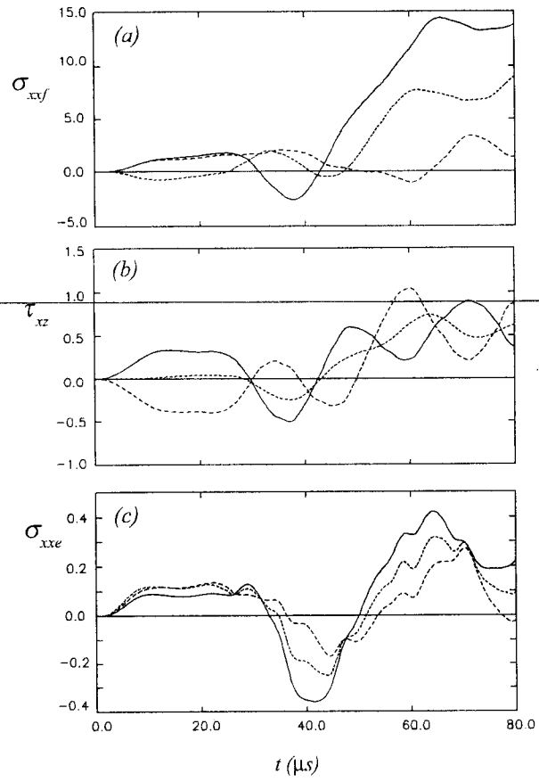
Figure 7. 2-D stress histories on left plate: (a) \sigma_{xxf} , (b) \tau_{xz} , (c) \sigma_{xze}
