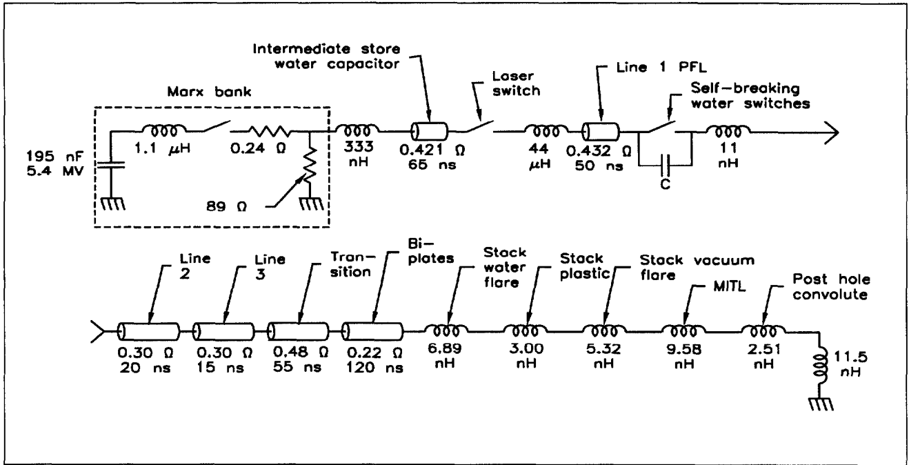
Figure 4. SCREAMER circuit model of one level of the Z-accelerator
