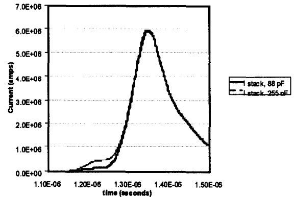
Figure 5. SCREAMER output current predictions for one level of the Z-accelerator.
