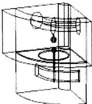
Figure 2. One quadrant of the waterline switch with prepulse shield.
