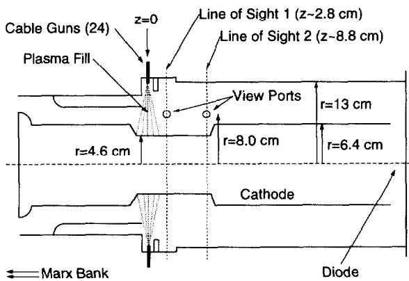
Figure 2. Schematic of POS region of DM1.
