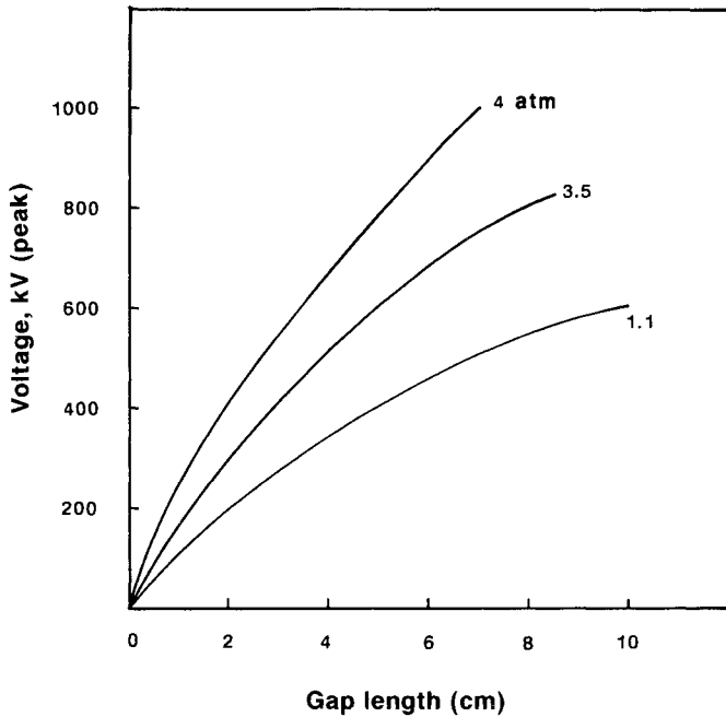
Fig. 5. Breakdown voltage vs gap length for different SF 6 pressures (from Ref. 9).
