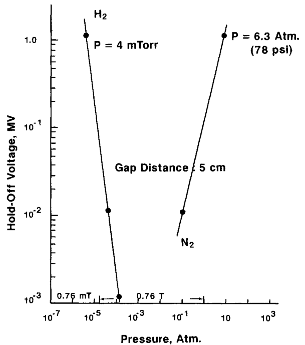
Fig. 4. Breakdown voltage vs gas pressure for the gap distance of 5 cm.
