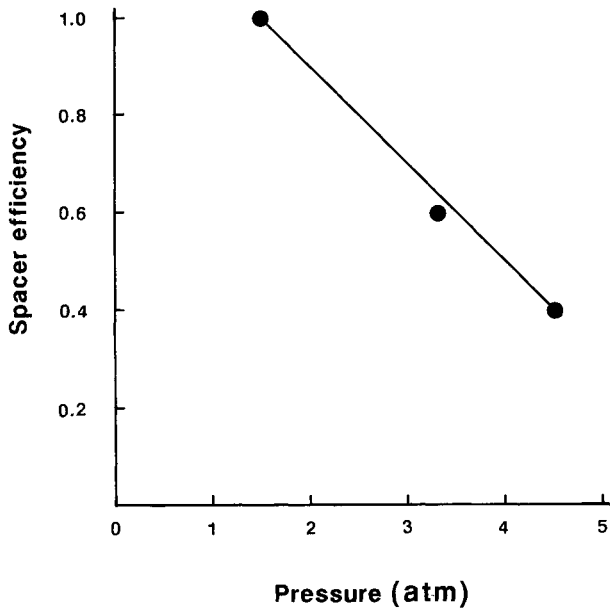
Fig. 6. Spacer efficiency vs SF 6 pressure from Ref. 9.
