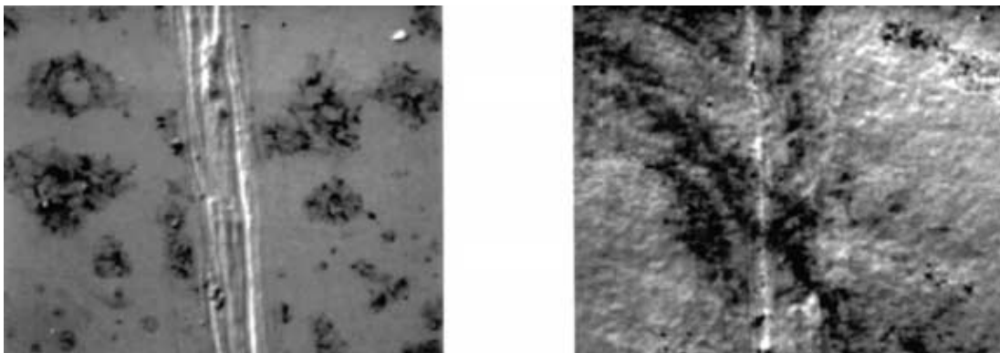
Figures 7a and 7b. Scanning electron images, showing Tribometer-caused wear tracks in Pt-Ti co-sputtered layer without beam treatment (left, magnified 300 times), and a sample area of treated layer that withstood 2000 wear cycles (right, magnified 200 times).
