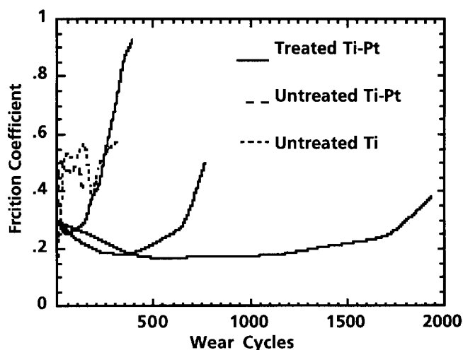
Figure 6. Friction coefficient as a function of wear cycles for untreated Ti-6Al-4V, Pt-coated but untreated Ti, and treated Pt-Ti layer (3 cases)
