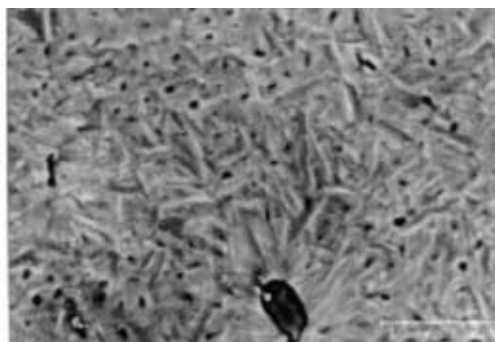
Figures 3a and 3b. Scanning electron images, magnified 2000 times, showing surface of 440C stainless steel before (left) and after (right) beam treatment.
