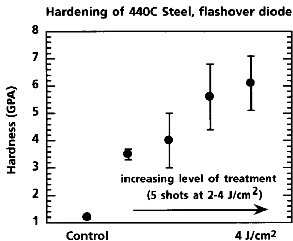
Figure 4. Surface hardening, as measured by nanoindentation, for 440C Stainless Steel as a function of beam fluence. Samples treated by flashover diode.
