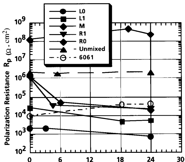
Figure 5. Polarization resistance R_p measured as a function of time for a Hf-coated Al6061 sample for 5 different fluences.
