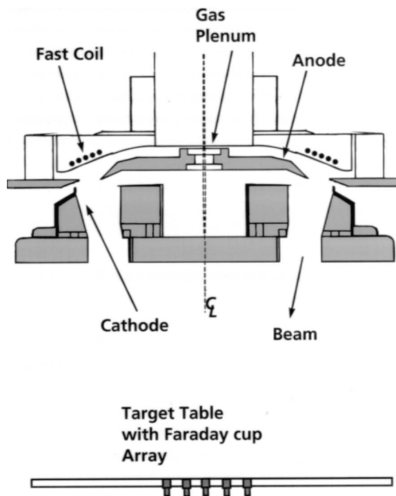
Figure 2. Diode geometry including MAP ion source and treatment area
