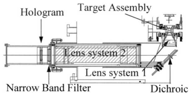
Figure 3. The in-line Fraunhofer holography experiment.
