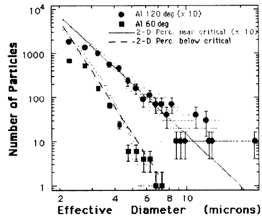
Figure 7. Ejecta particle size distributions for shocked Al compared with predictions from 2-D percolation theory.
