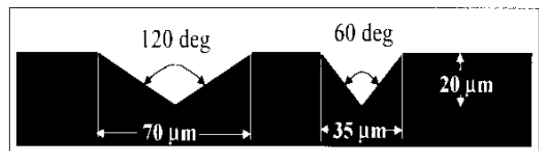
Figure 4. Cross section of the grooves that were used for the experiments
