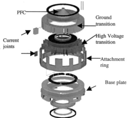
Figure 7: Transition Assembly
