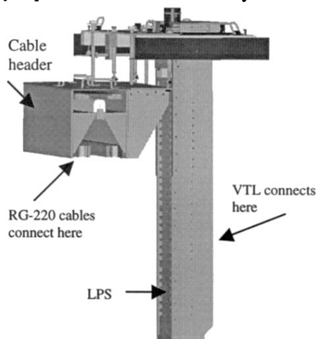
Figure 5: Cable header and LPS
