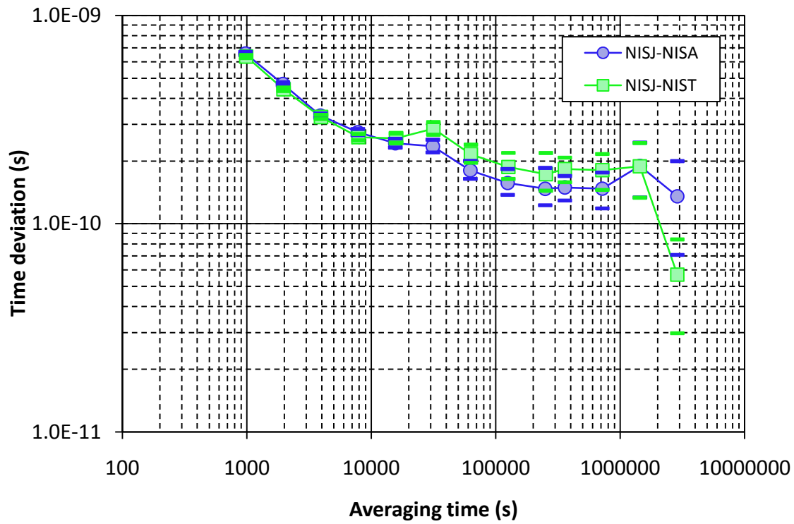
Figure 5. Time deviations of NISJ - NIST and NISJ - NISA common-clock, common-view differences.
