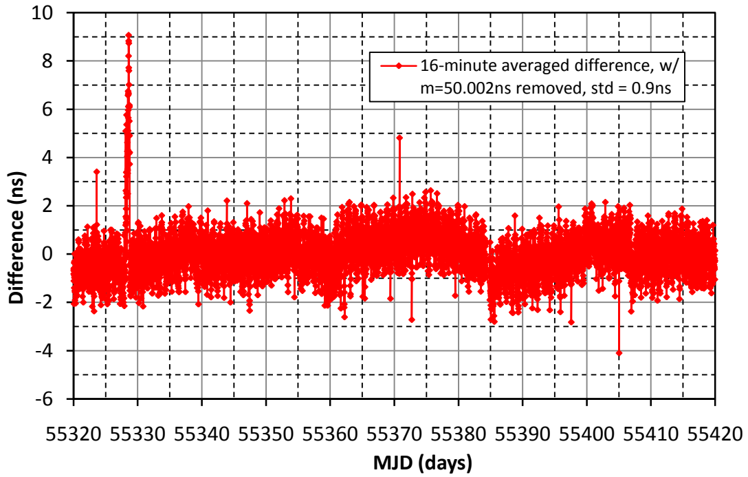
Figure 4. NISA - NIST common-clock, common-view difference.
