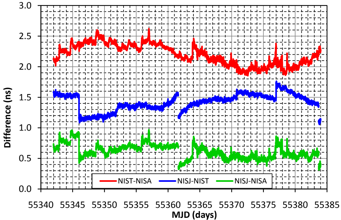
Figure 7. Common-clock, TAIPPP differences (offset for demonstration purposes).
