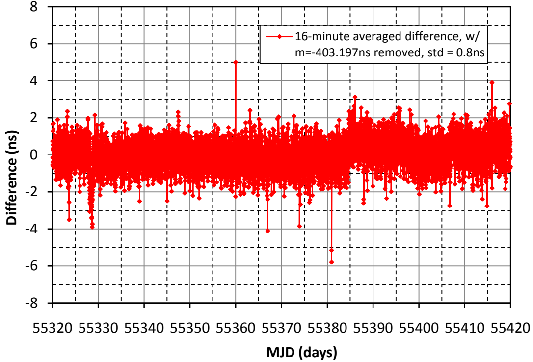
Figure 3. NISJ - NISA common-clock, common-view difference.
