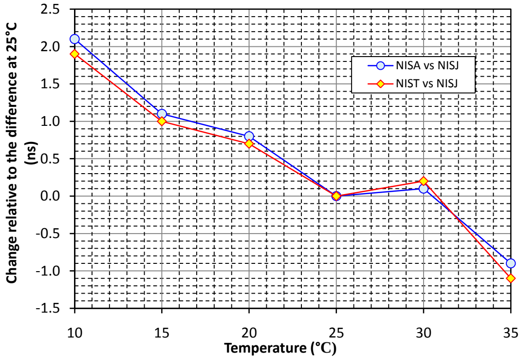
Figure 1. Temperature effect on NISJ 's code measurements relative to NIST and NISA .
