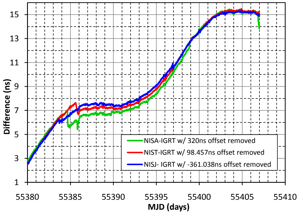
Figure 6. Carrier-phase differences from TAIPPP analysis (IGRT stands for the rapid solution of the International Global Navigation Satellite System time scale).
