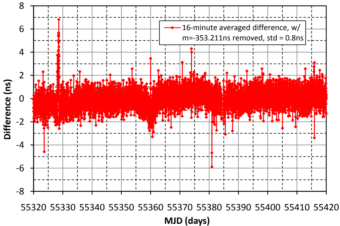
Figure 2. NISJ - NIST common-clock, common-view difference.
