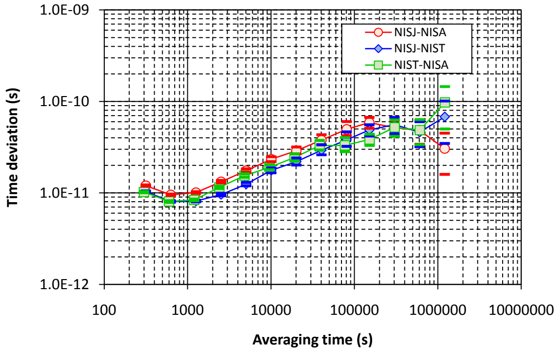
Figure 8. Time deviation of common-clock, TAIPPP differences.
