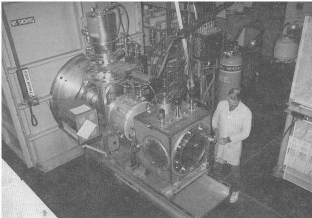
Fig. 6: Photograph of the intense ion beam device.
