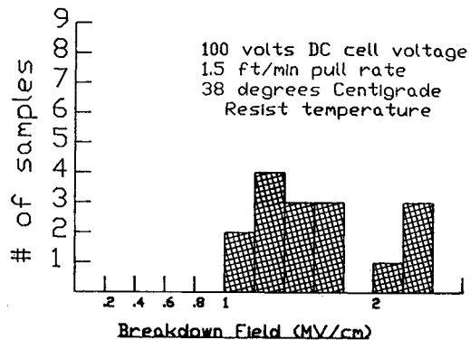
Fig. 4. DC breakdown distribution for capacitors wound from Metglas with a nominal 9 \mu\text{m} thick coating applied with the conventional EP coating technique.
