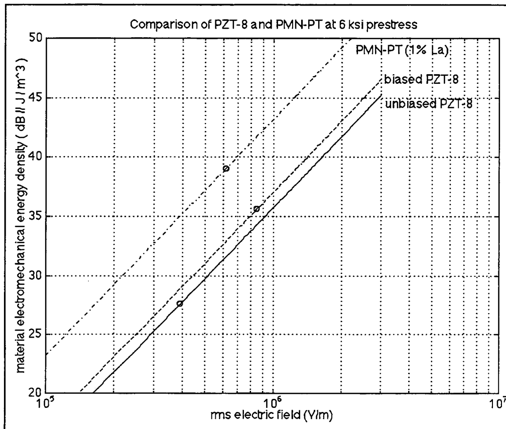
Comparison of PZT-8 and PMN-PT at 6-ksi Pre-Stress
