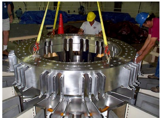
Figure 7 Transition ground conductor installation
