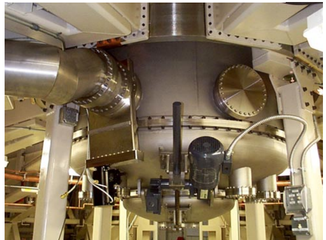
Figure 10 Atlas lower vacuum vessel
