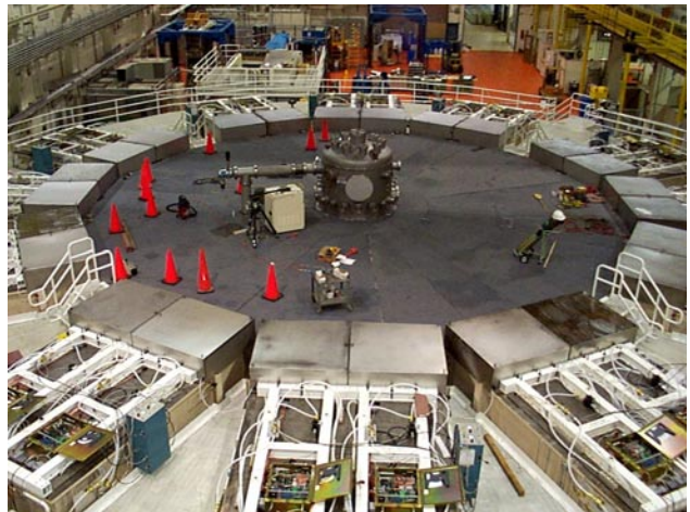
Figure 1 Atlas personnel platform and target chamber
