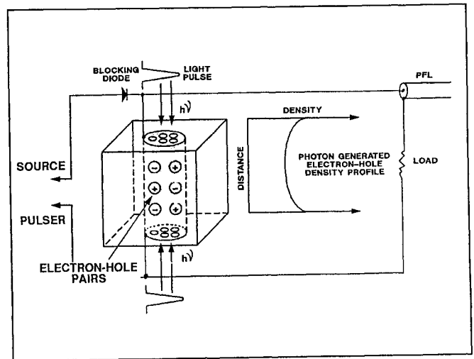
Figure 3. Conceptual Diagram of Optically Activated GaAs Switch with Opposite Gridded Electrodes. The Dual Grid Results in More Uniform Carrier Densities for Thicker Devices.
