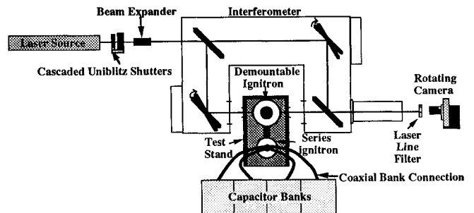
Fig. 2 Mach-Zehnder Interferometry System
