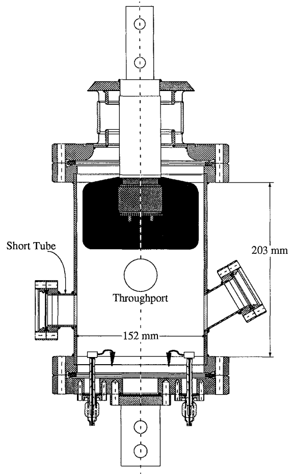
Fig. 1 Demountable Ignitron (DIG)
