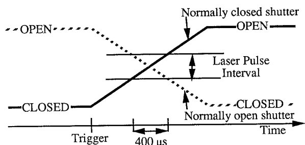
Fig. 3 Shutter Timing Diagram
