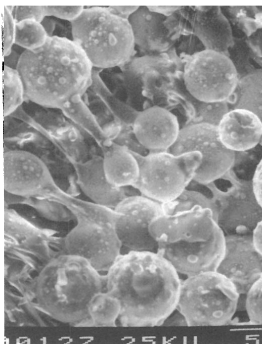
Figure 3. Scanning Electron Micrograph of copper/glass switch showing necks formed between glass spheres due to rarefaction wave. Marker indicates 50 \mu\text{m} .
