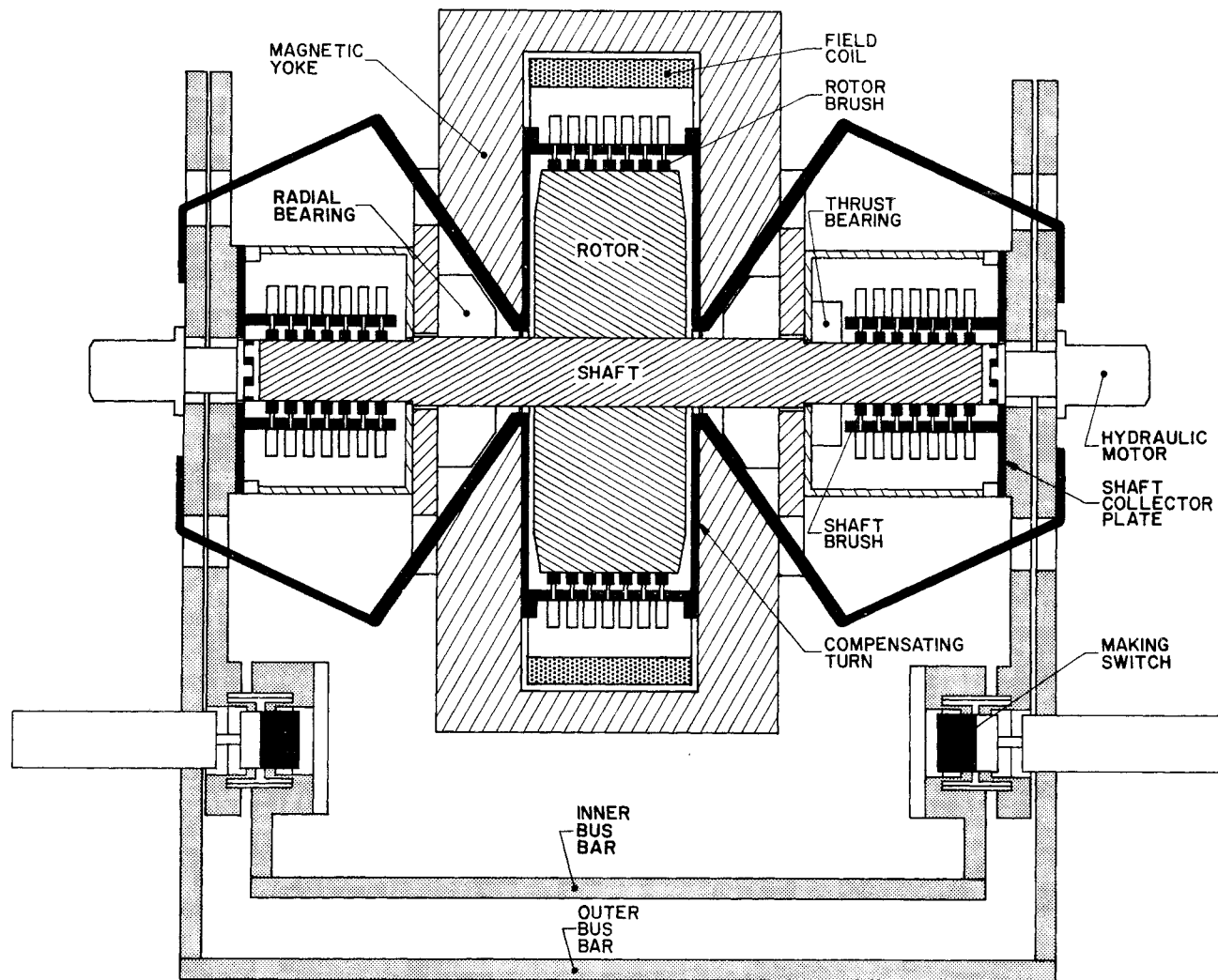
Fig. 1. 10-MJ HPG Configuration
