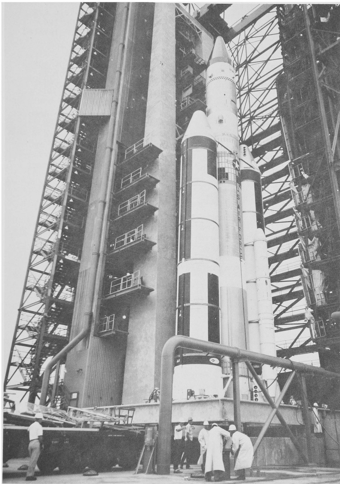
Titan III-C stands as a complete vehicle under service at Pad 41.
