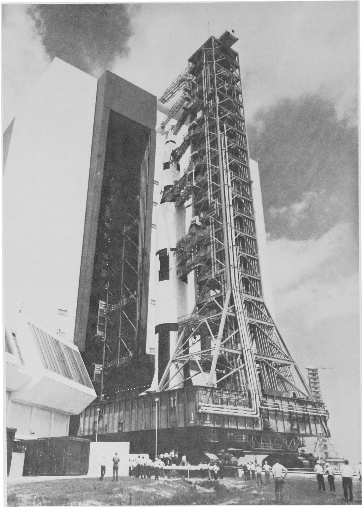
First Apollo-Saturn V spacecraft and rocket erected in the Vehicle Assembly Building leave on their maiden, 3½-mile trip to the launch pad.
