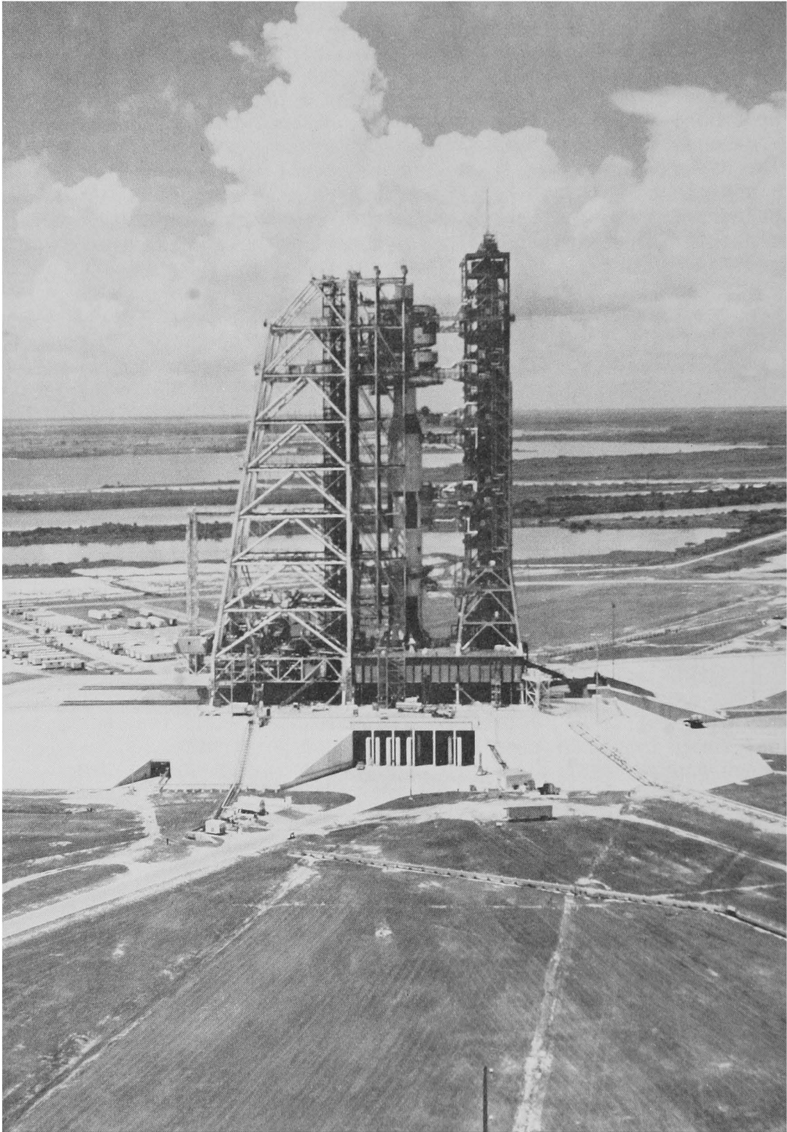
First flight version of Apollo-Saturn V launch vehicle is checked out at Pad A of NASA's Kennedy Space Center prior to launch on November 9, 1967. Tower to right of vehicle is Mobile Launcher; structure to left is Mobile Service Structure.
