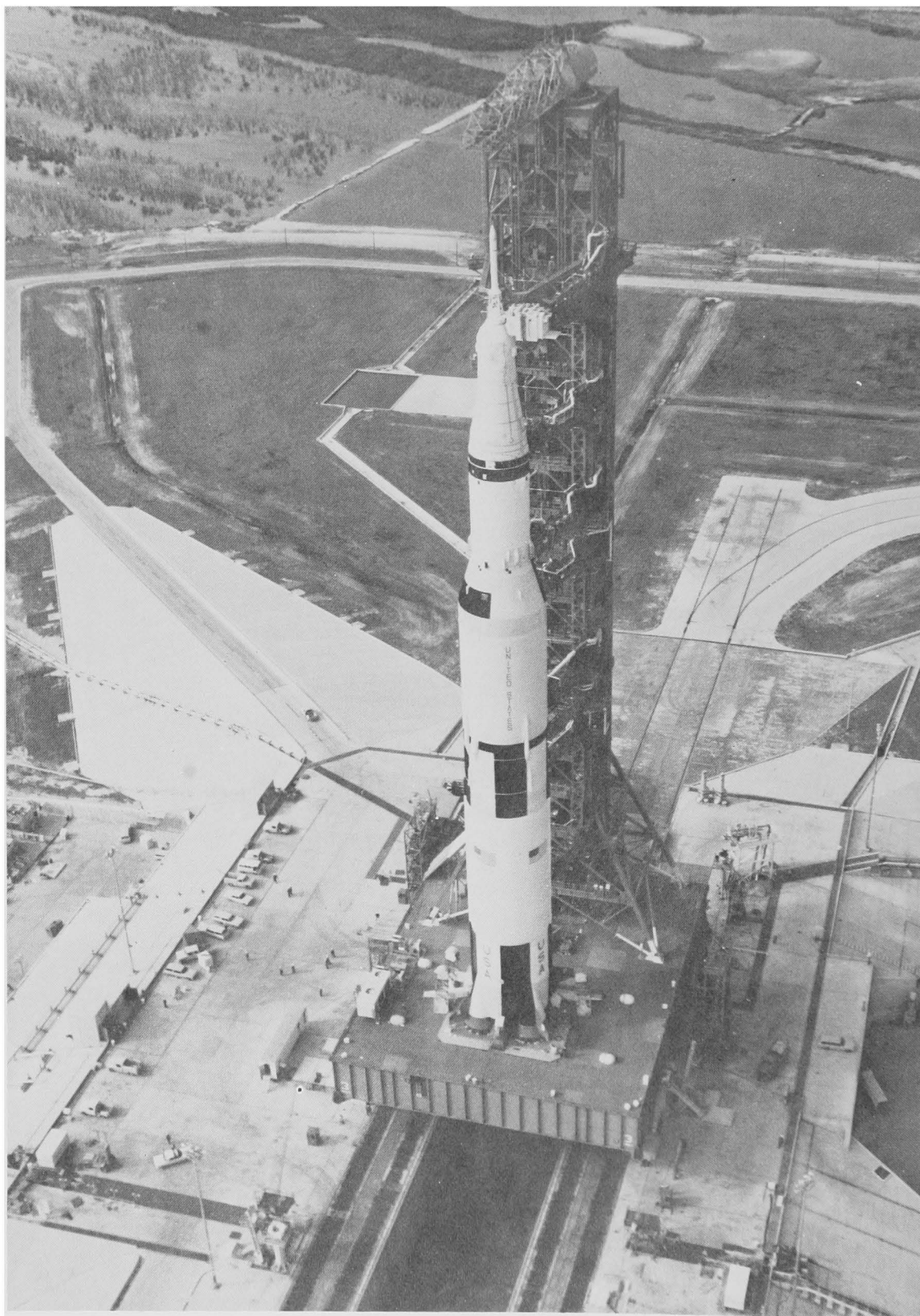
This view of Pad 39-B shows Apollo 10 in launch configuration. Note the antlike size of men below and to the left of vehicle.
