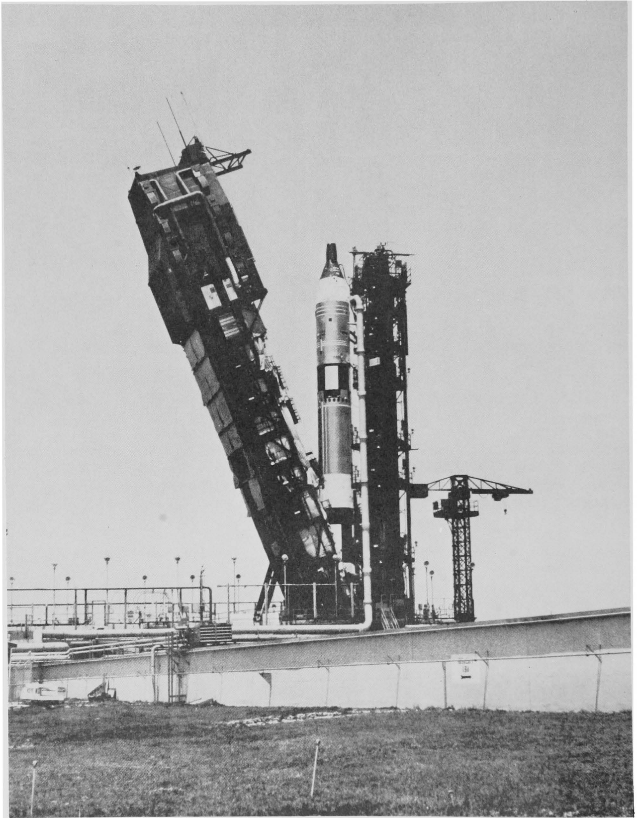
One of first major projects for new Canaveral District was completion of conversion of Launch Complex 19 from Titan I to Titan II facility for NASA's Gemini Program. Here Titan II Gemini vehicle is readied for space mission at newly modified facility.
