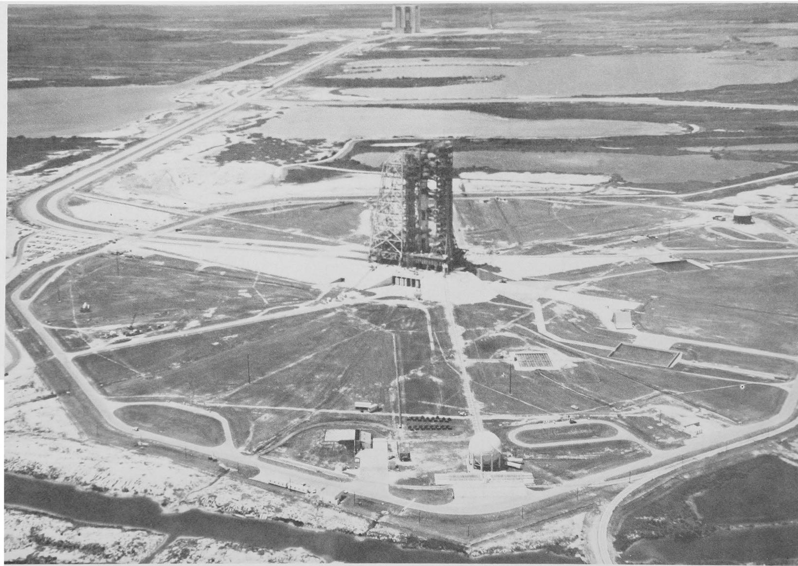
The westward view, Pad 39-A sits in foreground, with VAB in distant background and Crawlerway between. First flight model of Apollo-Saturn V sits on Pad, flanked by Mobile Service Structure (left) and Mobile Launcher.
