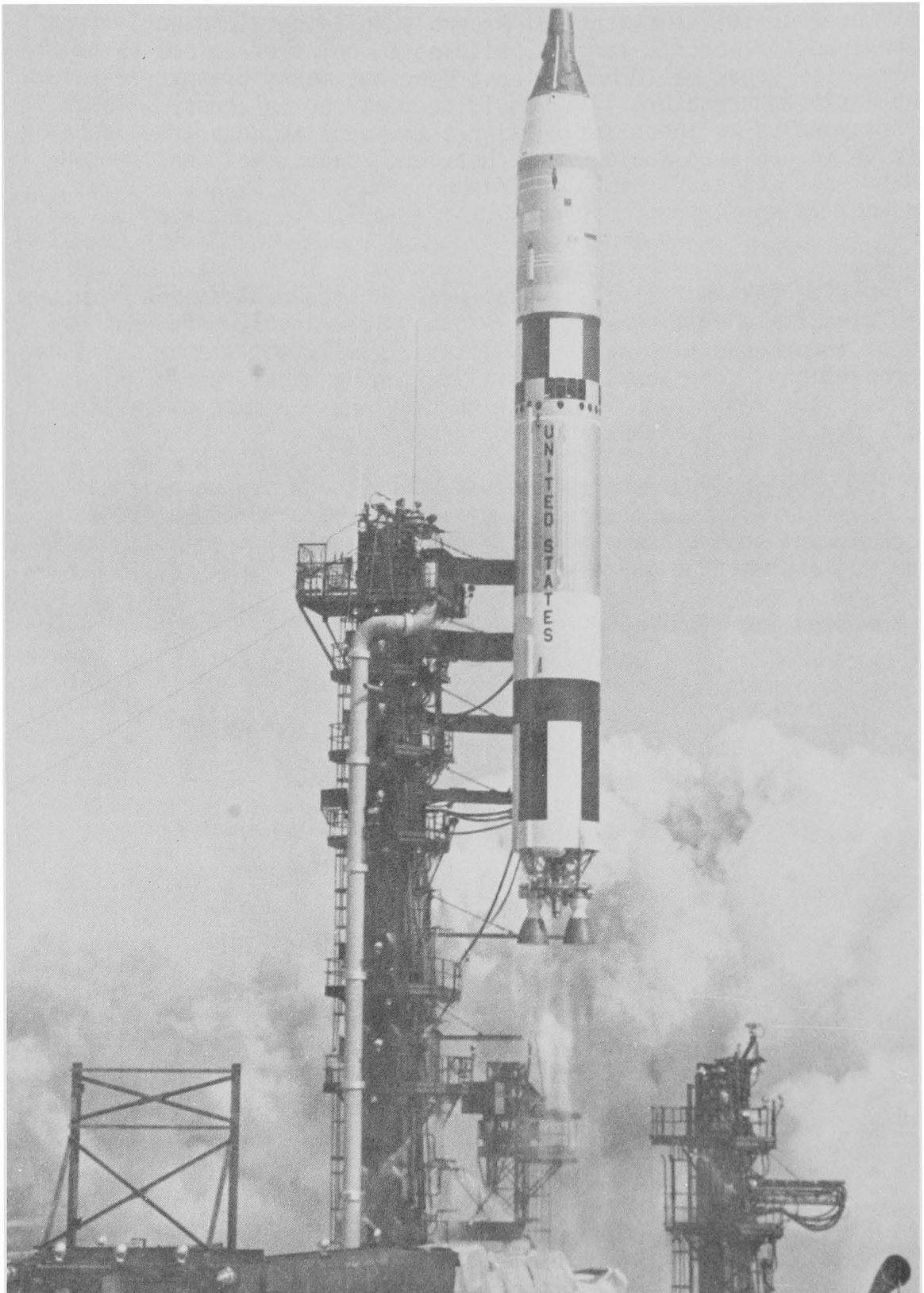
First U.S. two-man flight in Gemini program made three orbits of earth on 23 March 1965. Lift-off from Launch Complex 19.
