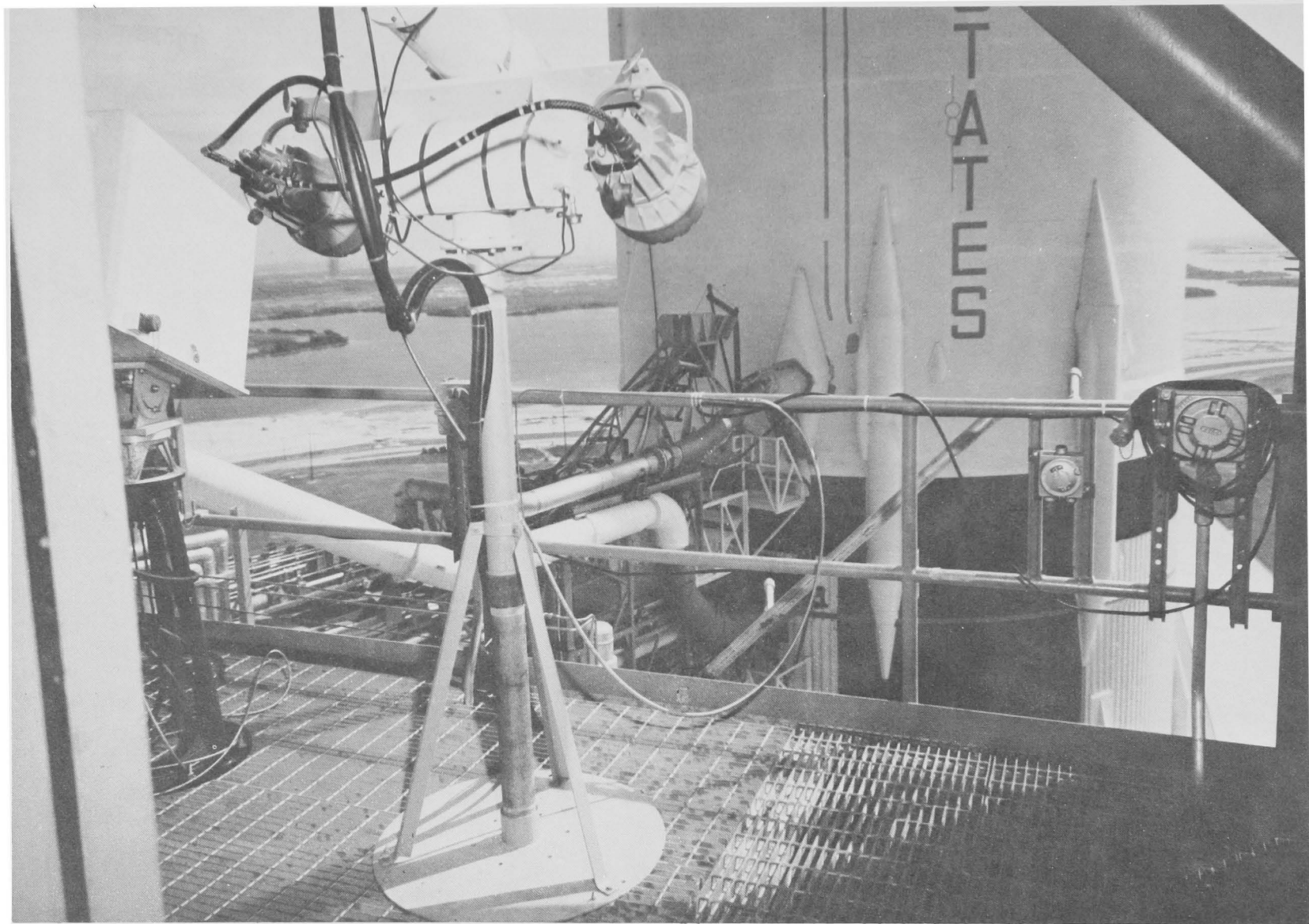
One for the Shutterbugs: This camera mount on Mobile Launcher is contrived to catch ignition and liftoff action at base of Saturn V when moonrocket leaves Complex 39. Elasticity is built into mount and all essential cabling to absorb launch-point shock moments.
