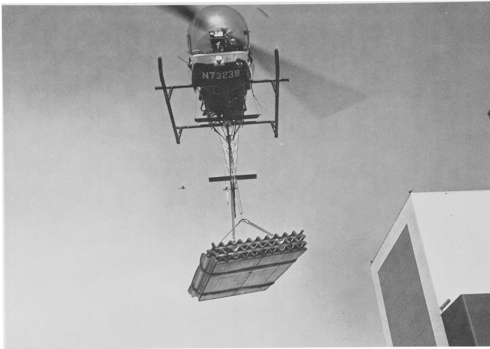
VAB construction brought on ingenious work methods. Here a helicopter lifts siding to building's upper levels. Construction of the 129 million cubic-foot VAB was completed at a cost of $117,000,000.
