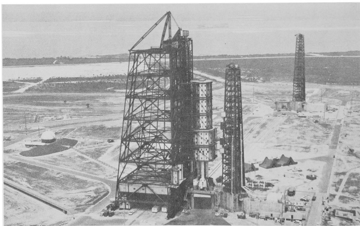
Upper view shows launch complex 37 as completed by Corps for NASA in late summer 1963. Lower photo shows Saturn test rocket erected on launch pedestal, its upper portions enclosed in the steel compartments of service tower which permit vehicle checkout in a protected environment.
