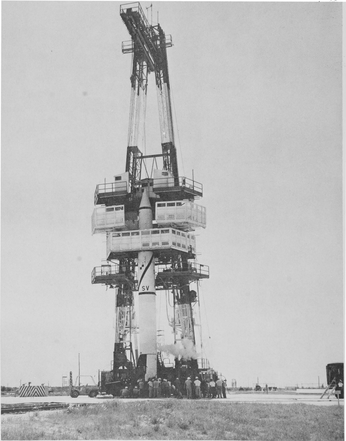
Redstone Service Tower was first (1953) of long and imposing row of missile gantries confronting the Atlantic at Cape Canaveral/Kennedy. Redstone booster itself put first American in space (CMDR Alan Shepard 1961).
