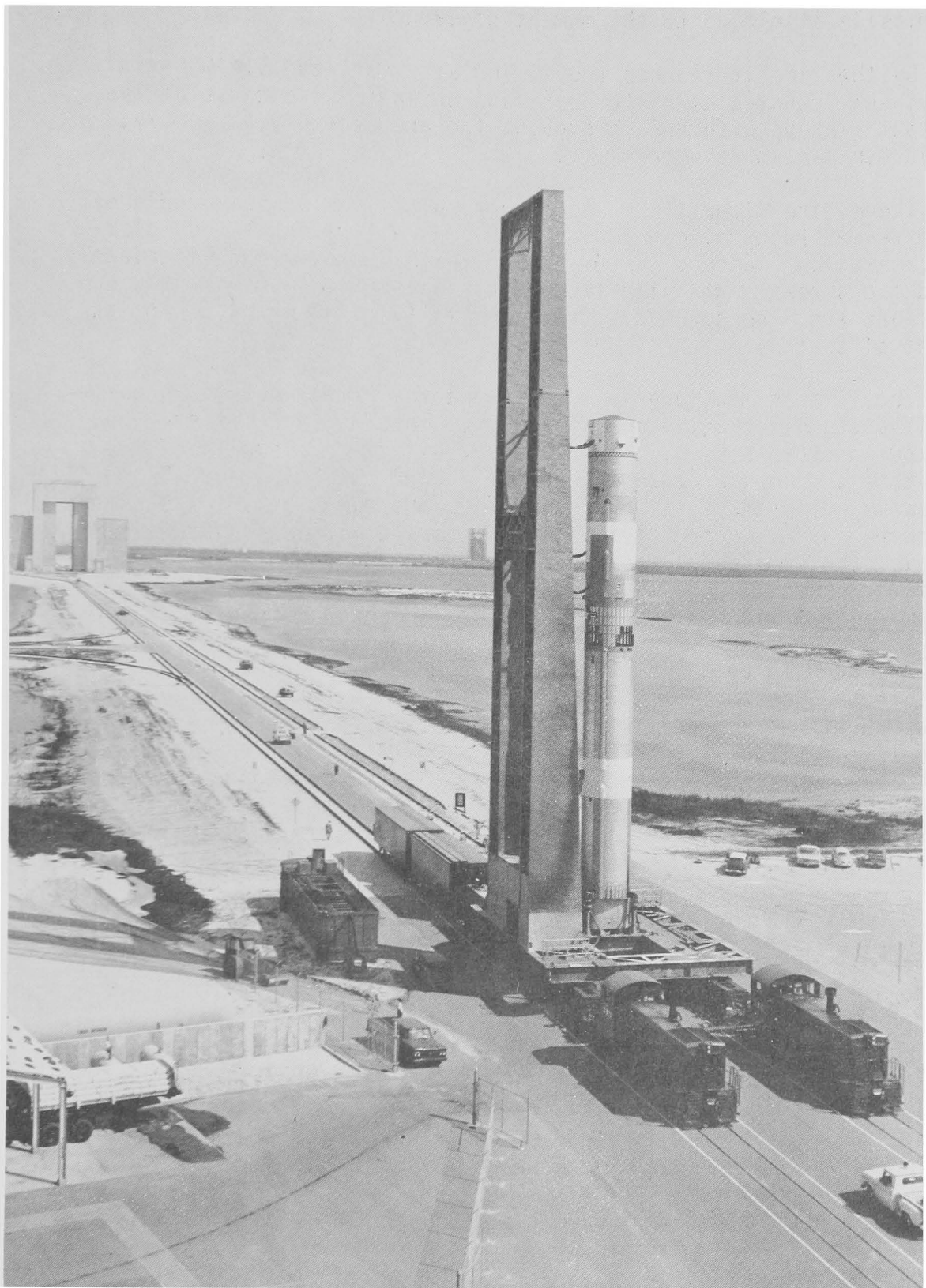
Here Titan III core moves with pusher locomotives from VIB to SMAB for strap-on boosters and later transport to Pad 41. Corps delivered island-chain complex, railroads, launch pads to Air Force as operational on April 1965.
