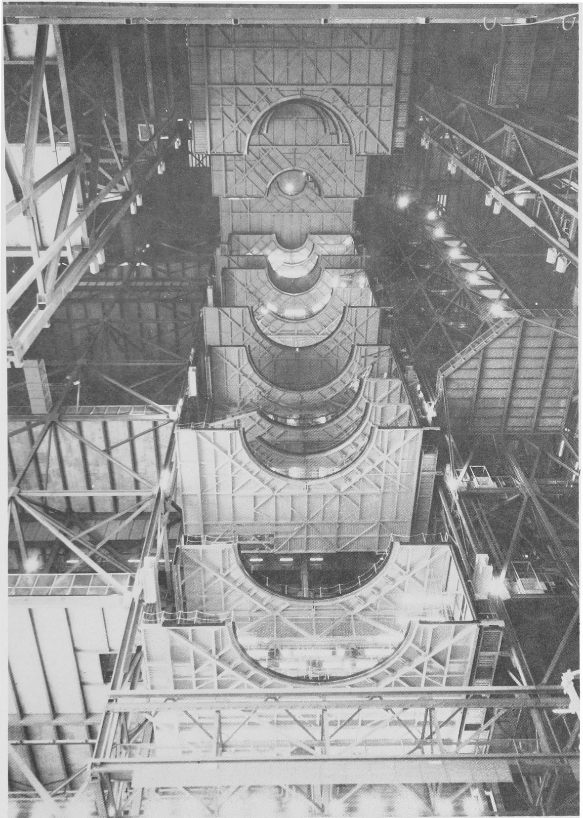
Looking aloft inside High Bay of VAB affords breathtaking view of extensible work platforms.
