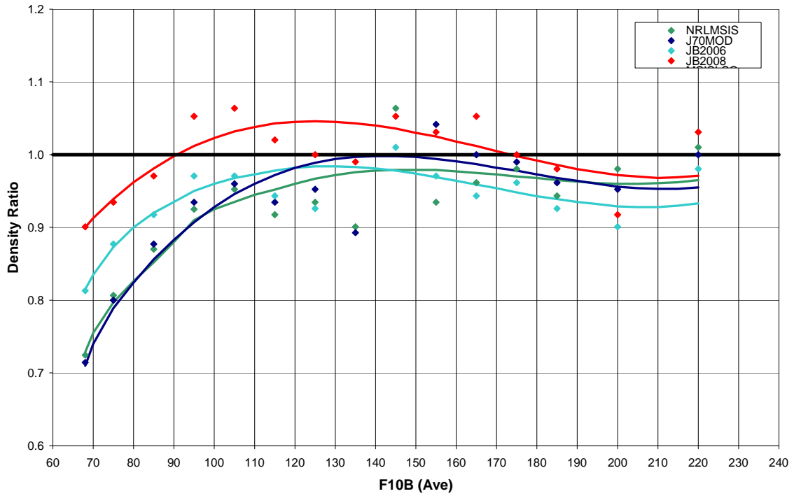
Figure 1. HASDM-to-Model density ratios at 400km altitude as a function of \bar{F}_{10} (F10B).
