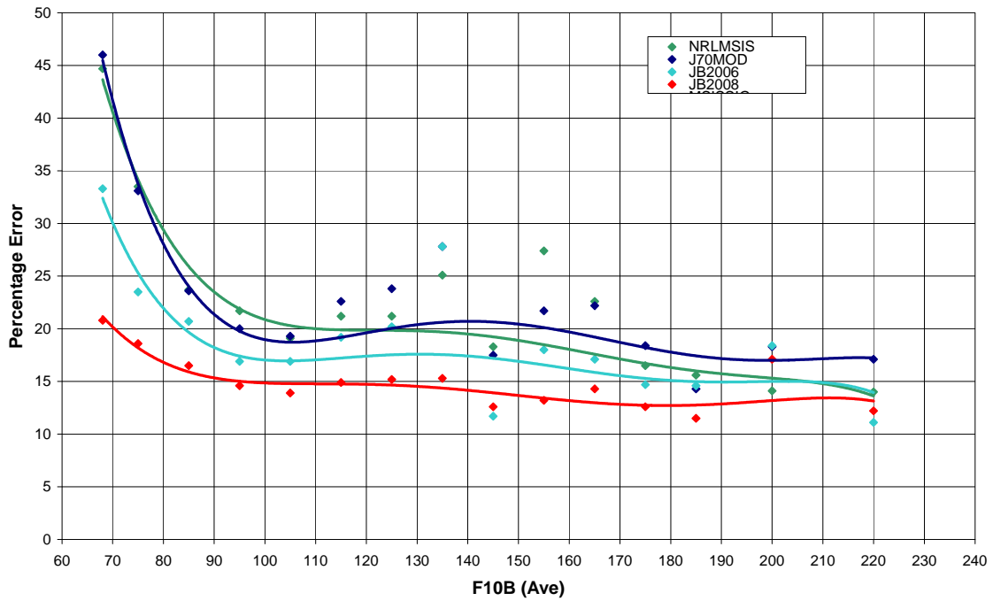
Figure 2. Density percentage errors (1 standard deviation) from model density values at 400 km altitude compared to HASDM density values.
