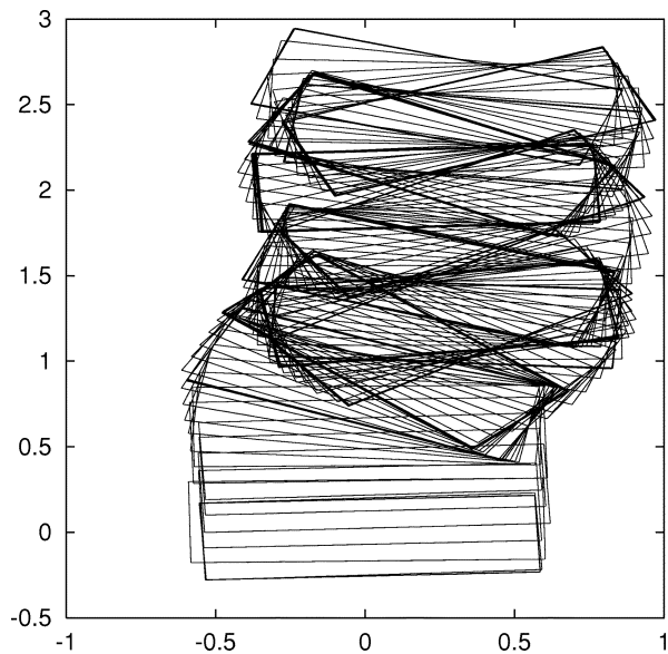
Fig. 9. Path of the box in an example trial from Experiment Set 3 (units are meters). The right pusher fails, leaving the other pusher to push either end of the box in turn.
