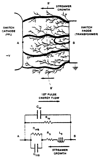
ig. 3. Positive tree growth showing heavy streamer channels that eventually form (top) and the electrical switch model of the process (bottom).
