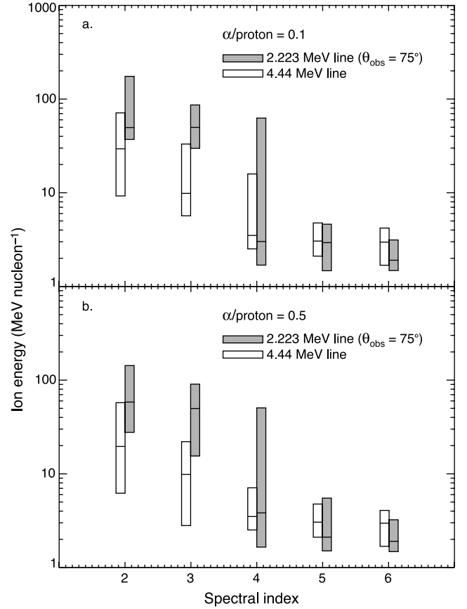
FIG. 21.—Effective accelerated ion energies for production of the 4.438 MeV ^{12}\text{C} line (white boxes) and 2.223 MeV neutron capture line (gray boxes) as a function of spectral index. The effective energy ranges are the 50% yield range as defined in the text. Panel (a) shows accelerated \alpha/\text{proton} = 0.1 and (b) shows \alpha/\text{proton} = 0.5 . For the neutron capture line, \lambda = 300 , \delta = 0.2 , L = 11,500 km, and \theta_{\text{obs}} = 75^\circ .
