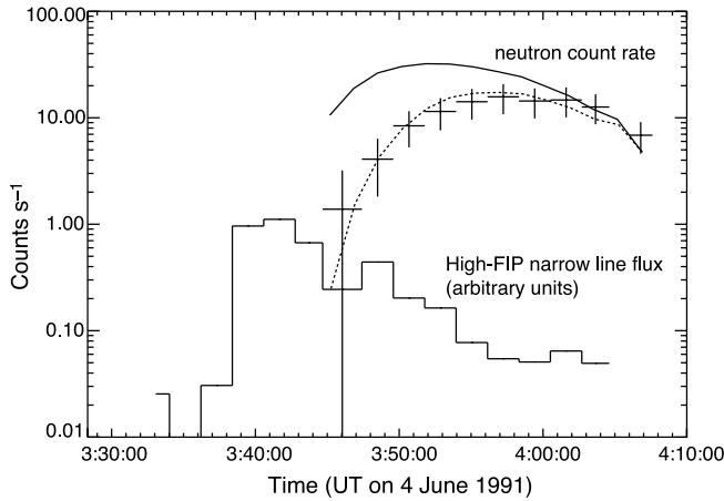
FIG. 31.— Comparison of the >23 MeV neutron count rate time history measured with OSSE from the June 4 flare with count rate time histories calculated with the parameters indicated in the text. The solid curve is for an unbroken power-law accelerated-particle spectrum and the dotted curve is for a spectrum cutoff at E_c = 125 MeV nucleon ^{-1} . Also shown is the time history of the high-FIP narrow deexcitation line flux (histogram) assumed to represent the accelerated ion release time history.
