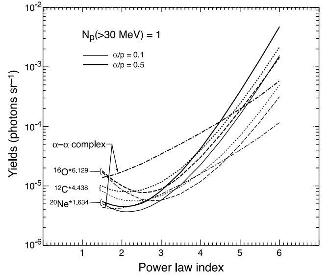
FIG. 6.—Calculated yields of the 1.634 MeV ( ^{20}\text{Ne} ), 4.438 MeV ( ^{12}\text{C} ), 6.129 MeV ( ^{16}\text{O} ), and \sim 0.45 MeV \alpha - \alpha complex as functions of the accelerated-ion power-law spectral index for accelerated \alpha /proton = 0.5 (thick lines) and 0.1 (thin lines). Deexcitation line yields do not depend on loop parameters. All yields are normalized to 1 accelerated proton of energy greater than 30 MeV.
