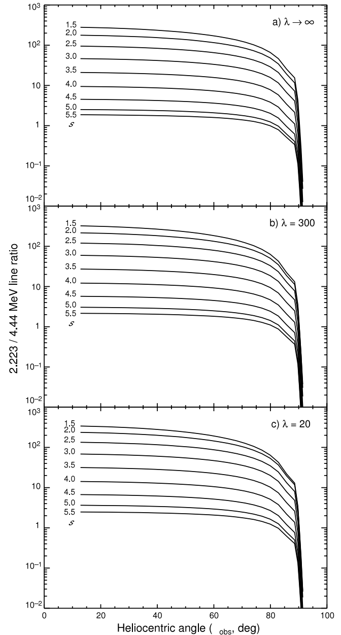
FIG. 16.—The 2.223 MeV (neutron capture)/4.438 MeV ( ^{12}\text{C} ) line fluence ratio as a function of the flare heliocentric angle ( \theta_{\text{obs}} ), parameterized by spectral index ( s ): (a) no PAS, (b) nearly saturated PAS, and (c) saturated PAS.
