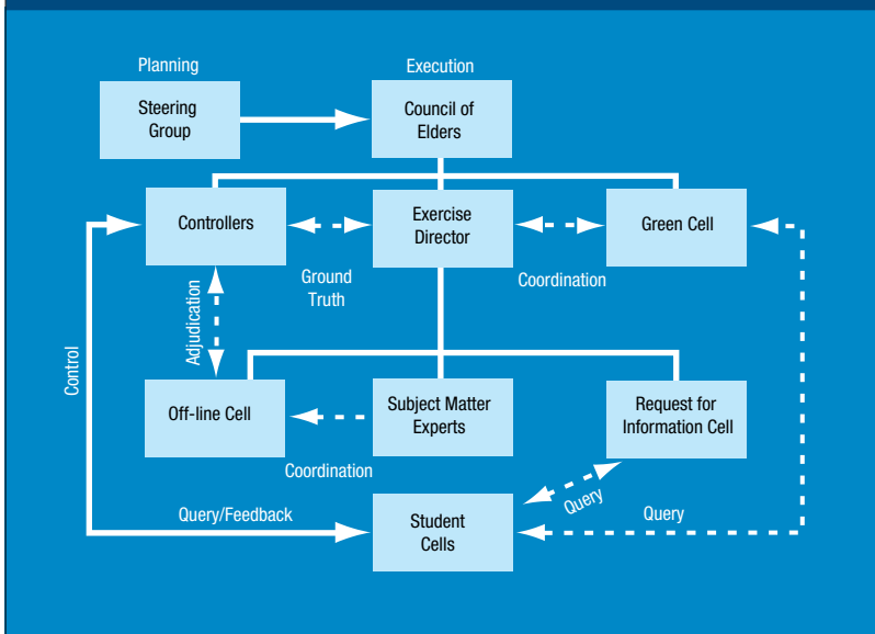
Figure 2: JLASS Structure
