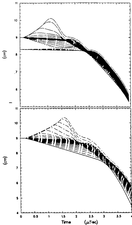
Fig. 2. Calculated positions as functions of time for the Lagrangian zones with (top) and without (bottom) a separate, polyurethane, barrier foil. Total mass is the same in each calculation, absolute positions have no significance.
