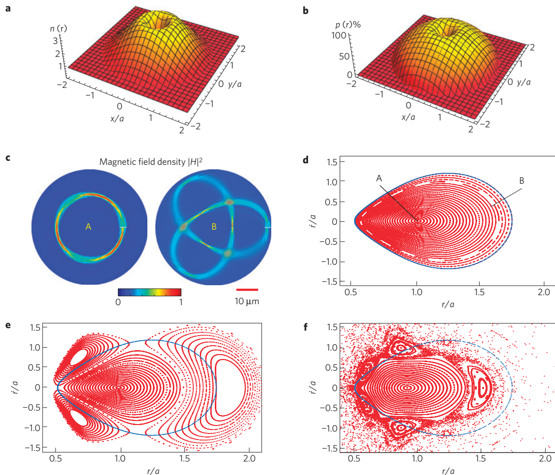
Figure 3 | CIPTs based on air-GaNAsP composite media. a, b Refractive index profile ( a ) and volume fraction ( b ) of the GaInAsP. c , FDFD simulations of bound and stable light propagation in the form of A, a circular orbit with period 2\pi and B, a 'Rosetta' type of orbit with period 4\pi . In the calculations, a linear source with width w = 6\lambda and wavelength \lambda = 1.55 \mu\text{m} is used. d-f , Poincaré maps ( P_T ) corresponding to all possible photon trajectories for linear ( d ) and nonlinear ( e, f ) refractive indices. In the linear case, the photon motion follows stable periodic and quasi-periodic trajectories for all initial conditions. With the introduction of nonlinearity, the stability of the system is disturbed with some trajectories passing through the cavity boundaries and leaving the system. f , For above-critical values of the nonlinear index \Delta n_{\text{NL}}/n_{\text{max}} = 0.2 , chaotic behaviour is observed similarly to the three-body problem in celestial mechanics. In generating the Poincaré maps, the scale-invariant parameters r/a and \dot{r}/a are sampled at times t_m = 2\pi m/\omega_{\text{NL}} that are an integer number m of the nonlinear period (or T-period map), and the derivative is taken with respect to the azimuth angle \varphi .
