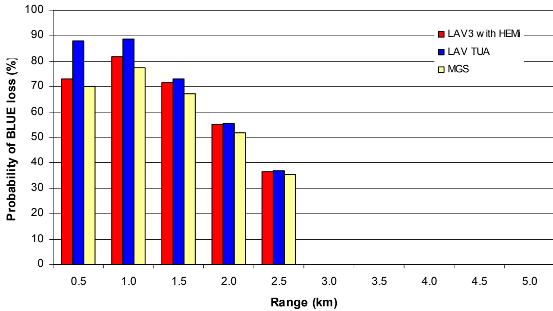
Figure 17. T-80U with 125 mm APFSDS, offensive scenario: probability of BLUE loss
