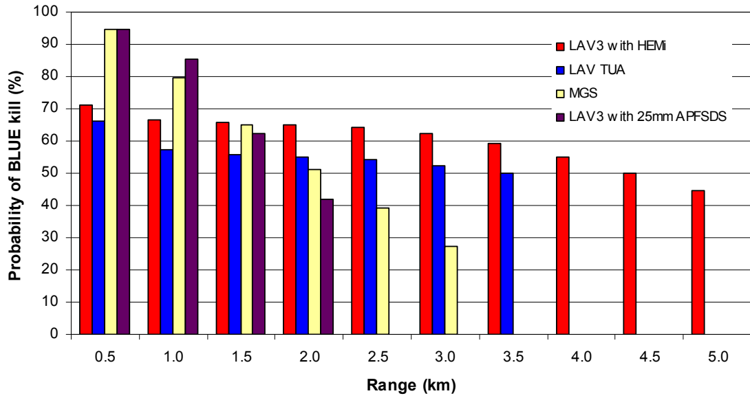
Figure 10. BMP2 with AT-5, defensive scenario: probability of BLUE kill
