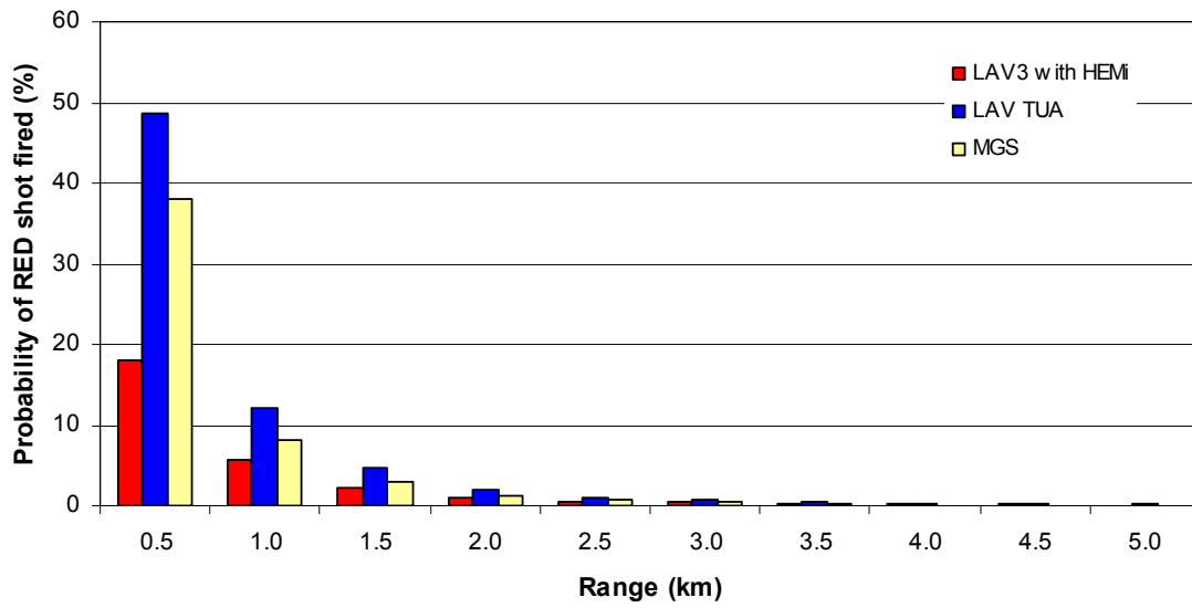
Figure C21. T-80U with AT-11, defensive scenario: probability of RED shot fired
