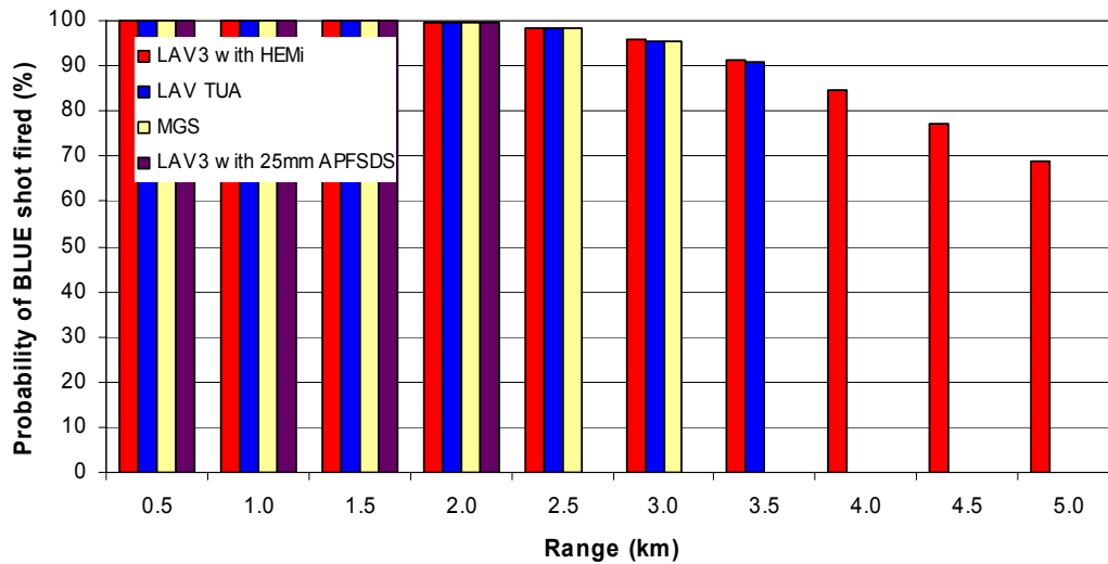
Figure C2. BMP2 with 30 mm APDS-T, defensive scenario: probability of BLUE shot fired
